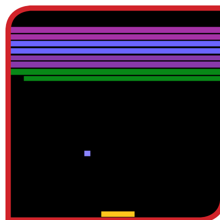
SUPER BREAKOUT
