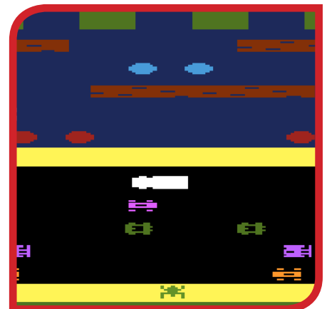
FROGGER
