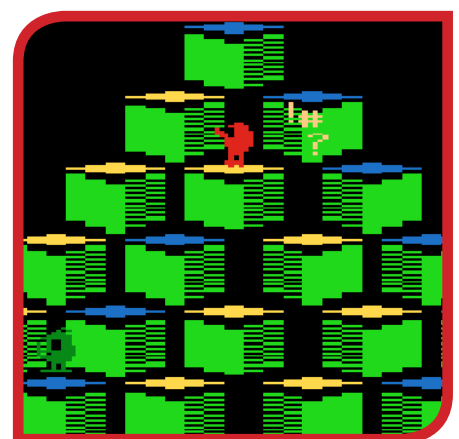
Q*BERT
