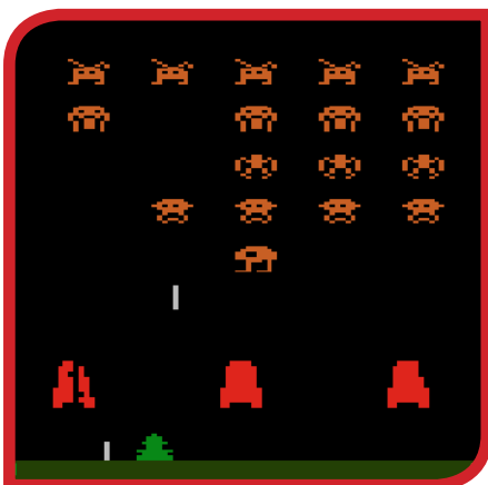
SPACE INVADERS
