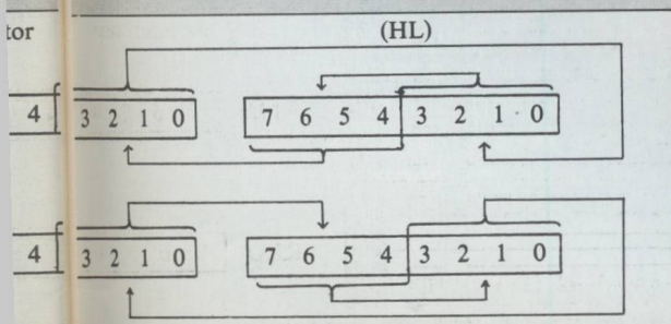
Figure II: Nibble shifting instructions
