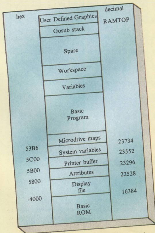
Figure I: The memory map
