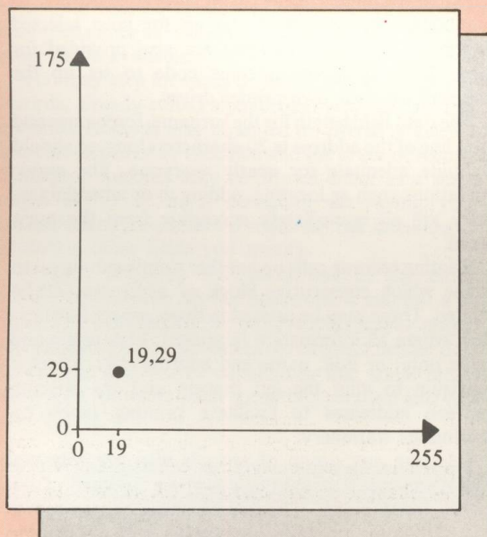
Figure 1: Pixel coordinates
