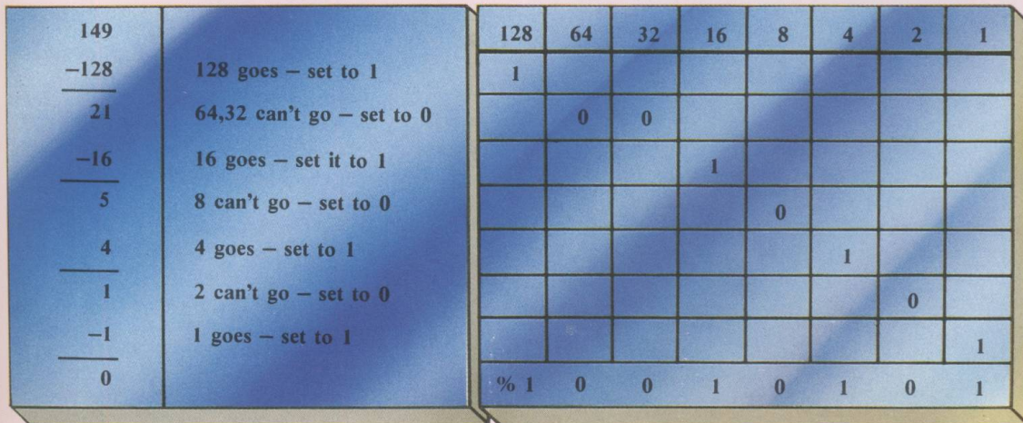
Figure 1: Converting from denary to binary
