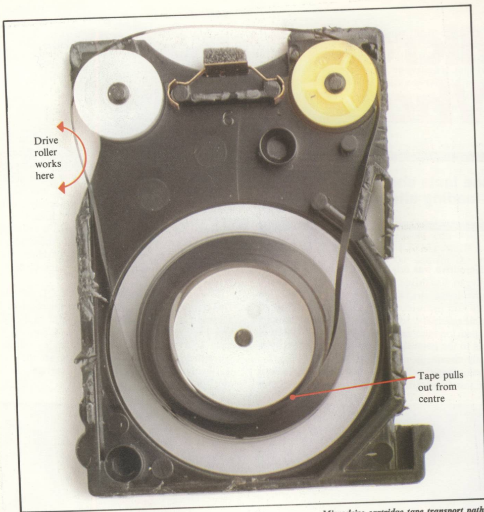
Microdrive cartridge tape transport path
