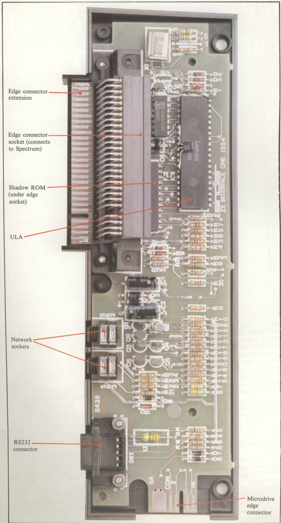
Interface 1 circuit board
