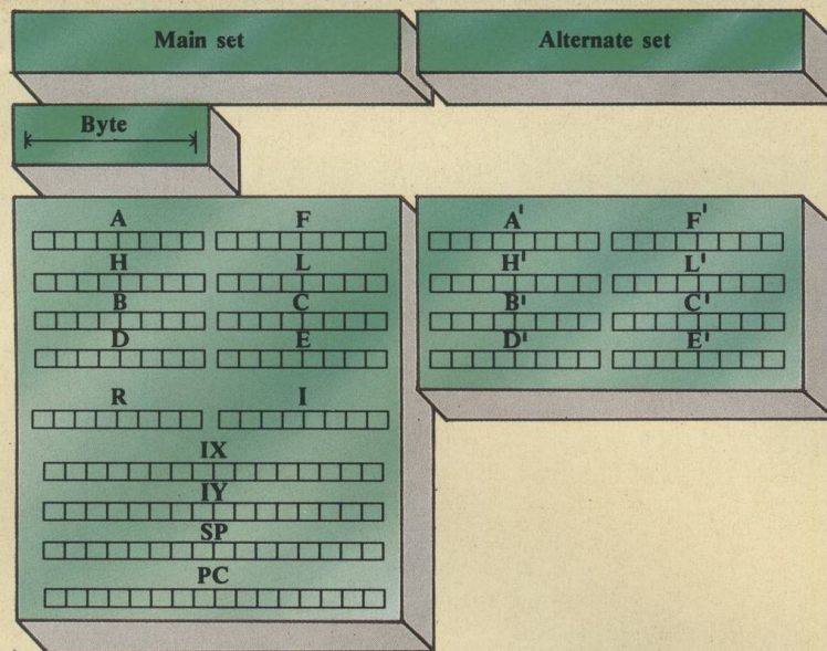
Figure 1: Z80 register set
