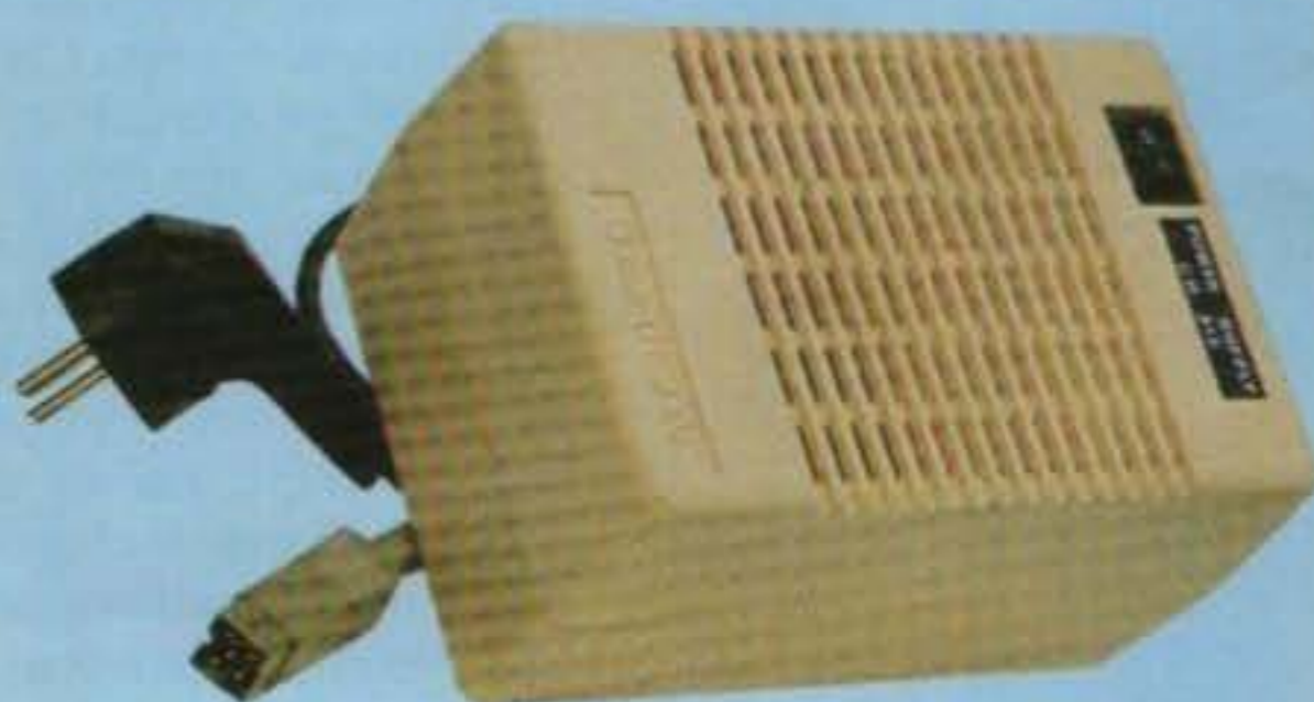
Power supply for Commodore Amiga 500. ART. CH 315. Input 220 V./50 Hz. - Output 5,1V./4A. + 12V./1,2A. - 12V./0,5A.
