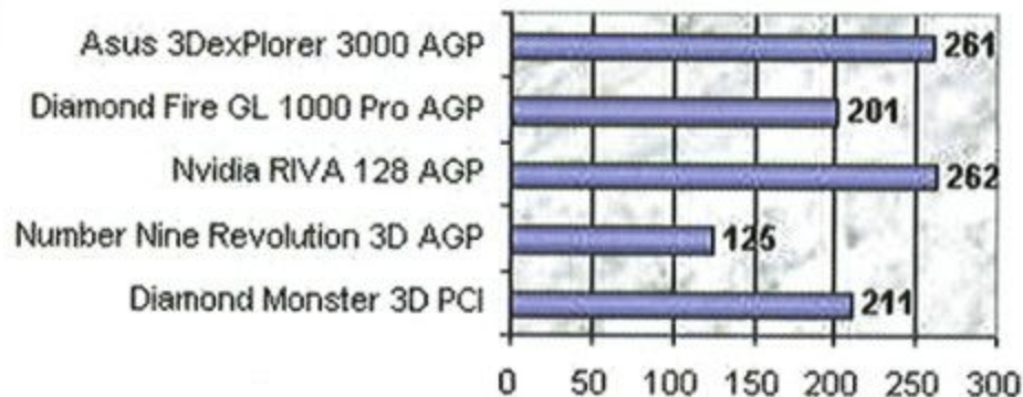
3D Winbench
