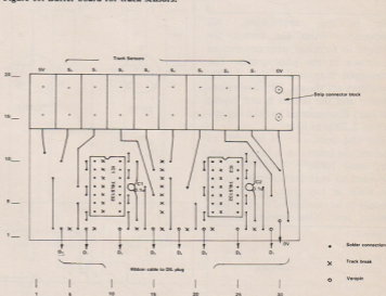
Figure 10. Buffer board for track sensors.
