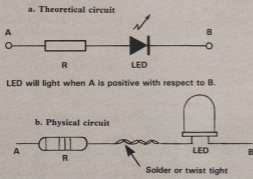
Figure 1. Test circuit.
