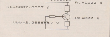
Equivalent circuit for figure 3.
