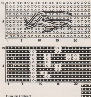
Figure 3b: Veroboard
