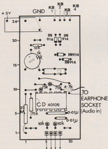
Figure 2: Music interface—top of PCB
