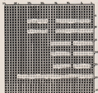
Figure 4: Veroboard.
