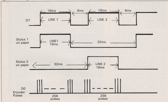
Figure 2: D0/D7 timing
