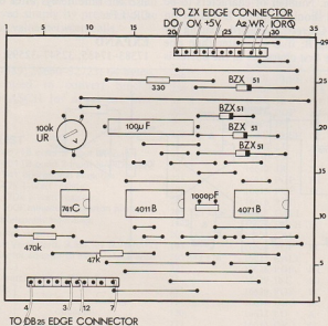
Figure 2: Top of PCB.
