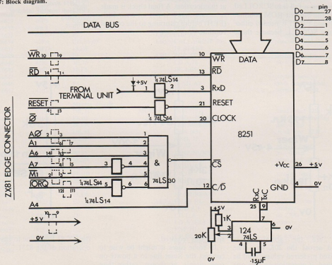
Figure 7: Block diagram.
