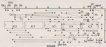
Figure 5: Output port—Veroboard
