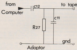
Figure 11: Music Interface
