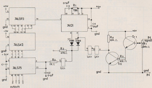
Figure 1: Output port—circuit diagram
