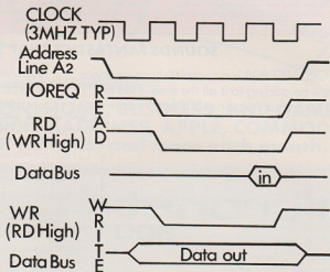
Figure 1: Printer I/O
