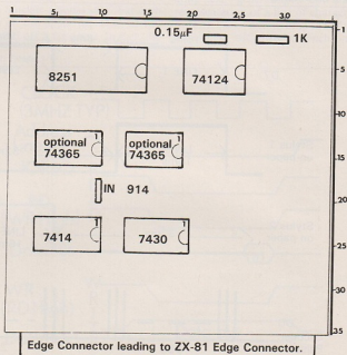
Figure 3: Top of PCB.
