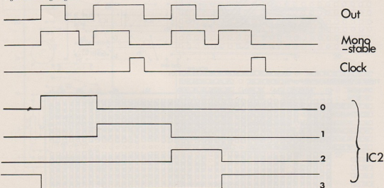
Figure 10: Timing Diagrams
