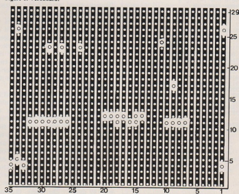
Figure 1: Veroboard.
