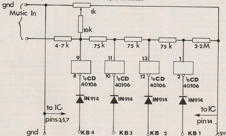
Figure 11: Music Interface
