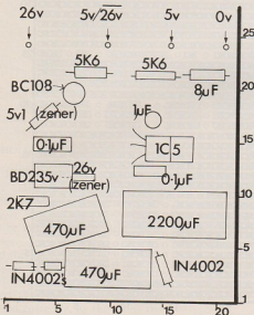
EPROM BLOWER: PCB layout for large board
