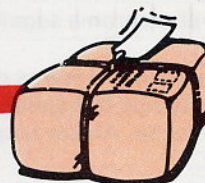
BETA-BASIC
