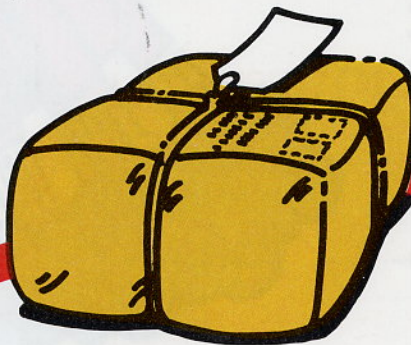
BASIC
