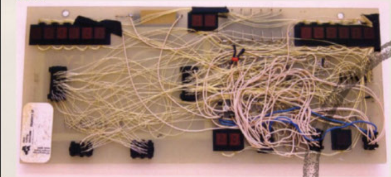
» [Fig. 7] The processor card for the Flicker pinball machine that David and Jeff retrofitted to use a microprocessor.
