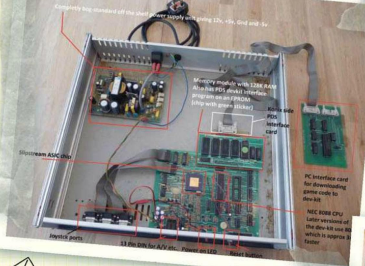
This is a photo of the only known surviving Konix dev-kit. Campbell has labelled the interesting parts of the board.
