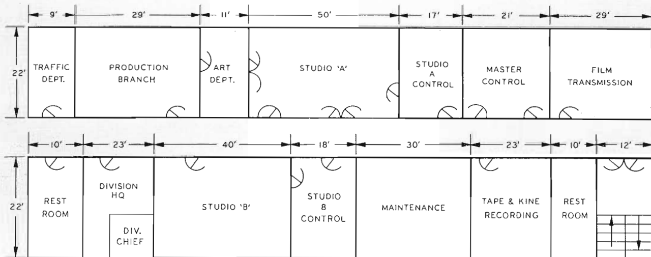
FIG. 26. Floor plan, WFM-TV television facilities.
