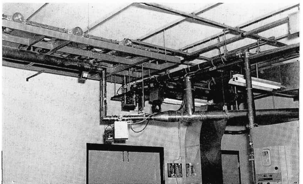
FIG. 5. This view of the RCA transmitter shows the side band filter, ceiling mounted visual low-pass filter, co-ax patch panel and gassing system for exterior coax run. All this was installed at the new WOW-TV transmitter building.
