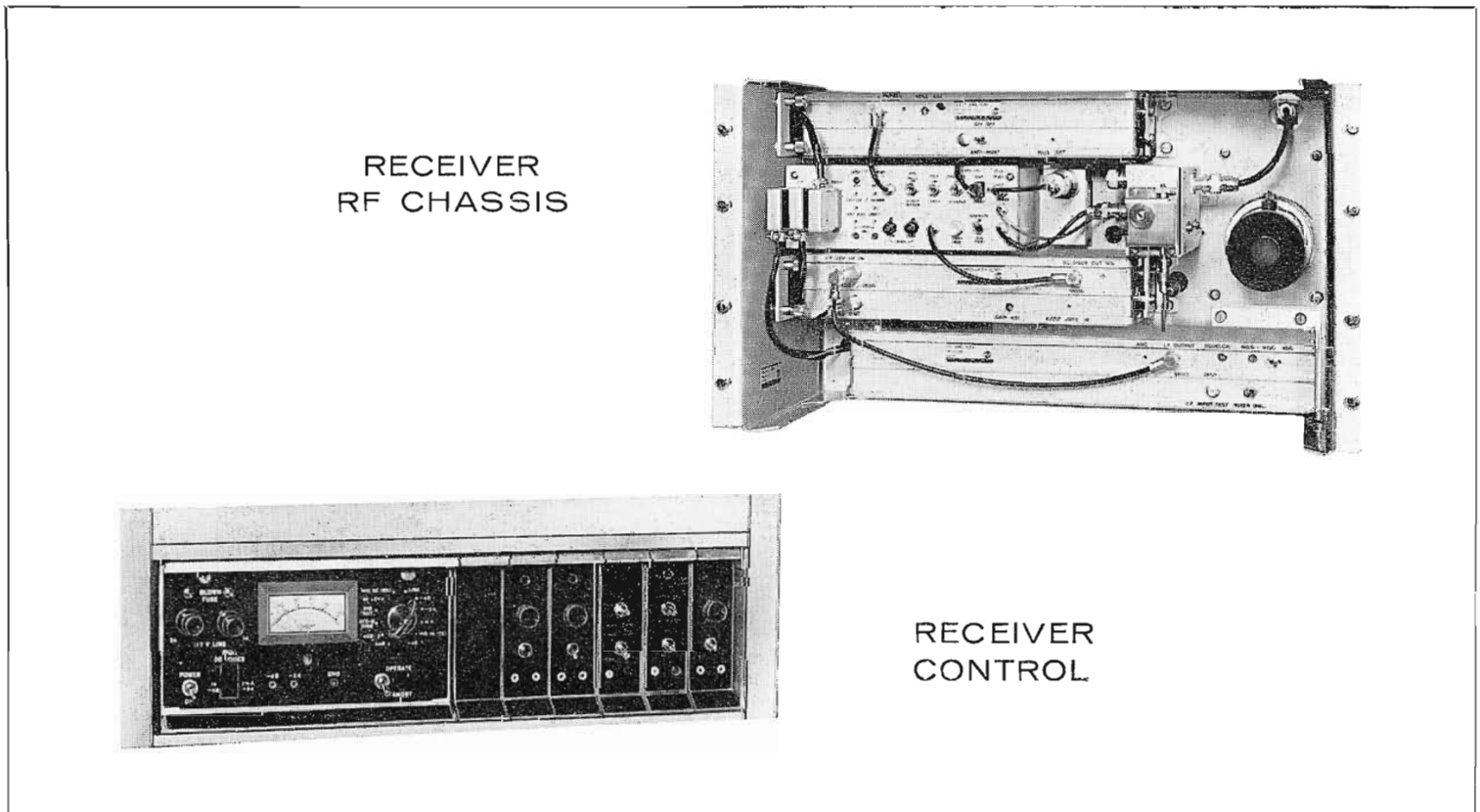
FIG. 9. TVM-6A receiver RF chassis and receiver control units. Control unit provides space for seven plug-in modules including the LVPS and the klystron control module, which are required, plus five optional slots for accessory modules. Shown are three sound modules (demodulators), an output amplifier, and a video patch module.
