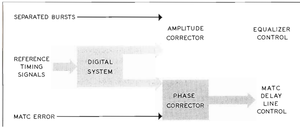
FIG. 8. Block diagram showing principal functions of CAVEC.
