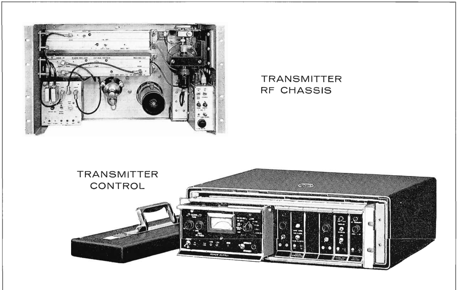
FIG. 4. Transmitter RF chassis and transmitter control units showing placement of operating elements. Change of sub-chassis units is easily performed and operating controls and adjustments on both units are convenient.
