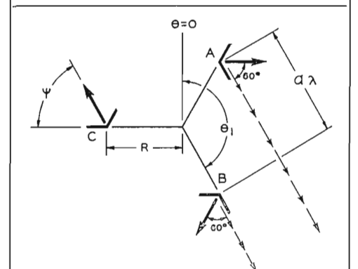
FIG. 5. Three skewed panels. a=n+\Delta , \Delta=0, 1/3 or -1/3 ; n =integer, \psi =skew angle.
