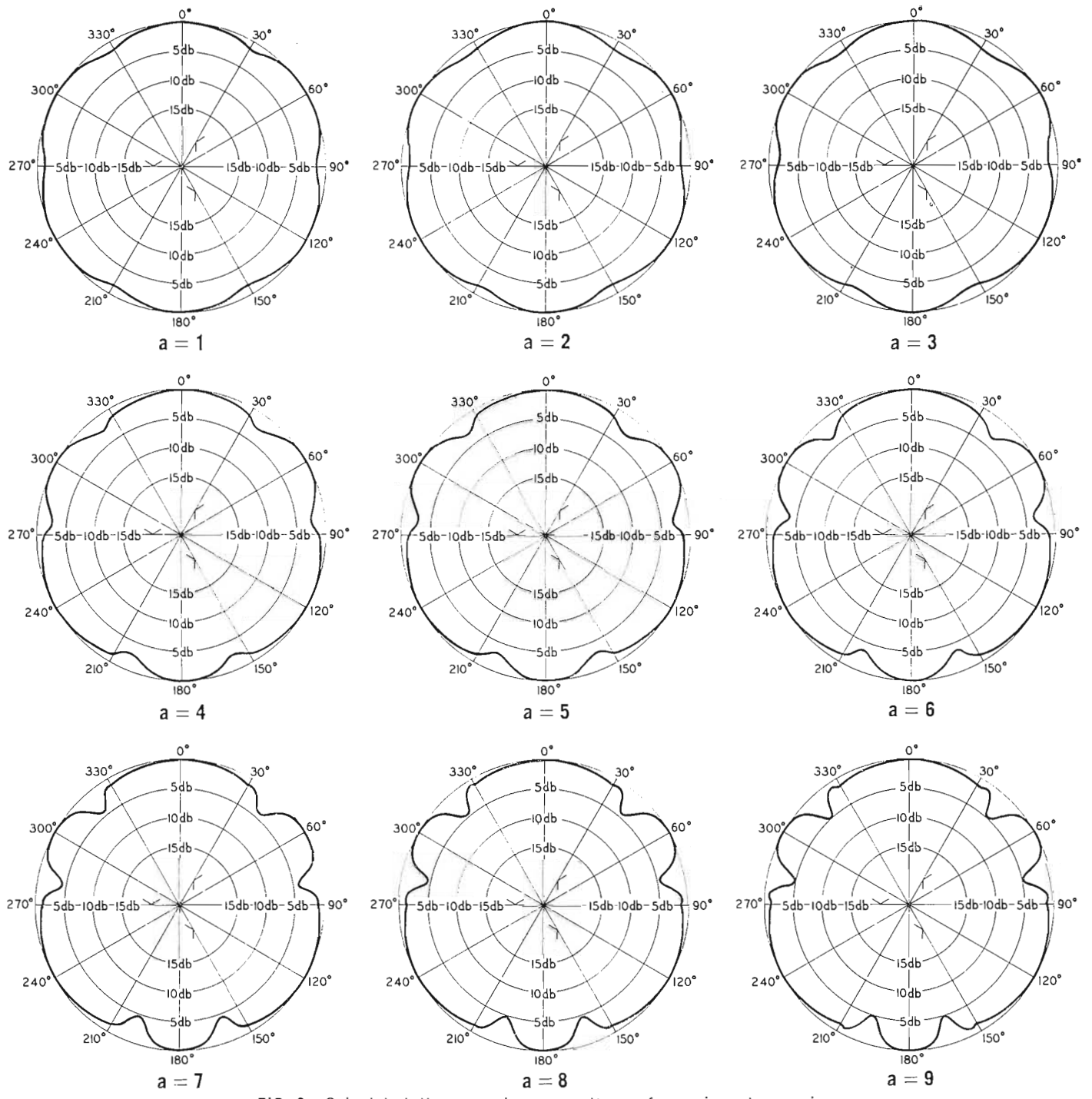
FIG. 9. Calculated three-panel array patterns for various tower sizes.
