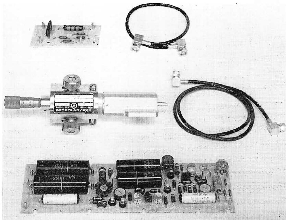
FIG. 5. Functioning elements of TVM-6A off-air monitoring system showing precision calibrated waveguide discriminator cavity (left center) and video component boards. Installation of the transmitter off-air monitor in a TVM-6A transmitter provides fully demodulated and restored signals. The monitor is a separate receiver within the transmitter.
