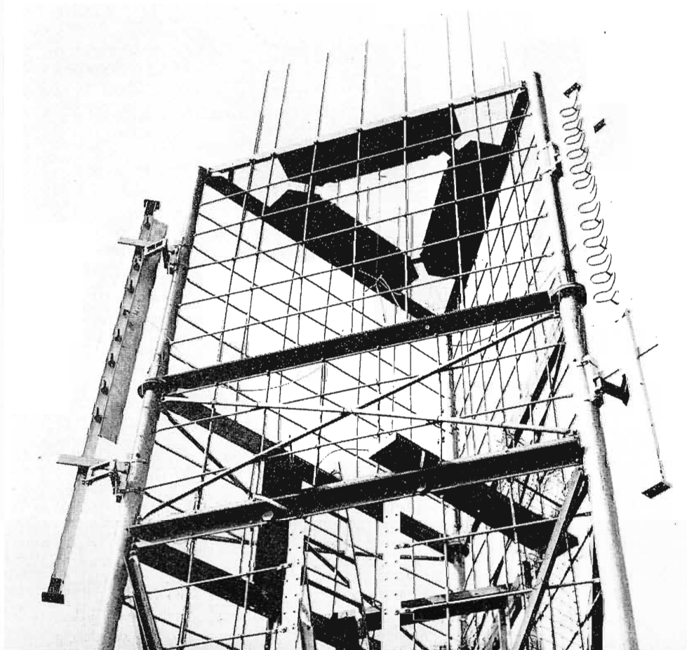
FIG. 2. Three Vee-Zee Panels mounted around a 7.5-foot test tower.
