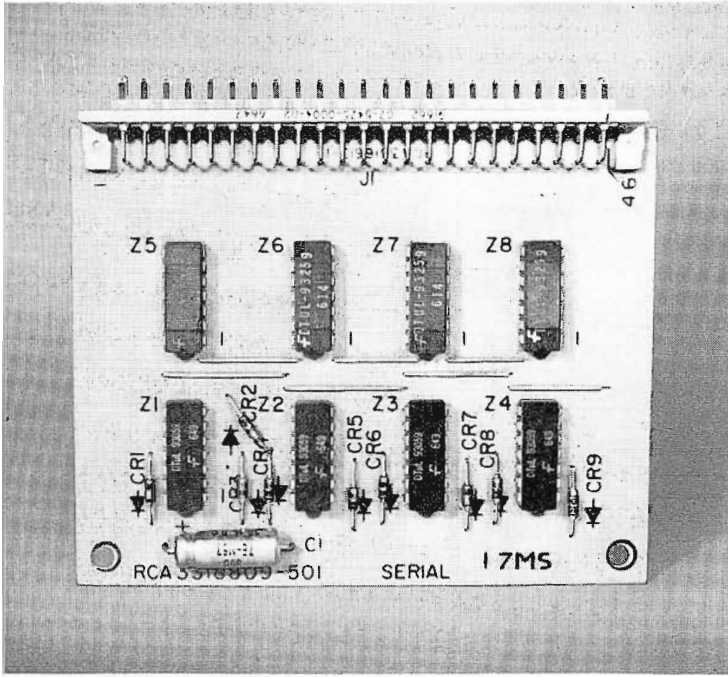
FIG. 6. Front view of plug-in board showing integrated circuitry that contains up to 65 transistors per card.
