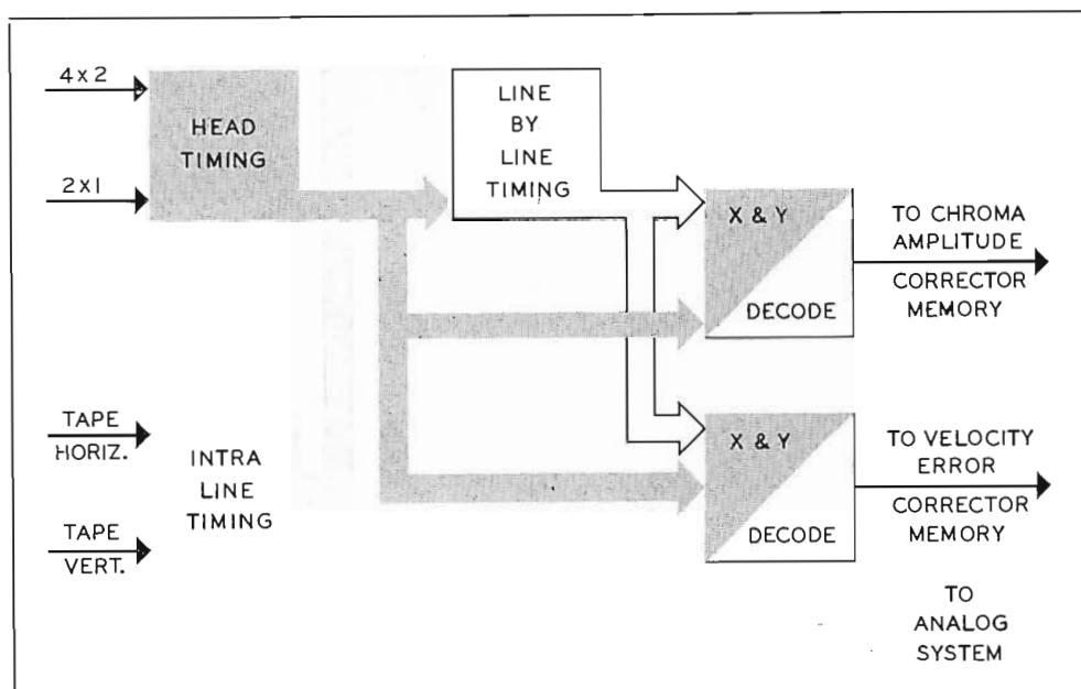
FIG. 12. Block diagram of digital switching system.
