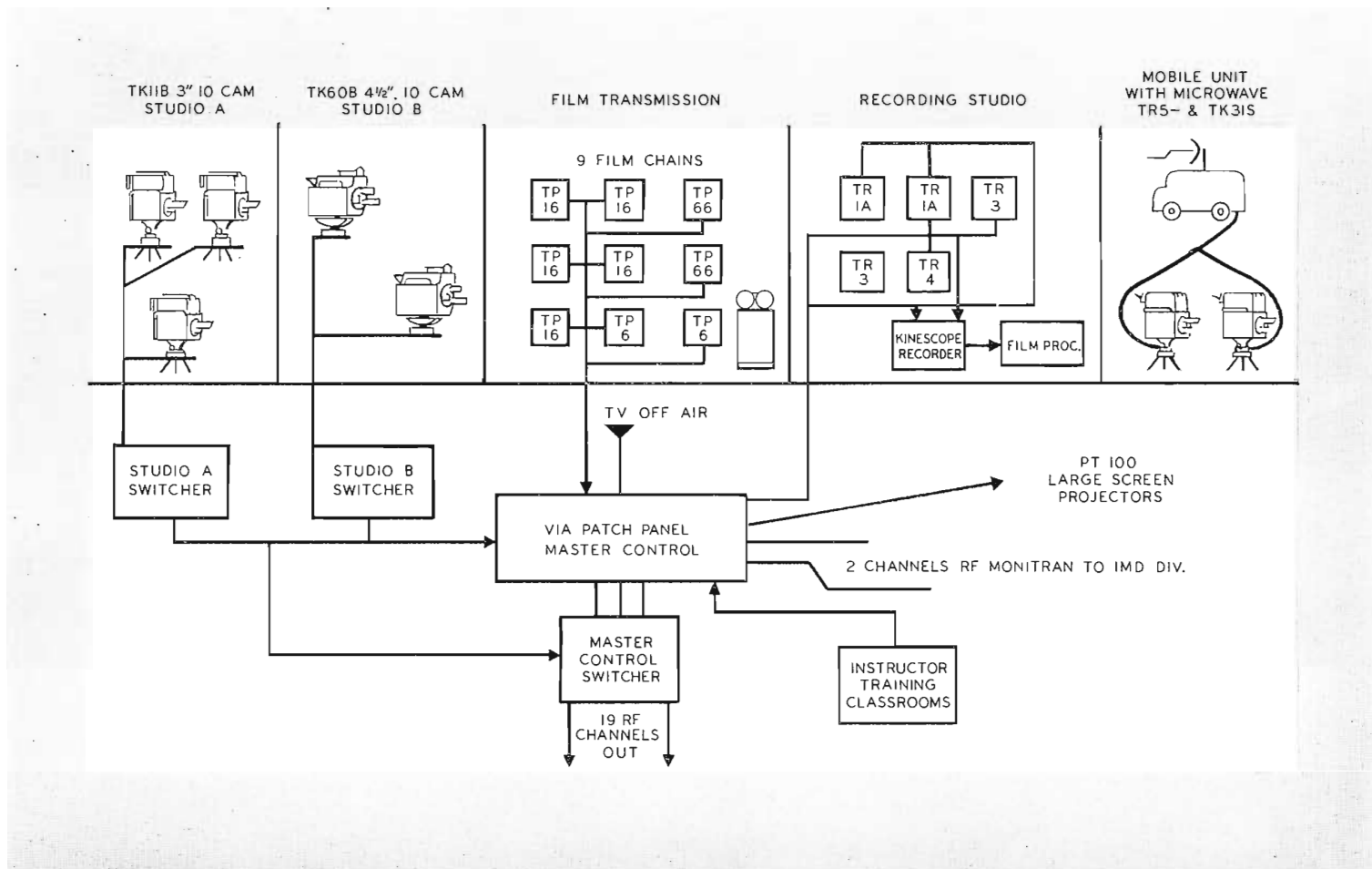
FIG. 27. Block diagram of WFM-TV technical facilities.
