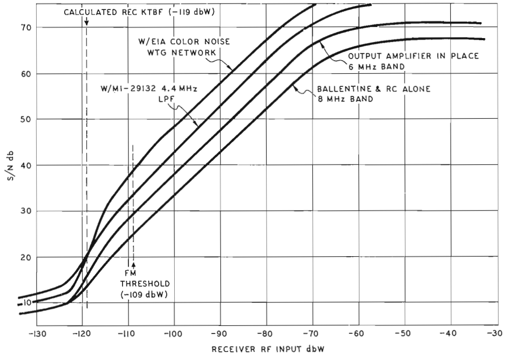
FIG. 12. Typical TVM-6A receiver signal-to-noise performance. Video S/N is in terms of peak-to-peak signal to RMS noise. Receiver RF input is in terms of decibels below one Watt. This plot is highly useful in determining proper antenna alignment and for making periodic measurements of receiver sensitivity.
