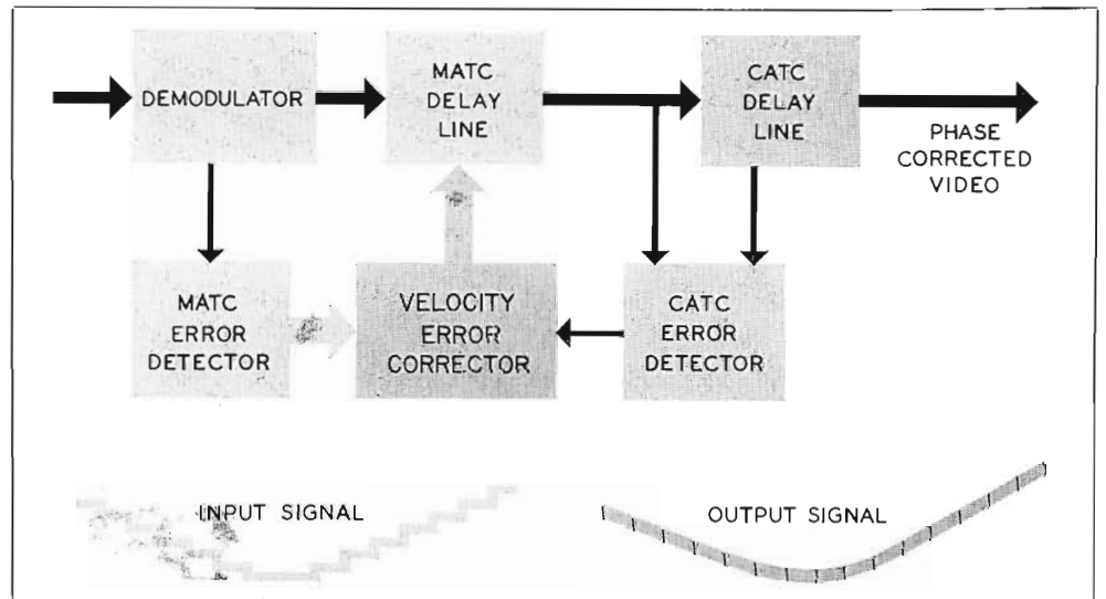
FIG. 9. Block diagram of velocity error corrector circuitry.
