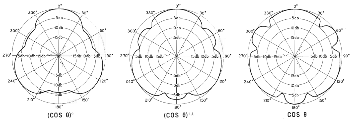
FIG. 10. Calculated three-panel array pattern using (\cos \theta)^p single panel pattern for a=8 .
