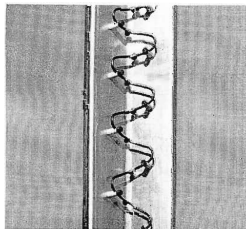
FIG. 8. Zee Panel bent into V-shape.
