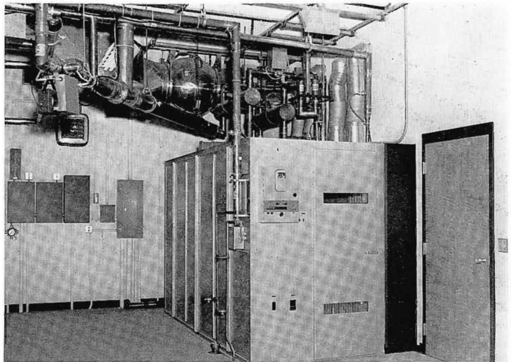
FIG. 4. This view shows the rear of the transmitter with the transmitter enclosure, hybrid couplers, visual low pass filter, tower light indicator panel and other vital parts.
