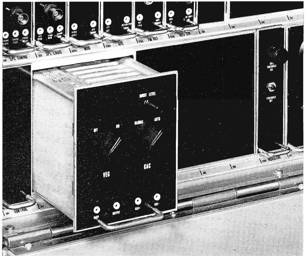
FIG. 4. CAVEC (Chroma Amplitude and Velocity Error Corrector) installed in module bank below tape deck.
