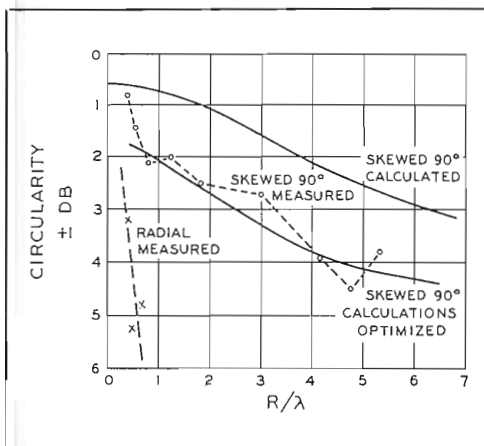
FIG. 14. Curves of circularity vs R/\lambda .
