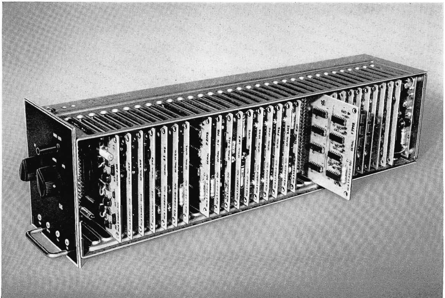
FIG. 5. Modular plug-in frame and solid state plug-in circuit boards provide ease of inspection and service.
