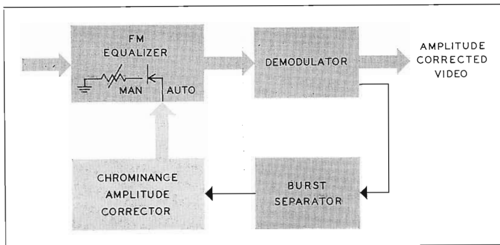
FIG. 11. Block diagram of chrominance amplitude corrector circuitry.
