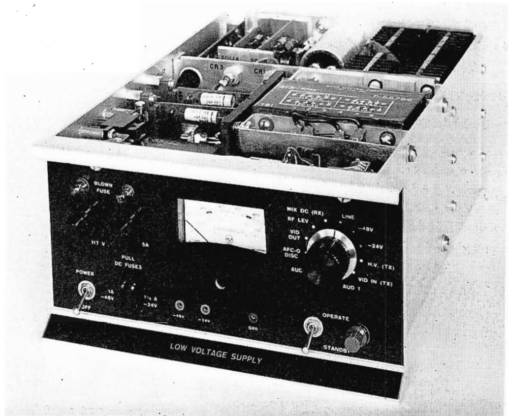
FIG. 8. The low voltage power supply (LVPS) furnishes -24 VDC and -48 VDC to operate all functioning low voltage elements in the system except the klystrons. The LVPS is directly interchangeable between the transmitter and the receiver and serves as the main metering center for all test and program levels in the system. The LVPS is stabilized to maintain \pm 15\% primary line voltage regulation over an ambient temperature range of -30 to +50^\circ Centigrade.
