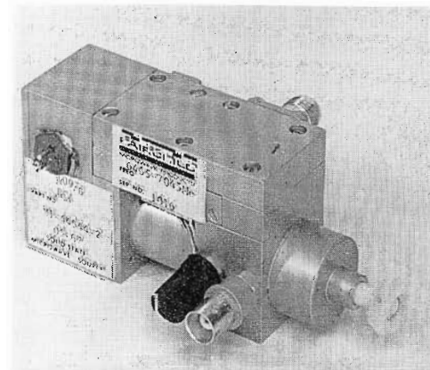
FIG. 11. Solid state local oscillator (LO) source used in the TVM-6A receiver. This non-thermionic device eliminates the need for a klystron tube. The LO source requires a nominal low voltage bias to operate. Mixer signal is generated by a crystal oscillator driving a varactor diode multiplier mounted in a tunable cavity.
