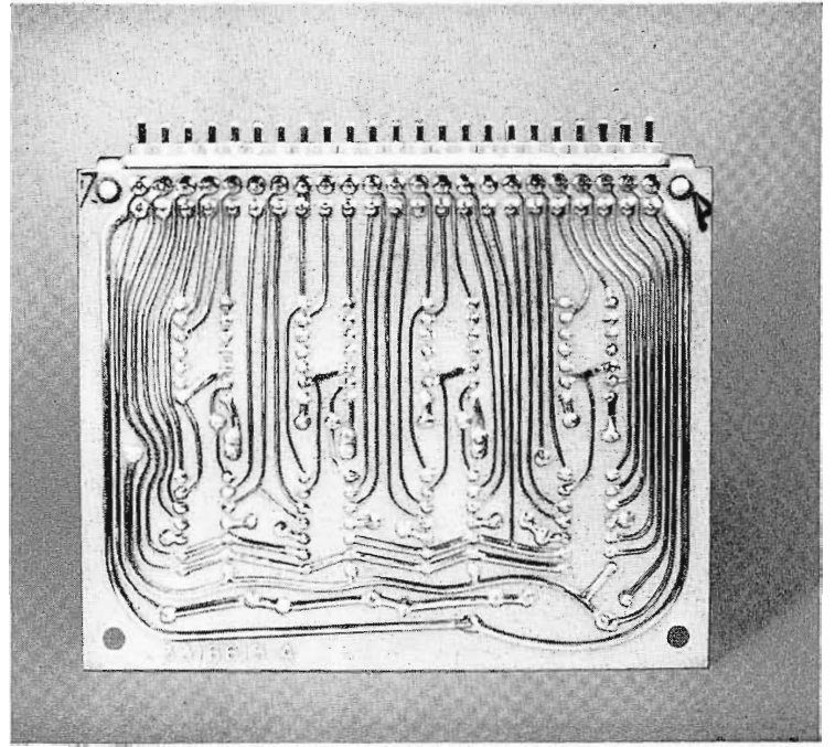
FIG. 7. Wiring interconnections on rear of circuit board.
