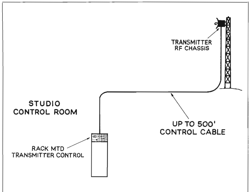
FIG. 2. Diagram illustrating remote application. Control unit mounted in studio with RF chassis mounted remotely on tower or roof top. Built-in equalization provided in equipment for up to 500 feet of control cable. No waveguide is used.
