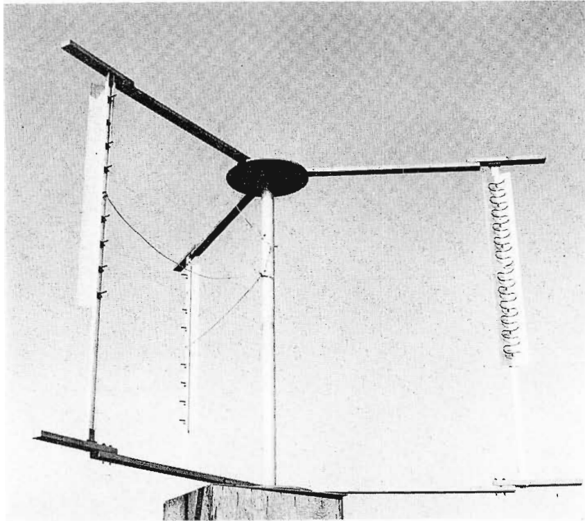
FIG. 11. Three Vee-Zee Panel models mounted around a small pole.
