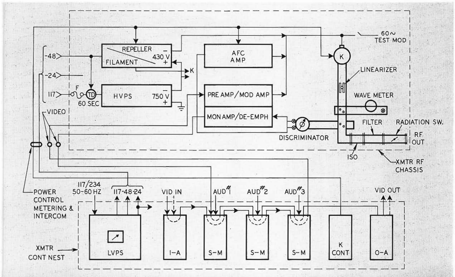
FIG. 7. Transmitter block diagram showing outline of both the RF chassis and the control units. Monitoring of all key program levels is provided by panel meter mounted on the LVPS. Control nest provides space for optional sound modulators or other accessories. Interconnecting cables between both units carry all power, control, metering and intercom circuits.
