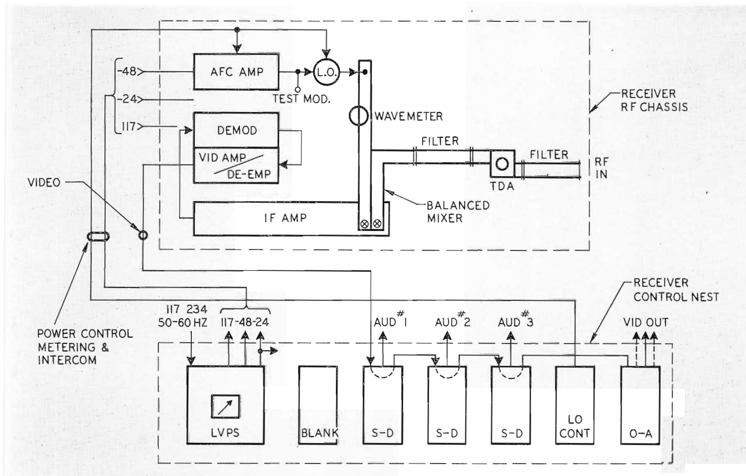
FIG. 10. TVM-6A receiver block diagram showing components in the RF chassis and control units.
