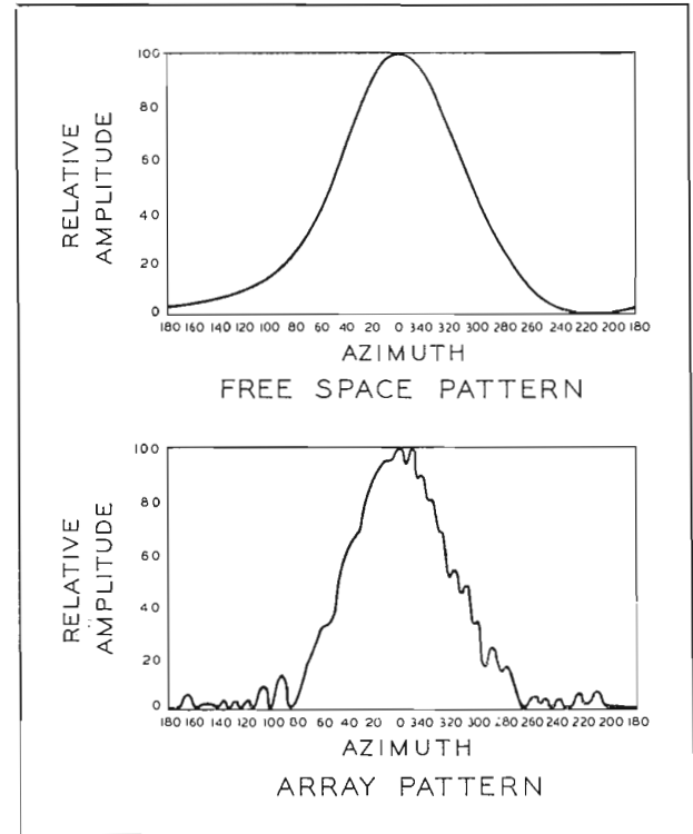
FIG. 12. Vee-Zee single-panel patterns.
