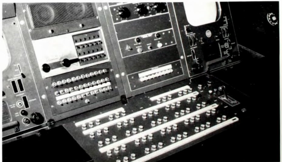
FIG. 15. Close-up of master control panel of TS-40 Transistorized Switching System. Note TM-6 Master Monitor with TS-2 Switcher; also remote controls for TA-9 Stab Amps and Sync-Gen changeover switching. Master intercom is at left.
