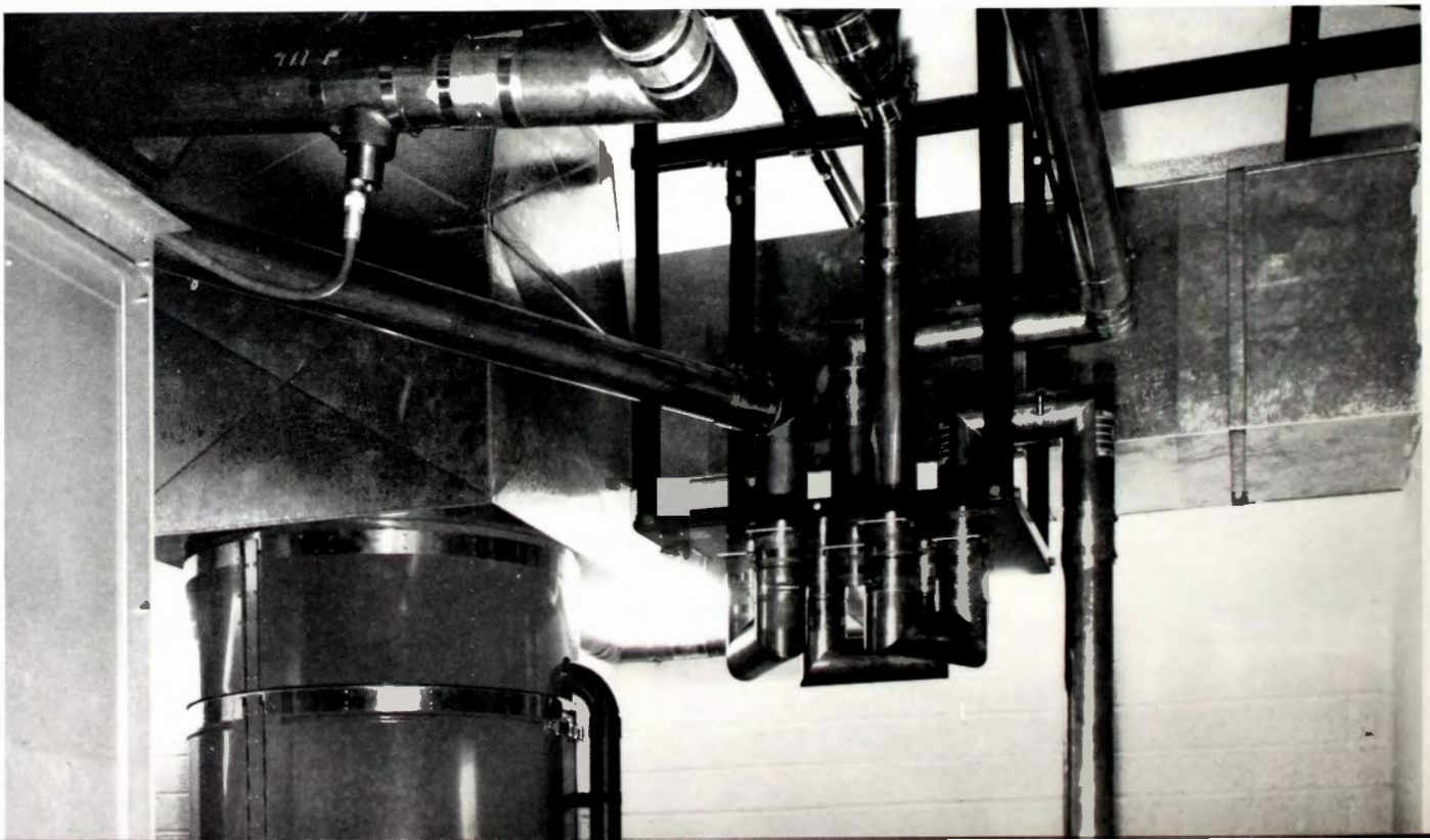
FIG. 6. Rear and side view of aural power amplifier showing the manual rf power patch arrangement in more detail.
