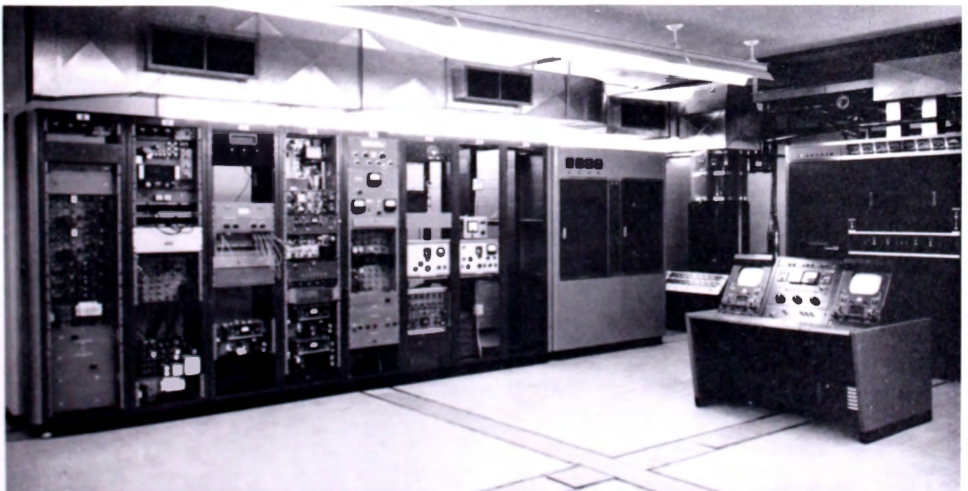
FIG. 4. Interior view of KPHO TV transmitter building showing input, monitoring and test equipment racks and console. The aural PA section of the TT-23CL can be seen in the corner. The visual PA is located in the opposite corner of the room.
