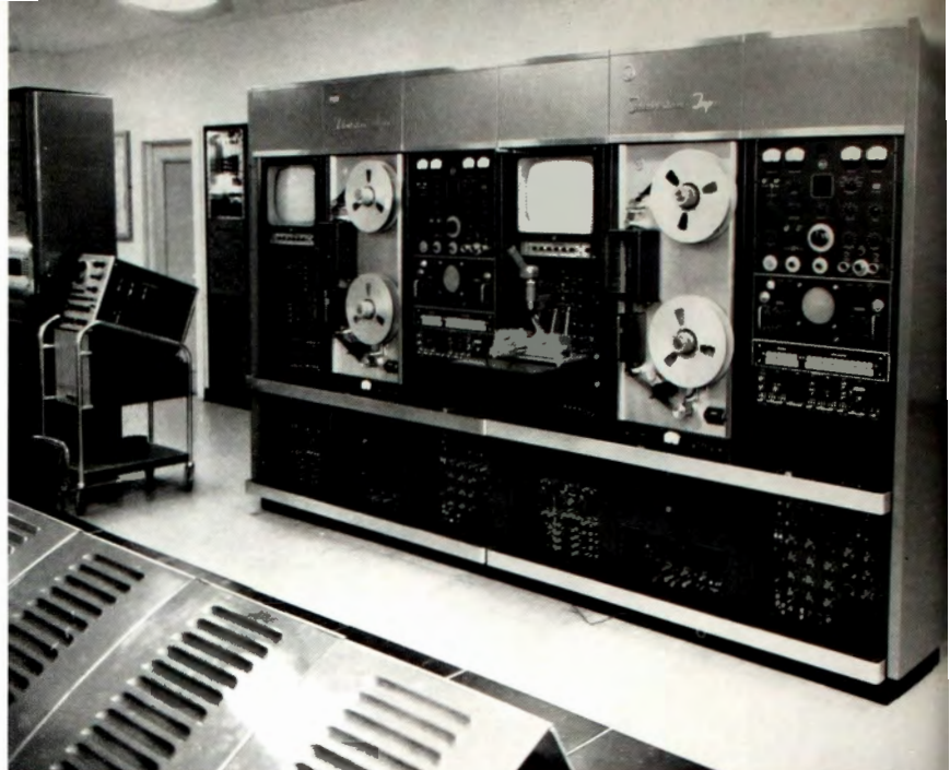
FIG. 20. Two RCA TRT-1B TV Tape Recorders, recently installed in Master Control area.
