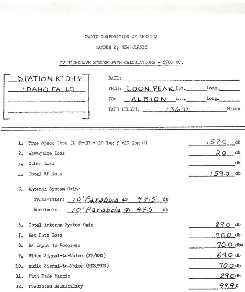
FIG. 4. Path calculation for 136-mile path.
