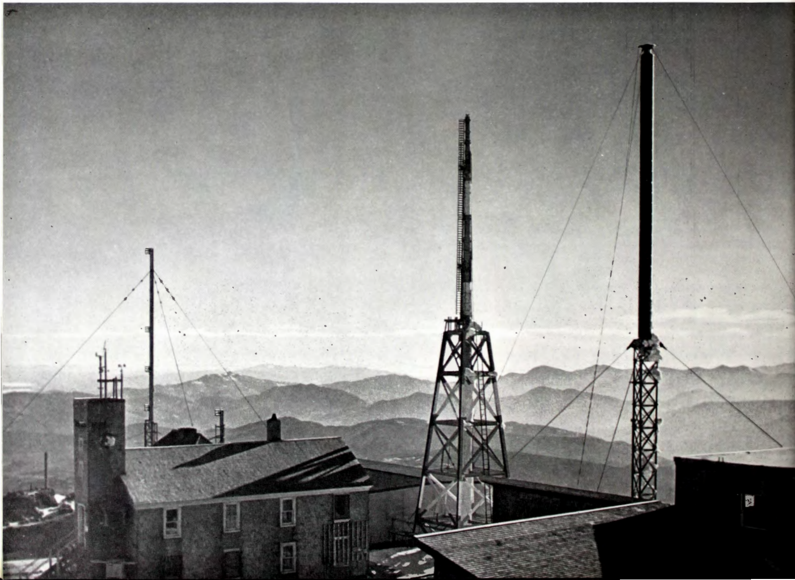
FIG. 1. An overall view of the WMTW installation atop Mt. Washington. The new Traveling Wave Antenna with its radome is shown on the right. WMTW's old antenna is in the center and at the left there are four pole mounted sections of an RCA BFA series of FM antennas. The height of Mt. Washington is shown in contrast to surrounding mountains.
