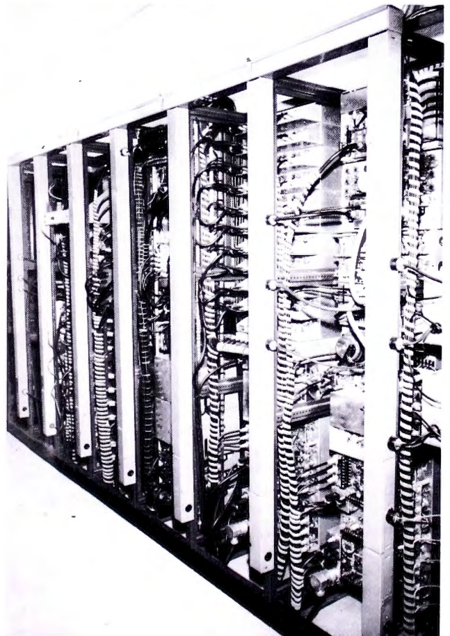
FIG. 18. Rear view of video racks, showing use of lay-in ducts for a-c wiring. Note also the use of Spirap for lacing cables.
