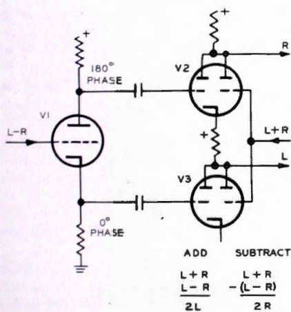
FIG. 6. Typical receiver matrix for FM stereo.
