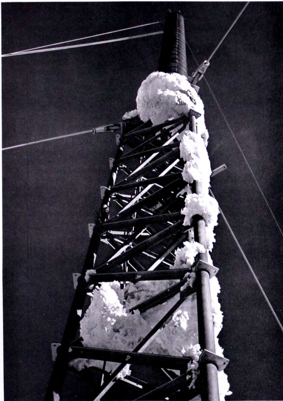
FIG. 2. A close up of the Traveling Wave Antenna. Note top guy arrangement required to support the tower and antenna against extremely high winds. Contrast, ice accumulation on tower with complete freedom from ice on antenna enclosure. This is typical.
