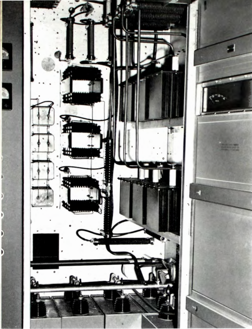
FIG. 4. The new silicon rectifiers are mounted vertically inside the cubicle. Filter capacitors are at the bottom of the cabinet.
