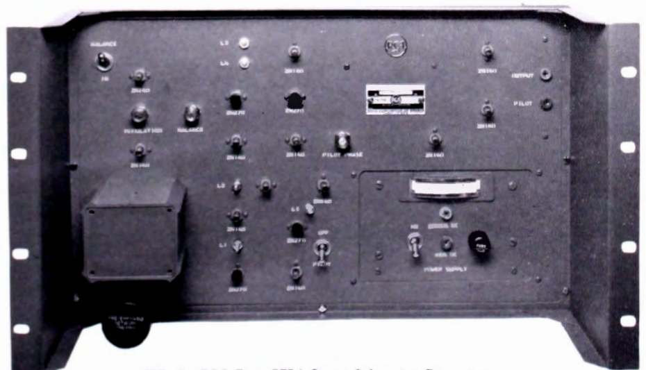
FIG. 3. RCA Type BTS-1 Stereo Subcarrier Generator.
