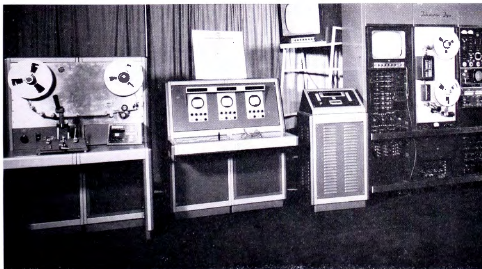
FIG. 3. New TV Tape Editor—developed for NBC by engineers of RCA's Astro-Electronics Division. It facilitates editing of tape programs with a speed and accuracy comparable to present film editing techniques. The television editor may select, view, compare and evaluate groups of frames in tape programs and then select the exact beginning and ending frame of the sequence he wishes to remove or alter.
