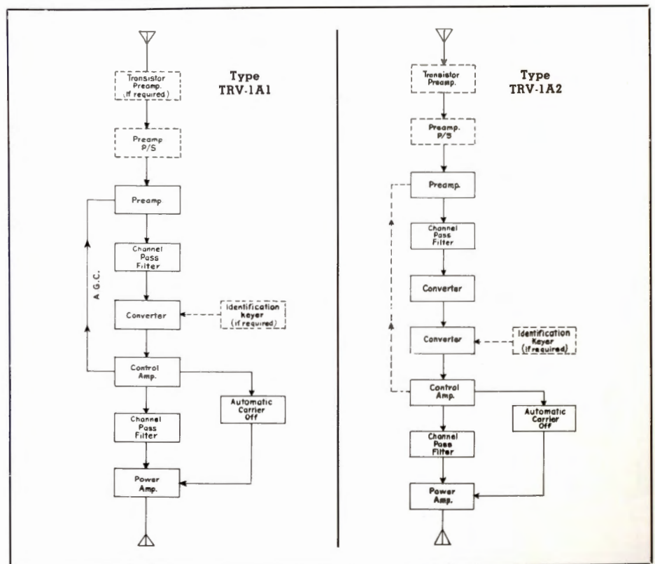
FIG. 1. Single and double conversion translator systems are shown here (left to right, respectively). Each has provision for an identification keyer.
