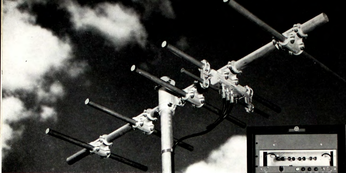
FIG. 3. High-gain yagi antennas assure uniform coverage of translated signals. A single bay unit is shown here. Higher gains are possible if several bays are stacked.
