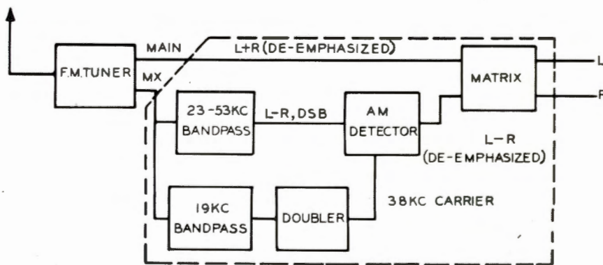
FIG. 5. Block diagram showing how FM stereo is received.
