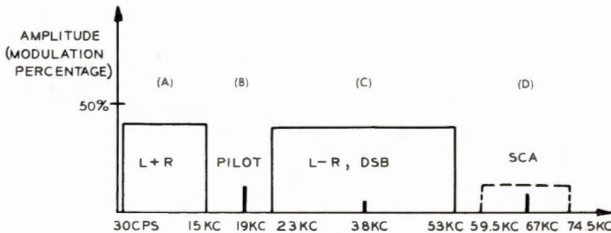
FIG. 4. Total modulating spectrum covered by exciter.
