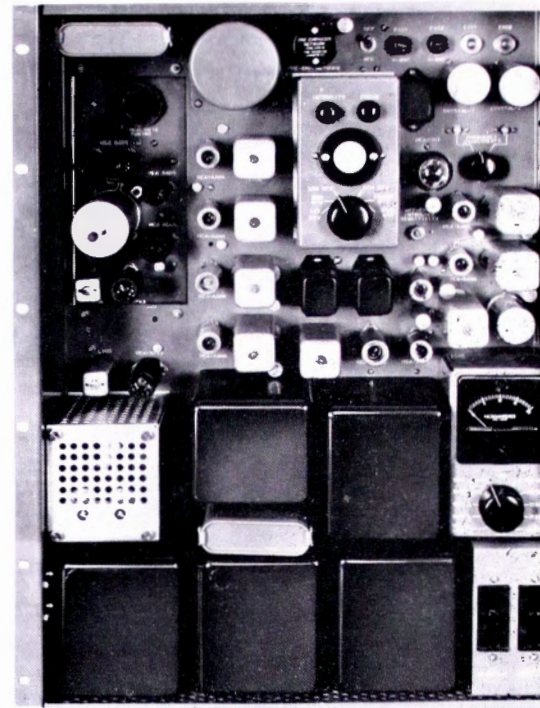
FIG. 2. RCA Type BTE-10B FM Exciter.
