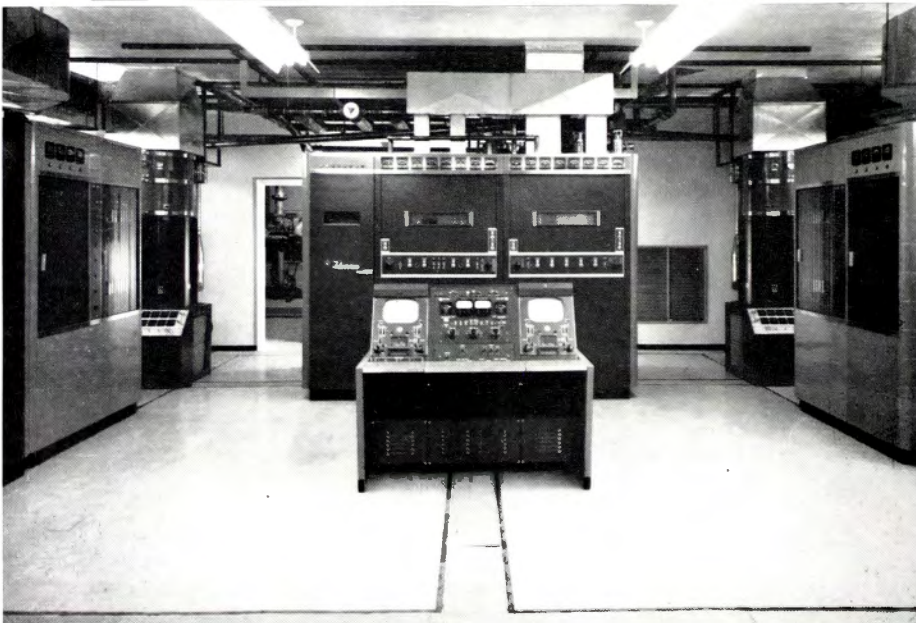
FIG. 2. Interior view of KPHO-TV completed transmitter building showing the control console and the TT-25CL Transmitter in the transmitter building atop South Mountain, 8½ miles south of Phoenix.
