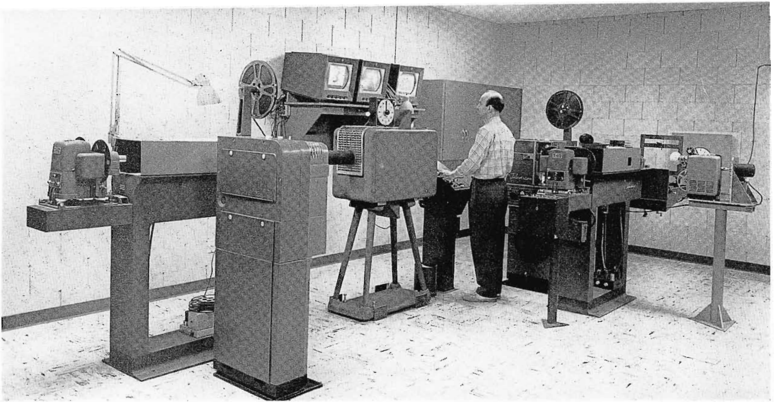
FIG. 16. KAKE-TV film room. There are two vidicon film chains, two TP-6 16-mm Projectors, two TP-11 Multiplexers, a telop, two TP-3C 35-mm Projectors. At far right, note 8-mm movie projector.
