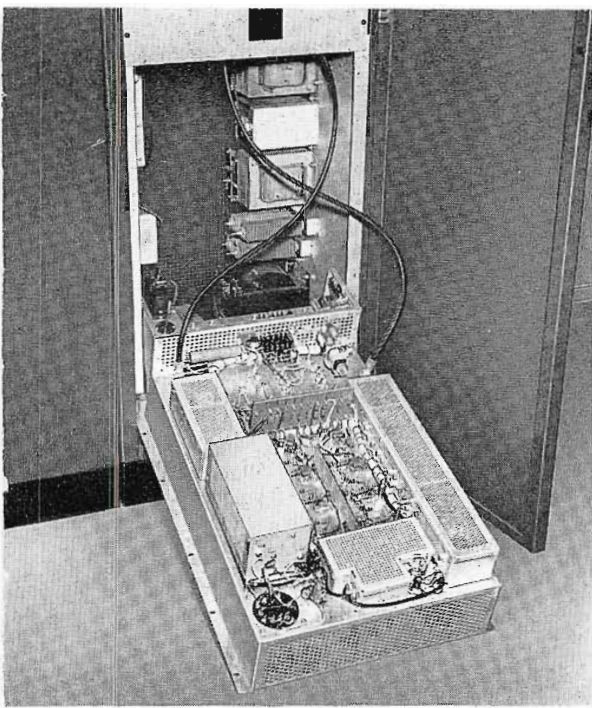
FIG. 3. Aural-visual exciter section of TTL-100AL/AH is easily tilted forward for servicing. Exciter is same type being used in many other RCA TV Transmitters, such as the TT-2BH, TT-6AL, and TT-25CL.
