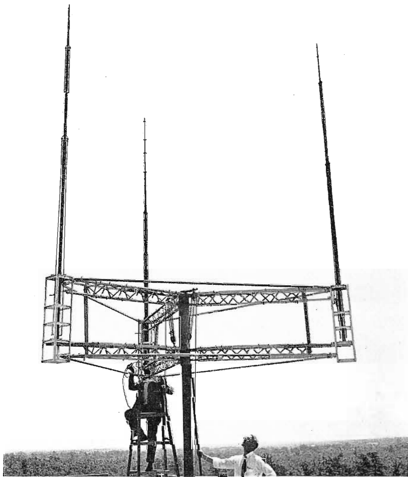
FIG. 10. Scale model of a Multiple Antenna arrangement, employing three superturnstiles, undergoing test.
