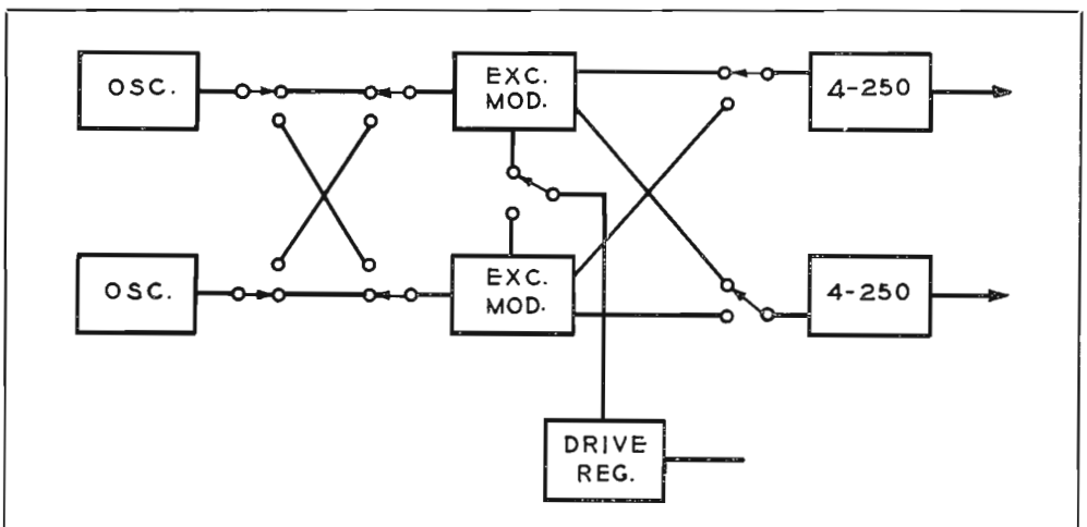
FIG. 4. Cross switching of exciter-modulator units is provided to permit either push button or remote transfer from one unit to the other. DC power remains on transmitter during switching, and automatically sequenced transfer results in only momentary loss of carrier.
