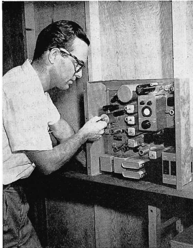
FIG. 10. All operating adjustments on the BTX-1A Subcarrier Generator are accessible from the front of the unit as shown here. Again the convenient built-in oscilloscope can be used to observe operation of AFC circuits. The author is shown checking divider circuits.
