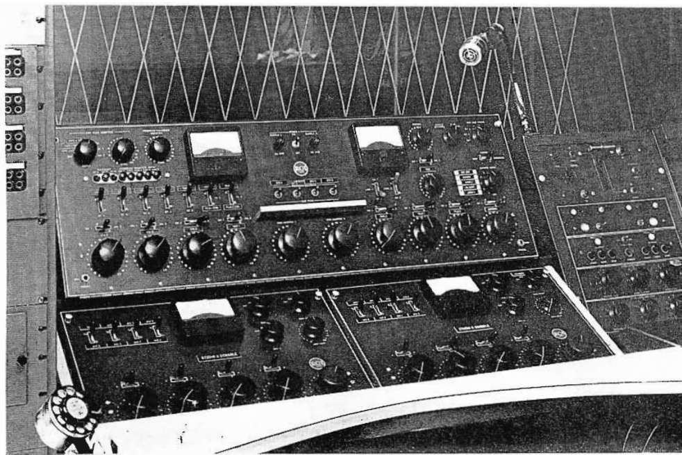
FIG. 4. Three consolettes are shown at the single operating position in the WCSH-TV control room. The BC-6A Consolette controls network, film and tape facilities, in addition to controlling the outputs of the two BC-5B Consolettes.
