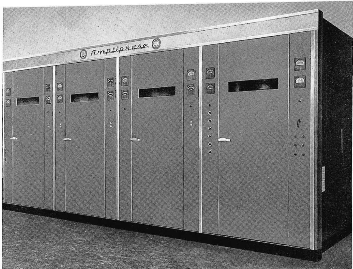
FIG. 1. This is the RCA Type BTA-50G "Ampliphase" Transmitter. Remote control system described in the article is ideal for this transmitter.
