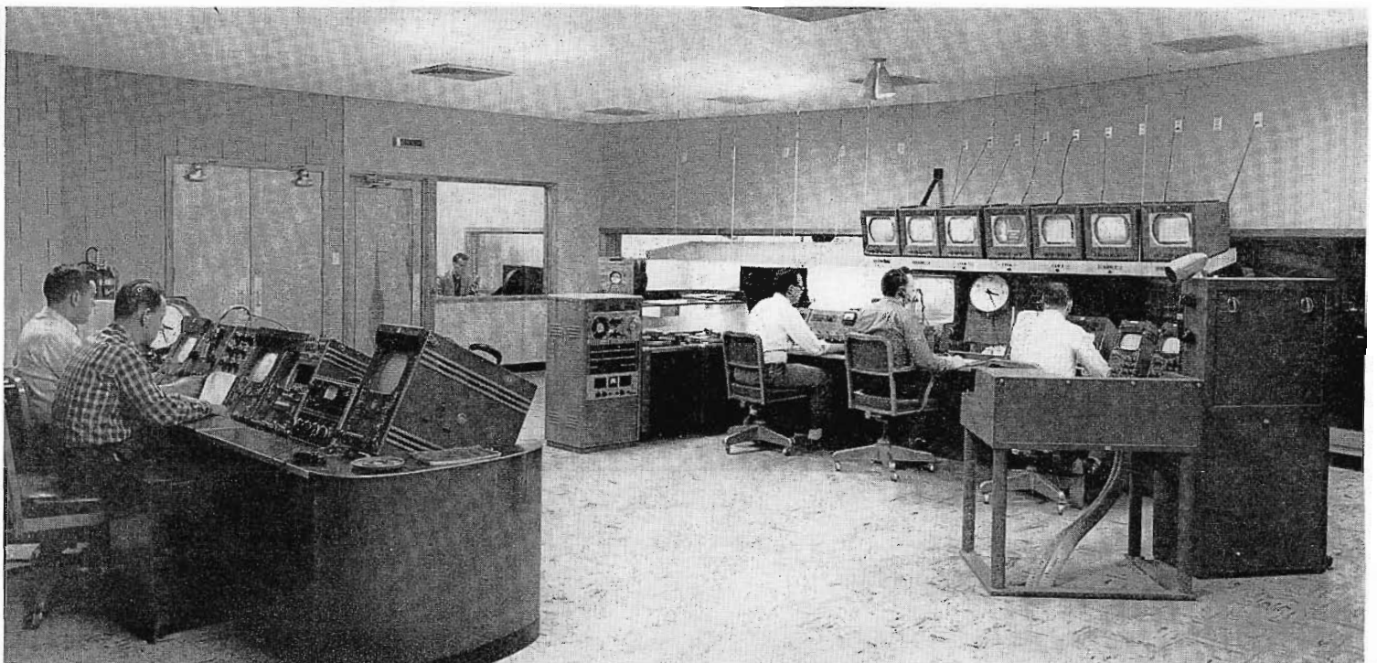
FIG. 11. Master control, at left, showing two operators. Studio control at right showing three operators, has following arrangement (left to right): tape recorder and microphone patch panel; two BQ-2B Turntables; audio control; director's position; video control, lighting.
