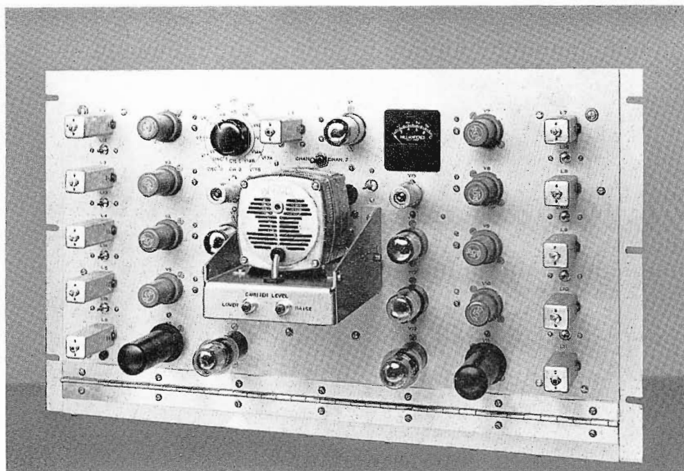
FIG. 7. Carrier level (power output control) is varied from a remote position with a friction clutch motor mounted on the exciter-modulator as shown here. Power variations are limited to \pm 10 percent by positive mechanical stops on the motor.
