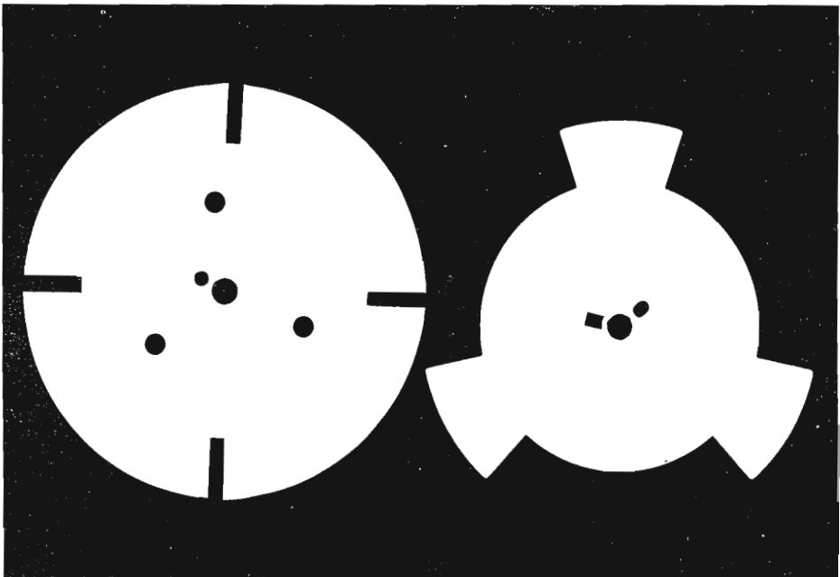
FIG. 20. Modified shutter for 8-mm movie projector, shown at left. Regular shutter is at right.
