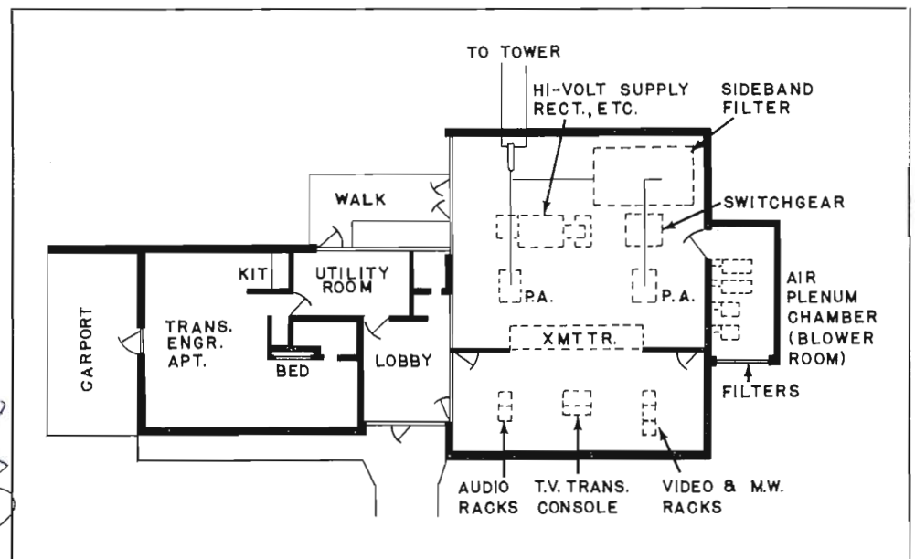
FIG. 25. Floor plan of transmitter building.
