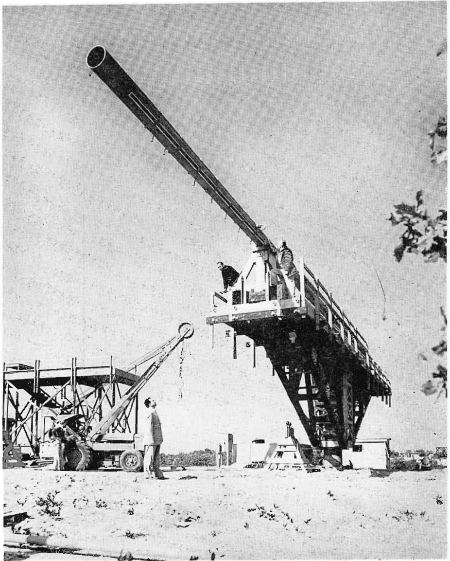
FIG. 1. An ultra-gain TV antenna is shown on a 15-ton turntable at the RCA Antenna Testsite.
