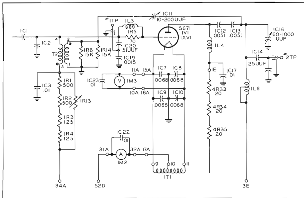
FIG. 5. This is the final amplifier circuit showing the special broad-band neutralizing transformers. Neutralization is effective over entire broadcast band and up to approximately 2.5 mc.
