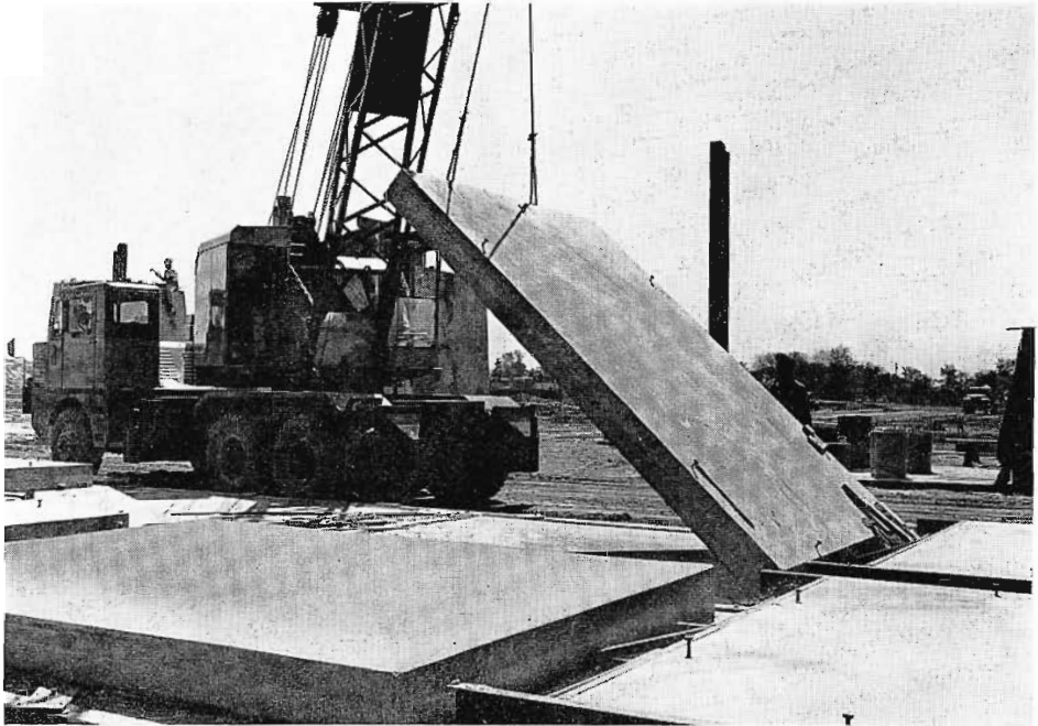
FIG. 5. Building is constructed of precast cement panels.
