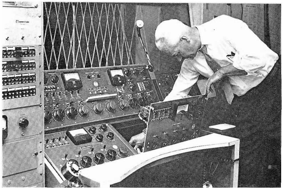
FIG. 7. The BC-5B Consolettes can be serviced by lifting up the front panel as shown here (or as shown in Fig. 8).
