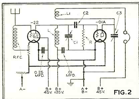
At the top, Fig. 1 shows the simplest form of short-wave receiver circuit while Fig. 2 below, shows the same circuit with a stage of untuned r.f. amplification added to it
