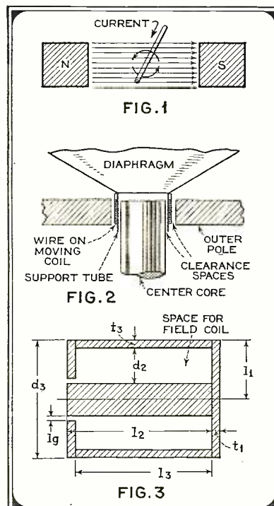
The three figures above tend to illustrate the general principles involved in the construction and operation of electrodynamic loud speakers
