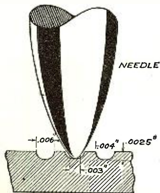
Fig. 7 (at right)—Behavior of a phonograph pick-up with various types of needles
