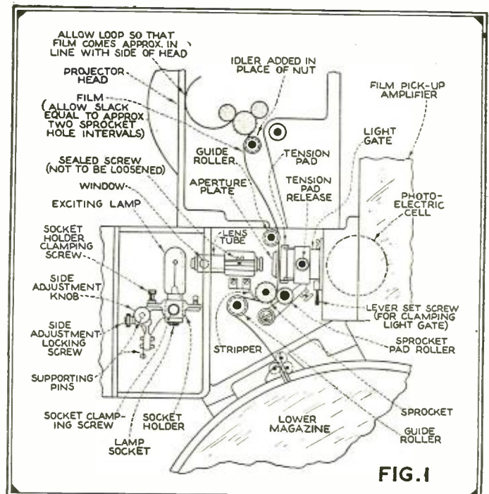
Above: The sound-on-film mechanism in the recorder is placed just below the projector head. The drawing, above, is self-explanatory
