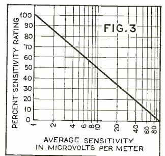
The per cent. sensitivity rating of a receiver is determined from this curve. The average sensitivity obtained at 600, 1,000 and 1,400 kc. is calculated and, knowing this average sensitivity, the per cent. rating is determined
