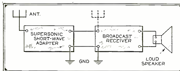
Fig. 1. A diagrammatic representation of the circuit arrangement employed in connecting the Supersonic short-wave adapter to a broadcast receiver
