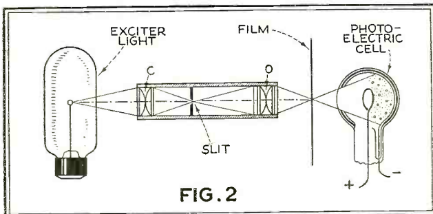
A general idea of the optical system of a reproducer is given in the above drawing showing the exciter lamp, the lenses and the photoelectric cell
