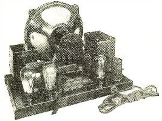
Compact yet accessible is the power supply-audio channel-speaker chassis of the Grebe audio unit
