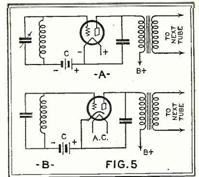
Fig. 5. Circuits for plate circuit detection, showing typical arrangements for use with d.c. and a.c. tubes. A is the circuit for d.c. tubes and B is the circuit for a.c. tubes
