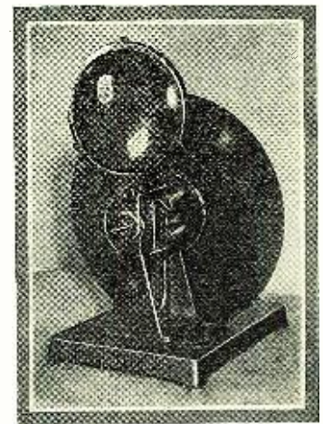
Fig. 2. Televisor driven by eddy current motor with 60-cycle synchronizing phonic wheel. The wheel is on the back of the disc
