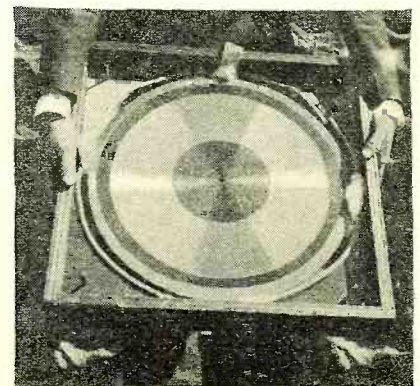
At the left are shown the bright metal stamper which stamps the records and a finished record ready for rebroadcasting purposes
