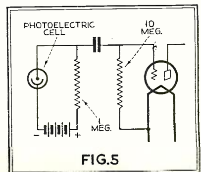
The diagram of a resistance-coupled photo-electric cell amplifier, otherwise known as a "peck"
