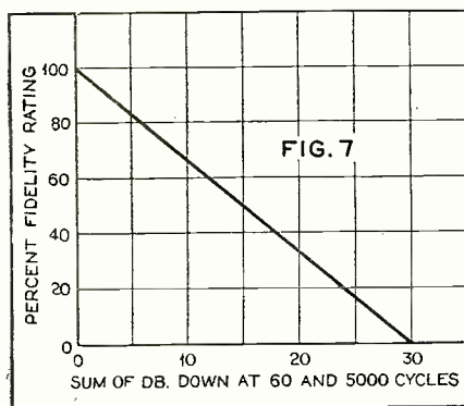
The fidelity rating is determined by measuring the loss in db. at 60 and 5,000 cycles, adding them together to obtain the overall loss and then using this figure of overall loss to determine the fidelity rating from this curve
