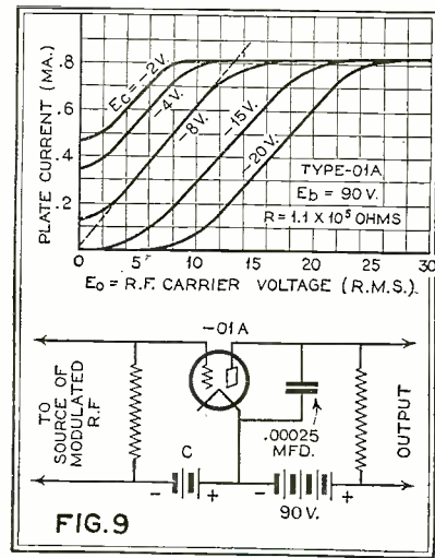
Fig. 9. The diagram may be used to determine the correct operating point for least distortion. The center point of the straight portion of each curve is the best operating point
