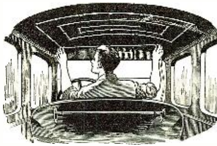
Fig. 1. Showing how wire or metalized tape may be tacked to the roof of a car to furnish satisfactory antenna for the auto-radio receiver
