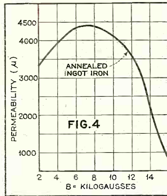
FIG. 4 The permeability curve of annealed ingot iron
