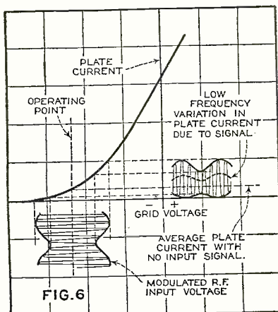
Fig. 6. How the plate circuit detector works. The modulated r.f. impressed on the grid causes the plate current to vary along the curved portion of the plate current curve
