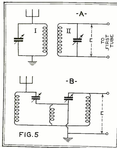
Fig. 5. Two systems of band-pass pre-selector circuits. A modification of "B" has been employed in the receiver whose design characteristics are described here
