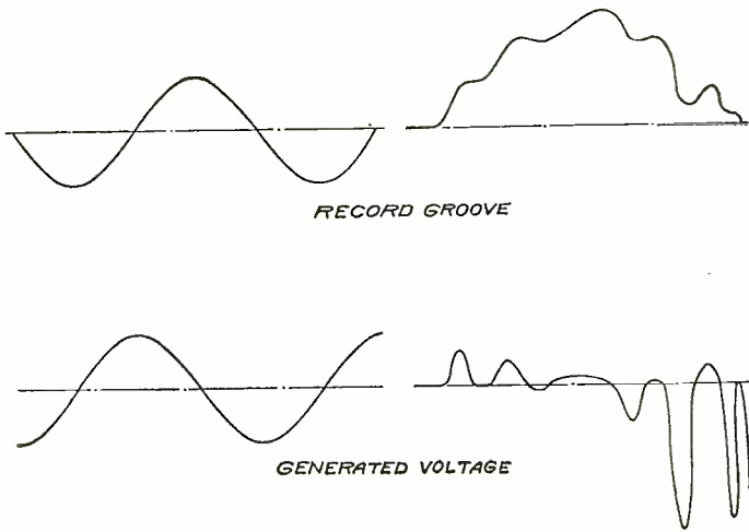
Fig. 9—Groove relation to voltage generated
