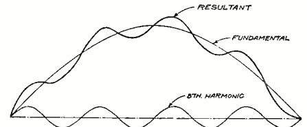
Fig. 12—Resultant of fundamental and 8th harmonic
