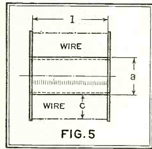
FIG. 5 The core form for a typical field coil
