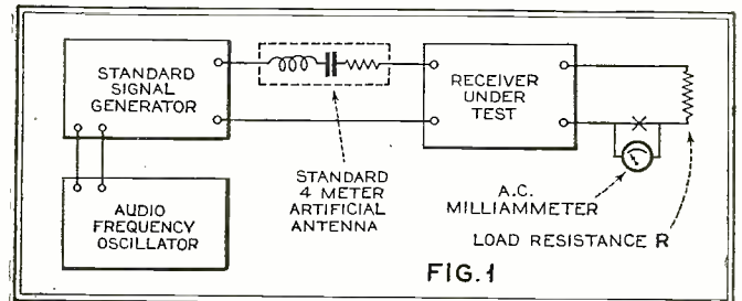
The fundamental circuit arrangement for measurements of the overall characteristics of radio receivers. The a.f. oscillator is used to modulate the r.f. voltages produced by the standard signal generator. The input to the radio receiver is adjusted to give the standard output of 50 milliwatts in the load resistance R
