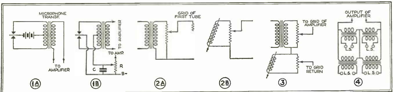
Fig. 1A shows how a double-button microphone is connected to the primary of a coupling transformer. Fig. 1B shows how, in place of the "mike" battery, current is obtained from the B power supply. Fig. 2A shows the generally accepted type of "mike" gain control, a resistance shunted across the transformer secondary. Fig. 2B shows a phonograph pick-up volume control system, while Fig. 3 shows how the "mike" and phonograph circuits are combined. In Fig. 4 the circuit is shown for connecting speakers in multiple in the amplifier's output
