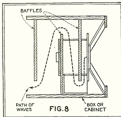
A sketch showing the general constructional details of a proposed dynamic speaker baffle, showing the obstructed path to the rear which confronts the back sound wave
