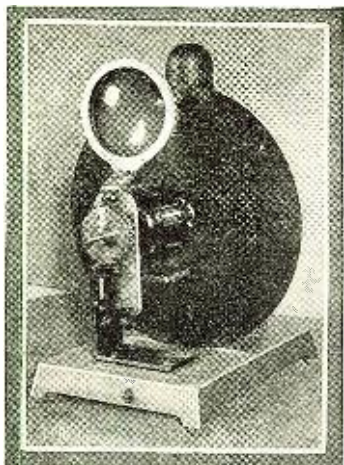
Fig. 5. Televisor driven by a d.c. motor and held in synchronism by the phonic wheel shown in the foreground. Synchronizing pulses are obtained at picture line frequency, 720 cycles
