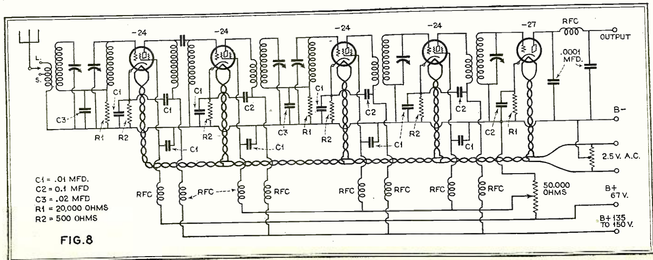
Fig. 8. The complete five-tube circuit evolved from the research which was conducted in the investigation of the design considerations treated in this article
