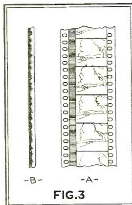
Two types of sound-on-film: A shows the variable density constant width type, and B the variable width constant density type
