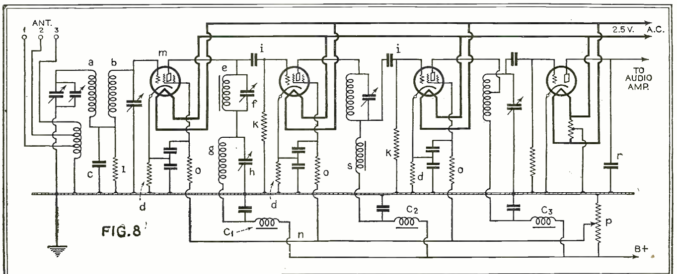
Fig. 8. The circuit of a four-tube tuner employing three stages of tuned r.f., two of which employ the band-pass system described here, while the antenna stage makes use of one of the standard pre-selector circuits
