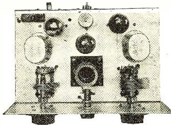
A top view of the revamped receiver. Note how a symmetrical layout has been maintained
