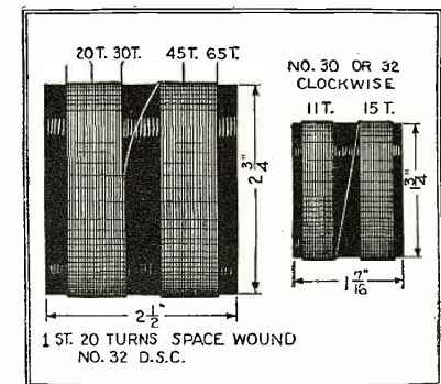
2176 DO.—The design of an oscillator and an oscillator coil in conjunction with a .0005- \mu f. condenser, in a super-heterodyne receiver employing 50 to 60 KC type intermediate frequency transformer.
