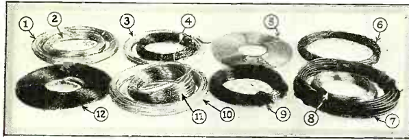
An assortment of aerial wire. 1, stranded; 2, braided; 3, solid; 4, enamel-covered stranded; 5, braided tape; 6, enamel-covered solid; 7, heavy insulated ground wire; 8, guy wire; 9, flexible enamel-covered; 10, stranded tinned copper; 11, enameled-stranded and 12, enameled braided tape.
