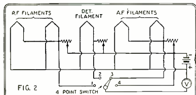
When more than one rheostat is used for tubes, voltmeter connections should be made as shown above.
