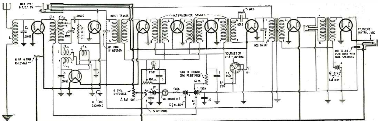
The nine-tube Super-Heterodyne has an audio-frequency amplifier that is made of standard apparatus. The grid and plate voltages must be determined experimentally.
