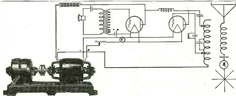
Item 37. 2 unit four bearing set, delivering 1000 volts, 600 watts for plate and 12 volts, 300 watts for filament. The "ESCO" Set is shown here furnishing Power Supply for 4-50 watters in a phone or telegraph set. This is the Item used by CB28 in pioneer achievement of the first two way amateur wireless communication between North and South America.
