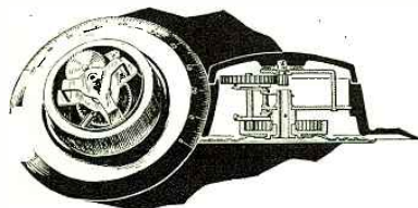
The gears in this vernier dial are cleverly arranged so that there is no chance of any backlash in the dial's movement.
