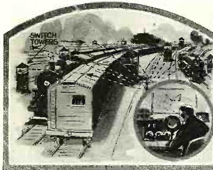
The Illinois Central Railroad has reduced one yard crew from 228 to 27 men by the use of twelve microphones and a central power circuit operating loud speakers, together with an automatic braking system. The dispatchers' orders and switchmen's answers are heard throughout the yard.
