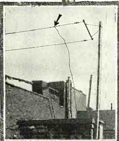
Above: The lead-in should have been taken off from the end of the aerial and the aerial itself guyed with ropes. Right: This ribbon aerial is well fastened to the pipe with a piece of rope but is not insulated.
