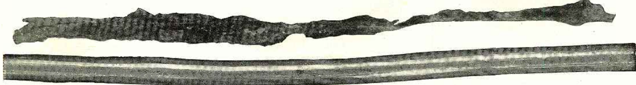
A photograph of two sections of solid aerial wire subjected to extreme climatic conditions. It is clear that the upper wire had no protective coating. One should not expect such damage under normal conditions; but it goes to show what corrosion the atmosphere can effect on metallic objects.
