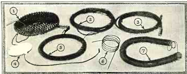
Left: Aerial and ground wire. They are: 1, stamped copper ribbon; 2, stranded copper; 3, lightning ground wire; 4, copper ribbon; 5, enameled-stranded; 6, heavy-duty copper ground wire; 7, indoor spring aerial. Above: a complete spring aerial and a group of insulators for use in conjunction with outdoor aerials. Illustrations courtesy Parker-Acolus Corp., Radear Mfg. Co., Acme Wire Co.
