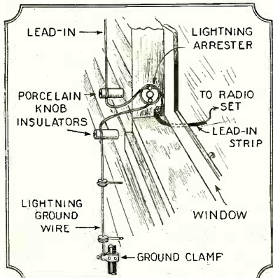
Details of an aerial and lightning-ground installation on the side of a house.
