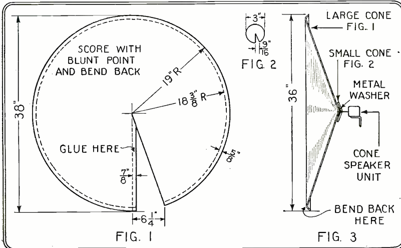
Details of the paper cone. Great care should be exercised in forming the "skirt" around the edge of the cone.
