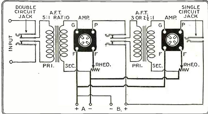
Q. 2177.—The circuit diagram of a conventional two-stage audio amplifier, with jack connections after each stage. This amplifier may be added to a one-tube receiver, or any other type in which audio-frequency amplification is desired after a detector tube.
