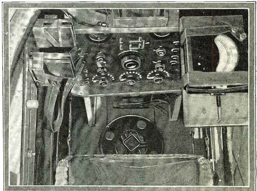
The radio set installed in an airplane. The reel containing the antenna is under the pilot's seat.
