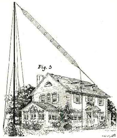
A cage antenna composed of a number of wires attached to a series of metal rings. The lead-in is taken from the low end.
