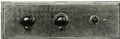
The panel view of the Reflex Five, showing the two tuning, and one volume, controls. Courtesy Acme Apparatus Co.
