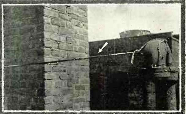
Above: The lead-in should have been taken off from the end of the aerial and the aerial itself guyed with ropes. Right: This ribbon aerial is well fastened to the pipe with a piece of rope but is not insulated.
