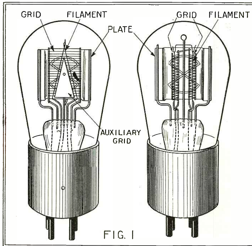
Constructional details of the two vacuum tubes described in this article. The auxiliary grid shown in the left-hand tube functions as a control element. A number of circuits particularly adaptable to this tube are shown above.
