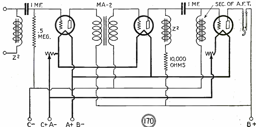
A special type of audio amplifier which, when efficiently constructed with a good grade of apparatus, is capable of meeting the most exacting requirements of any "music-lover." A power tube should be used in the last stage or socket for highest efficiency.
