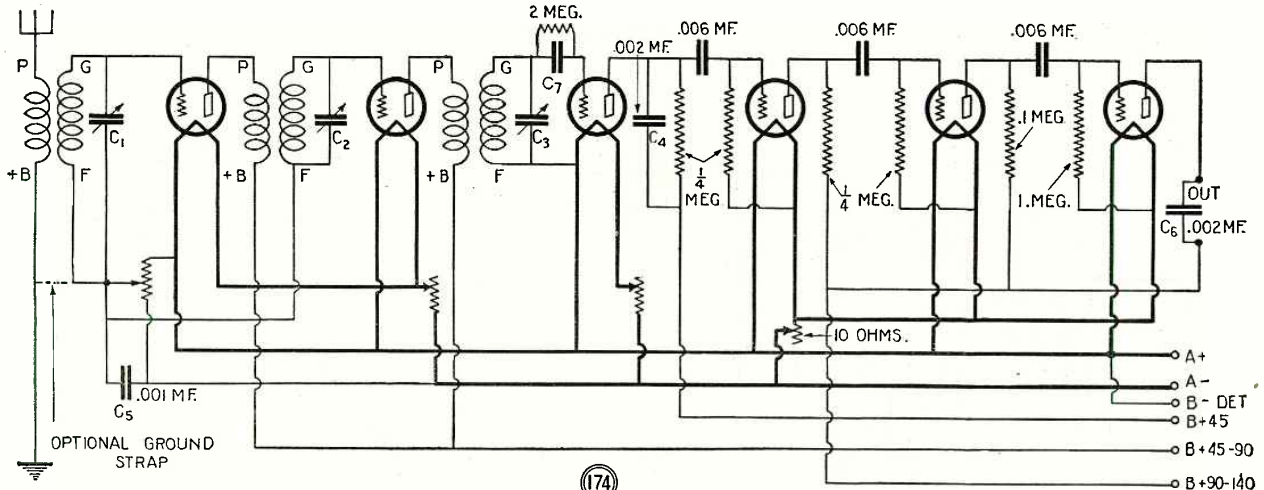
A receiving circuit with none of the frills which usually result in troublesome adjustments, complicated tuning, critical results, etc. Stations received by a set employing this circuit are loud, clear and consistent and are tuned in with ease. Clarified reception is obtained, due to the resistance-coupled audio amplifier employed.
