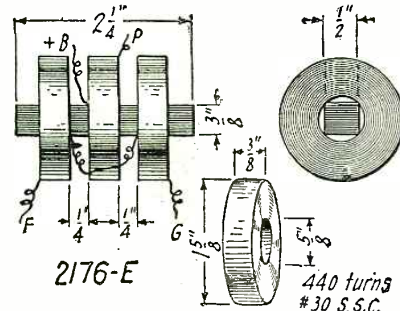
The design of a tuned intermediate frequency transformer, employing an iron core. A small variable condenser, approximately .00025- \mu f., is connected across the secondary and varies the wave-length range from approximately 2,000 to 7,000 meters.
