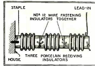
A simple sectional stand-off insulator.
