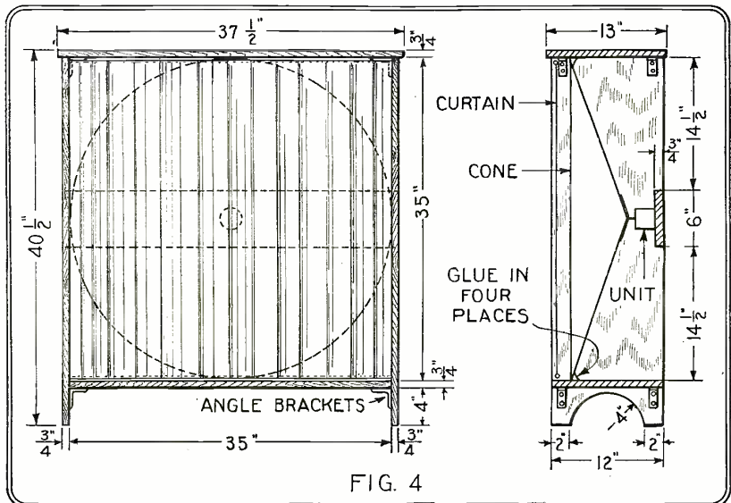
Constructional details of the loud speaker cabinet-table. The skirts of the cone are glued to the boards at four places, as indicated.
