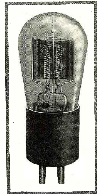
A tube so designed that it has a very low inter-element capacity. Note the slender two-section grid.
