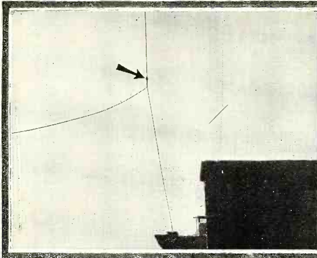
Above: As an aerial this is a good ground. It will be noted that the wire touches the metal framework of the skylight. In consequence very little current reaches the set. Left: This man's aerial was too long so he shortened it by inserting an insulator as indicated by the arrow. Good, but the lead-in should have been taken off at the insulator eye, to relieve the strain on the wire.
