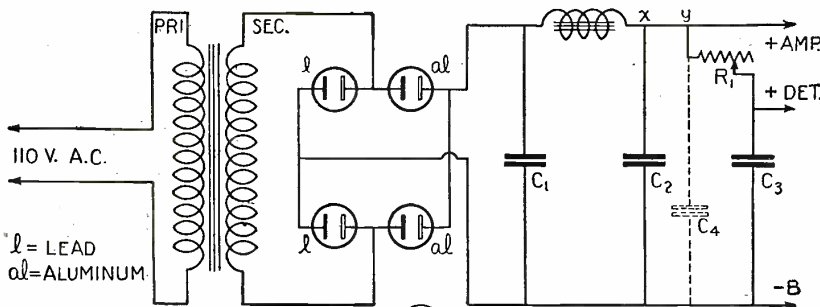
A very efficient "B" eliminator employing chemical rectification. The cost of construction of this eliminator is very small and the current output obtained is as pure "D.C." as can ever be obtained from any similar type of instrument. The step-up transformer should be purchased.
