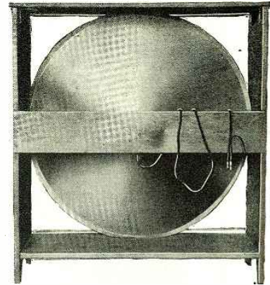
A rear view of the completed cone speaker. The unit is mounted on the wooden cross member.
