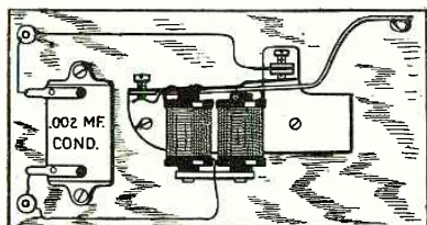
Details of the Vacuum Tube Safety Device.
