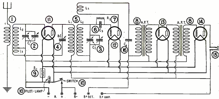
The schematic diagram of the receiver, numbered like the others. Two different, but both very popular methods of obtaining regeneration are employed in the R.F. and detector stages, although three-circuit tuners are used. C-1 and C-2 represent a tandem .0005- \mu f. variable condenser, with separate vernier units, preferably of the S.L.F. type.
