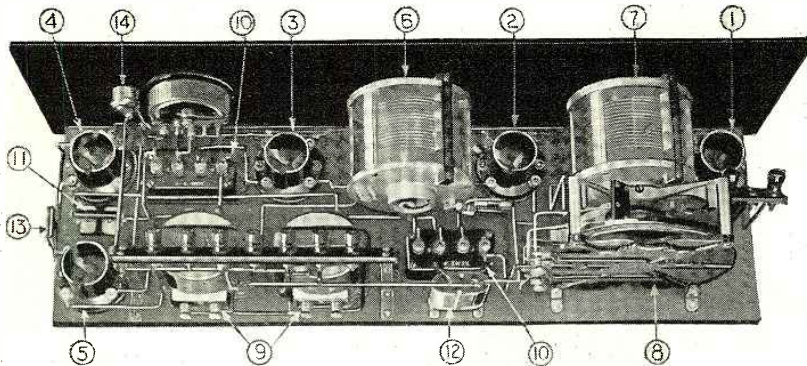
1, 2, and 3 are R.F. tube sockets; 4, detector; 3 and 5, A.F. sockets; 6 and 7, tuning condensers; 8 and 10, R.F. transformers; 9, A.F. transformers; 11, grid leak and condenser; 12 and 13, by-pass condenser; 14, filament switch.
