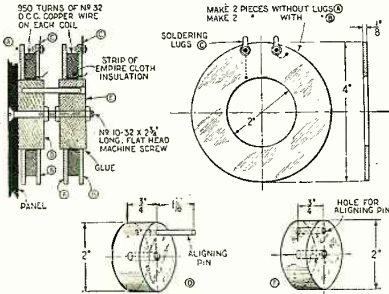
Circuit No. 2176-A.—The design and constructional data including all necessary dimensions of an intermediate frequency transformer, air core type, having an amplification peak at 10,000 meters.
