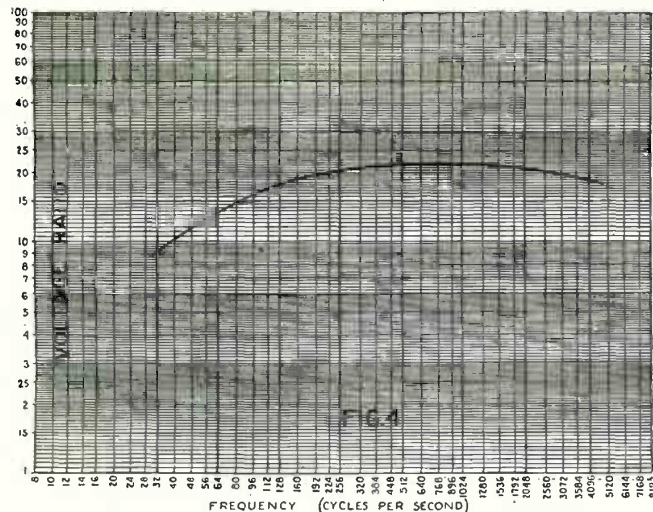
Here is an example of the manner in which Mr. Harris says that amplifier characteristics should be plotted. A special "logarithmic scale" is used for the horizontal distances, giving each octave an equal space—that between the heavy vertical lines. The vertical scale, that of voltage step-up, is logarithmic also, but on a different scale based on a study of the sensation of loudness, as explained elsewhere. The resulting curve shows most intelligently the effect on the ear of the tones emerging from the phones or speaker when the A.F. currents of the frequencies causing them have passed through this amplifier.
