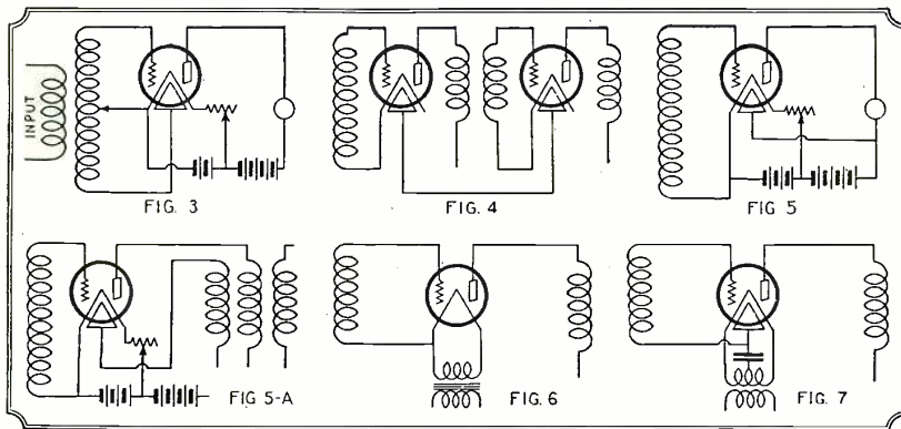
Circuits wherein the "Quadrotron" is utilized. Fig. 3 represents a form of push-pull amplifier. Figs. 4, 5 and 5-A depict two methods of equalizing tube capacity by means of the fourth element. This "control grid" is of particular advantage in a circuit using filtered A.C. for heating the filaments of the tubes. The circuit is outlined in Fig. 7.
