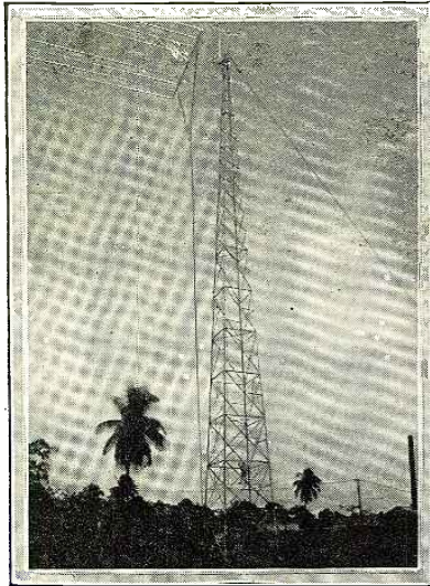
A typical steel construction radio tower. All members are galvanized to protect them from deterioration through climatic influences. Photo courtesy of Milliken Brothers Mfg. Co.
