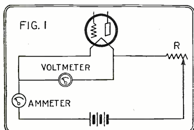
FIG. 1 Meter connections for ascertaining condition of the filament.
