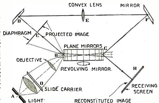
Fig. 1. This diagram is fully explained in the text. The cylinder is covered with plane mirrors, revolving downward on the side toward the lantern. One ray at a time, from 1/25,000 of the area of the image, passes through the opening in C. The fixed mirrors D and F send it back to the mirror G, opposite B on the cylinder, and it is finally reflected against H in a position corresponding exactly to the portion from which it was first taken. The effect of continuous vision is produced.
