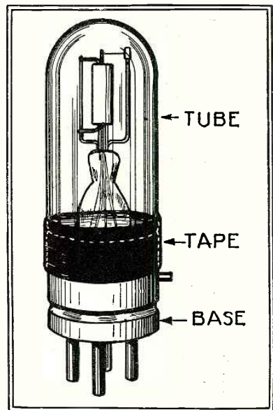
A tube that has become loosened from its base can be repaired by winding friction tape around the section where the tube and base meet.
