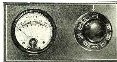
The rotary switch on the right designates the circuit whose voltage is indicated on the meter. Photo courtesy Weston Elec. Instrument Corp.
