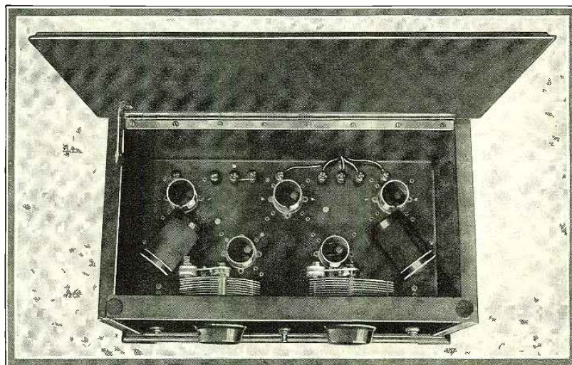
The ample space allowed in this five-tube receiver for the various instruments. is made possible by the use of a sub-panel. Photos courtesy of De Witt La France Co.
