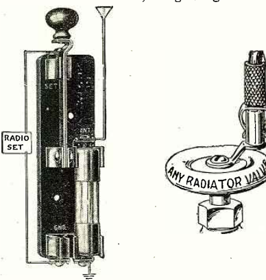
Left: A combination lightning switch and lightning arrester which can be mounted on the frame of a window.
