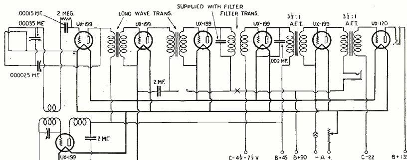
Although there are but two stages of intermediate-frequency amplification, this "super-het" gives remarkable volume because of the audio amplifiers. Dry cell tubes may be used in this receiver for transportation; and storage battery tubes (with a 200,000-ohm variable resistance at X) when it is set up in a more permanent location.
