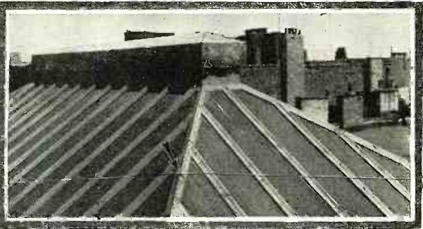
Above: As an aerial this is a good ground. It will be noted that the wire touches the metal framework of the skylight. In consequence very little current reaches the set. Left: This man's aerial was too long so he shortened it by inserting an insulator as indicated by the arrow. Good, but the lead-in should have been taken off at the insulator eye, to relieve the strain on the wire.
