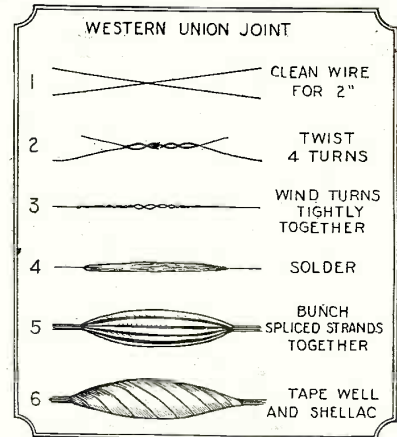
Details in the making of a "Western Union joint." If it is possible, make all your connections this way.
