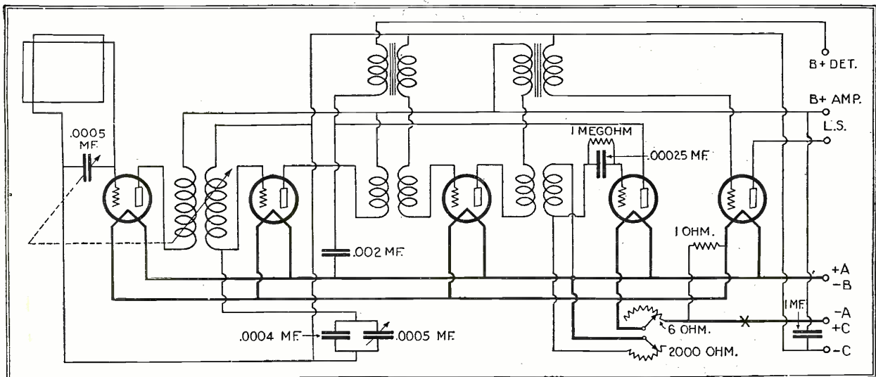
This five-tube reflex receiver combines the best features of tuned and aperiodic transformer coupling, as well as reflex.
