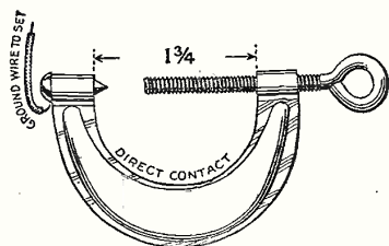
A unique type of ground clamp which, though it has not the surface contact of other types, insures a perfect contact by nature of its pointed stud which will bite through rust or paint.
