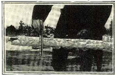
An aerial wire with a four-inch coating of ice. The aerial, having been well installed, and equipped with a safety device, was able to withstand the strain.
