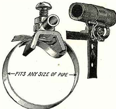
Two types of ground clamps having a large surface contact. Being adjustable, they will fit almost any size of pipe.
