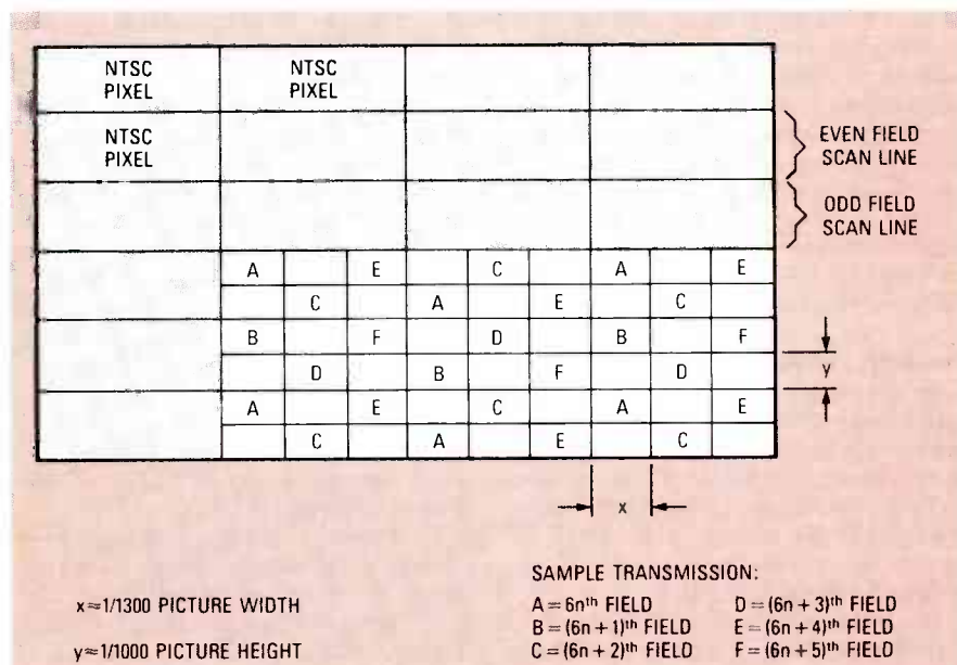
FIG. 4—IN THE DEL RAY HDTV SYSTEM, each NTSC pixel is broken up into six samples for transmission. Picture information is relayed in a sequence of six fields.
