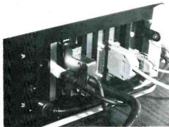
FIG. 5—CONNECTORS IN PLACE AND READY FOR USE. The 37-pin D-connector is a real heavyweight, so be certain that you tighten its mounting screws to ensure reliable operation.
