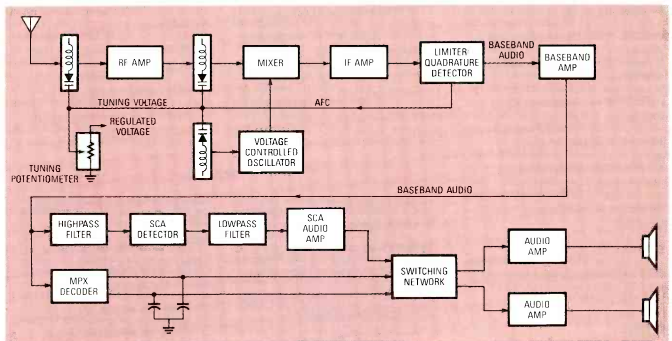
FIG. 1—OUR SCA RECEIVER is shown here in block diagram form.
