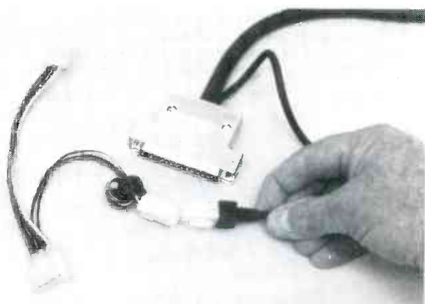
FIG. 1—THE CABLE FROM THE 3 1/2-inch drive has its own power connection take-off that matches the miniature power socket on the supplied Y-adaptor. The ring through which the adapter's power wire loops is a toroid choke that help suppress RFI.
