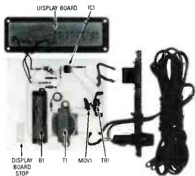
FIG. 5—THE COMPLETE TIMER CIRCUIT appears as shown here. Trim the PC board so that it fits into the case properly, and insert a sheet of insulating paper between the board and the bottom of the case.
