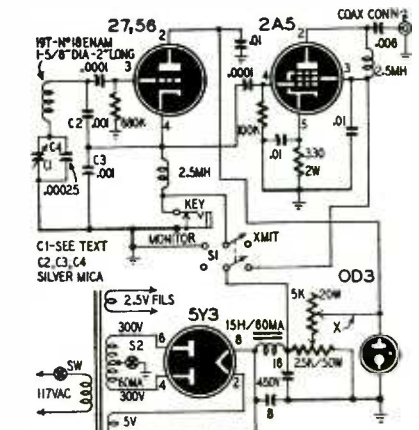
Fig. 3—Circuit of the final model of the v.f.o. complete with power supply.
