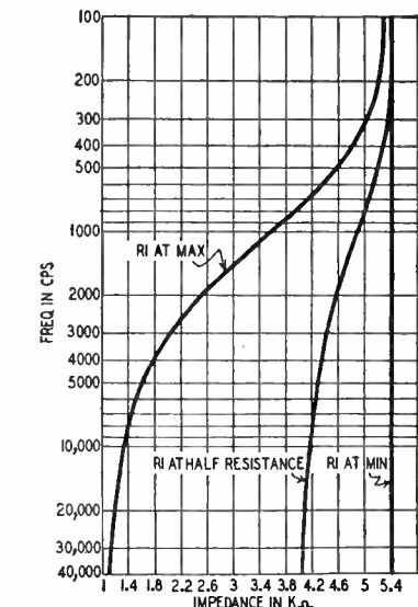
Fig. 2—Impedance variation of treble circuit with bass control at minimum.
