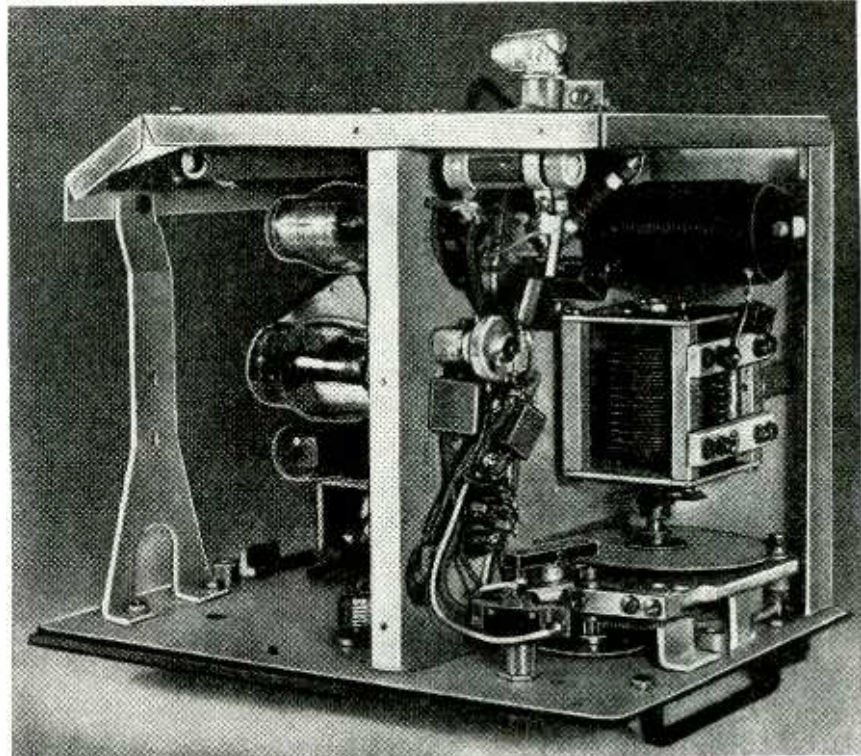
Photo C—Rear view of the larger model showing the tuning section. The power supply is in the compartment at left, the tuning components are at the right.
