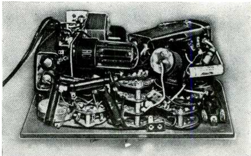
A back-of-the-panel photo. Many of the components are mounted on the switches.
