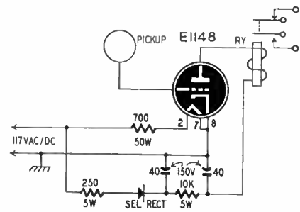
Fig. 1—Electrostatic switch circuit.
