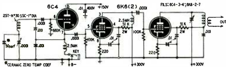
Fig. 2—This circuit, the prototype of the final model, gave excellent results.
