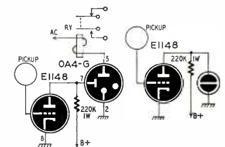
Fig. 2, left—Circuit for 25-ma relay. Fig. 3, right—Hookup for indicator use.
