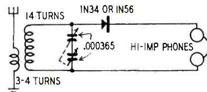
Fig. 1—Though it tunes broadly, this conventional circuit works quite well.
