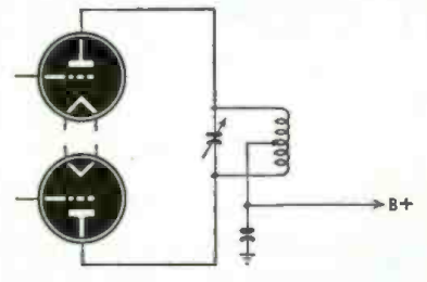
Fig. 4—A standard push-pull amplifier.
