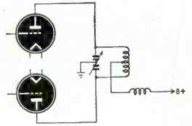
Fig. 5—Push-pull and split-stator unit.
