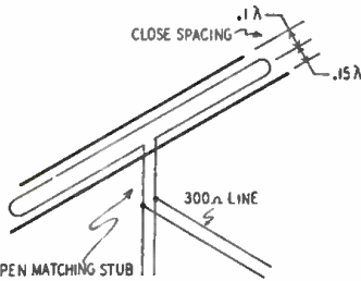
Fig. 2—Standard parasitic element spacing.
