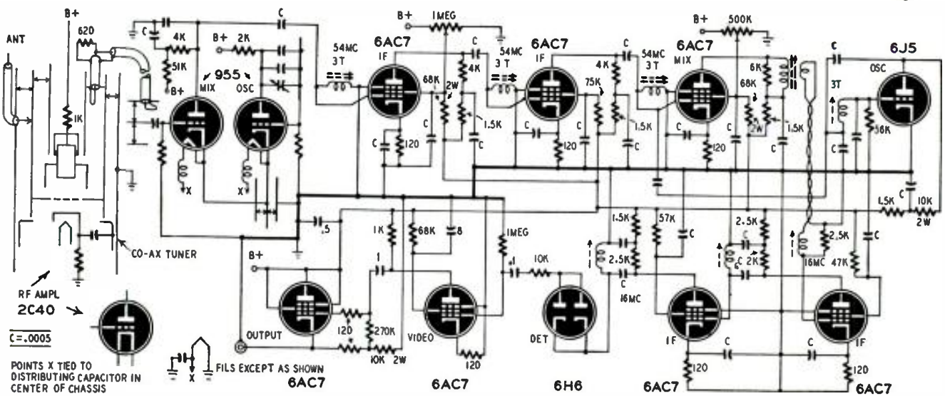
Fig. 6—A surplus ASB-6 radar receiver is used by most viewers to convert the 600-mc signal of W3XB8 to one suitable for the TV receiver.
