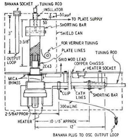
Fig. 3—A side elevation of the final stage. own way, both of the systems mentioned in addition to a few variations are in use.
