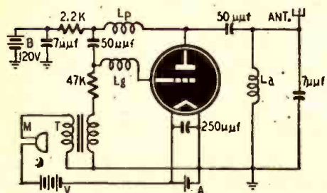
Fig. 2—Schematic of flat-plate transmitter.
