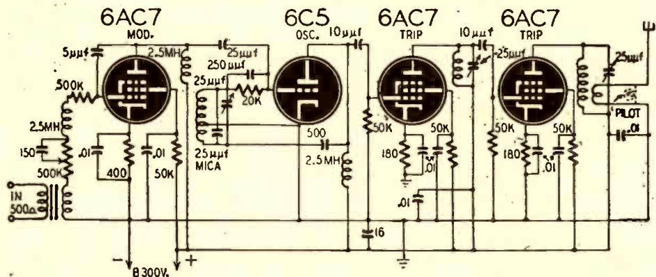
Fig. 1—The FM transmitter. This 4-tube job might serve as a model for amateur exciter.
