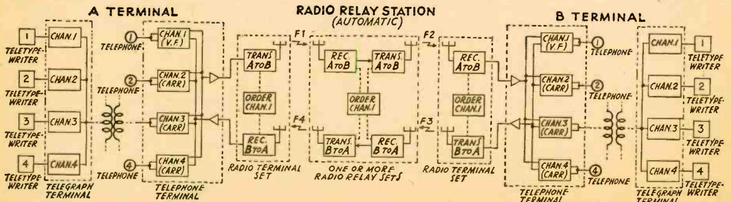
Fig. 1—A typical army network, in which wire lines, carrier channels and VHF radio circuits are combined in a large multi-channel system.
