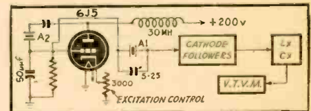
Fig. 2—Push-button Comparator. Six crystals are switched into each position shown.
