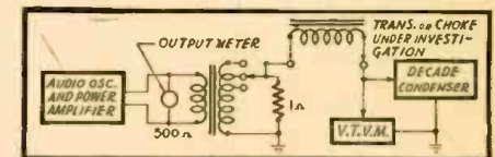
Fig. 3—A Comparator for audio frequencies.
