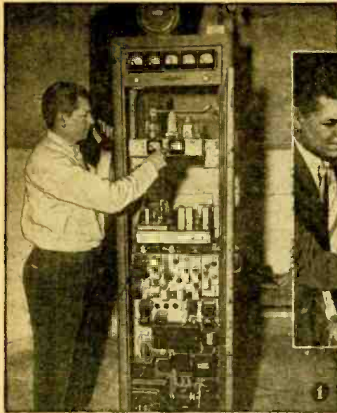
Photo 1—The 250-watt 118.55 Mc. Motorola transmitter. Lt. Ben Denby, at left of rack is using handset for monitoring during adjustment.
