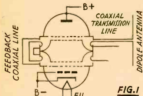
FIG. 1 BASIC KLYSTRON OSCILLATOR CIRCUIT
