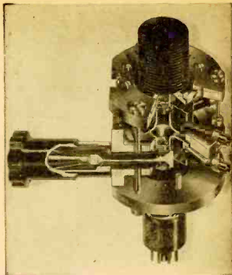
Courtesy Sperry Gyroscope Co. Cut-away shows Klystron's internal construction, co-ax leads and vernier tuning screw.
