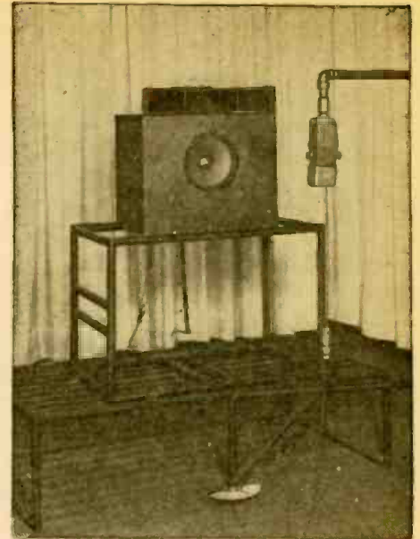
Speaker calibration. Note how microphone is swung to measure angular sound distribution.
