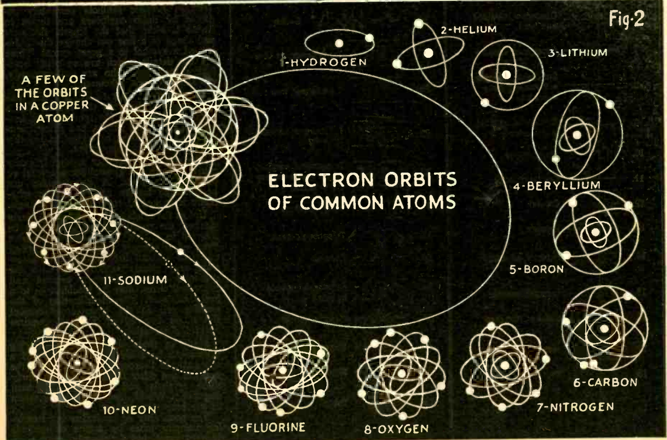
Fig. 2—Electron shells of atoms from hydrogen to sodium, also copper. The long orbits are the "wild" electrons of copper and sodium. RADIO-CRAFT for APRIL, 1944
