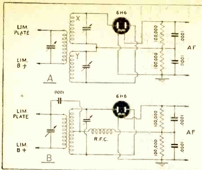
Fig. 1, left—Two fundamental FM discriminator circuits. The system at B is the one now commonly used in commercial FM receivers. Fig. 2, right—How the two separate AM detectors of Fig. 1-A can be made to operate as a discriminator for detecting FM signals.
