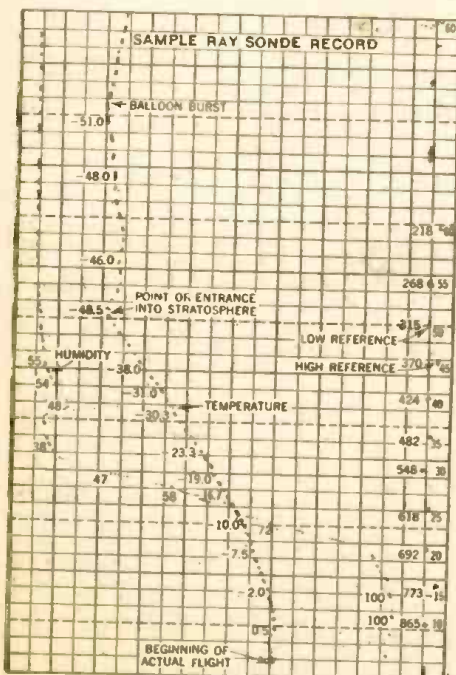
Chart above is an actual record of a flight. Marks along the right edge are made by the reference frequency, described in the text.
