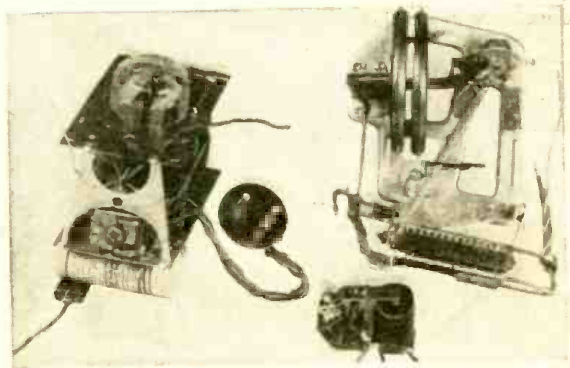
Fig. 3, right—A view of the transmitter and the pressure unit which operates it.
