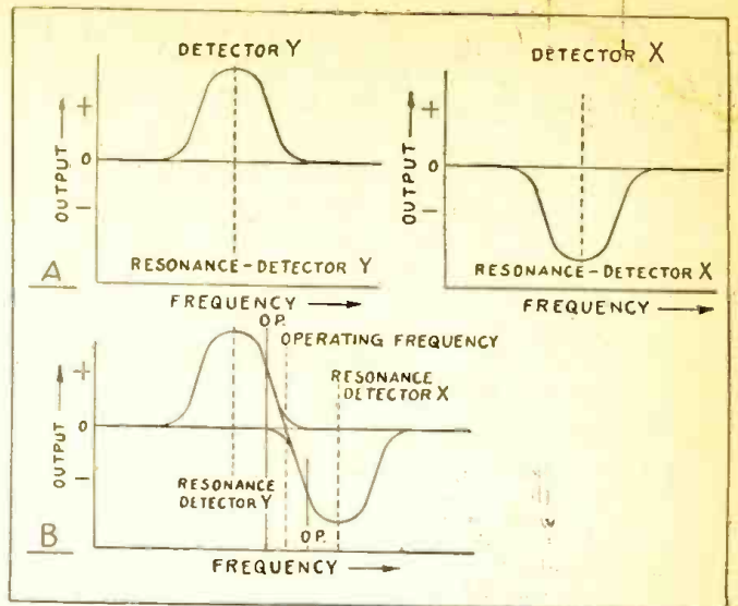
Fig. 1, left—Two fundamental FM discriminator circuits. The system at B is the one now commonly used in commercial FM receivers. Fig. 2, right—How the two separate AM detectors of Fig. 1-A can be made to operate as a discriminator for detecting FM signals.
