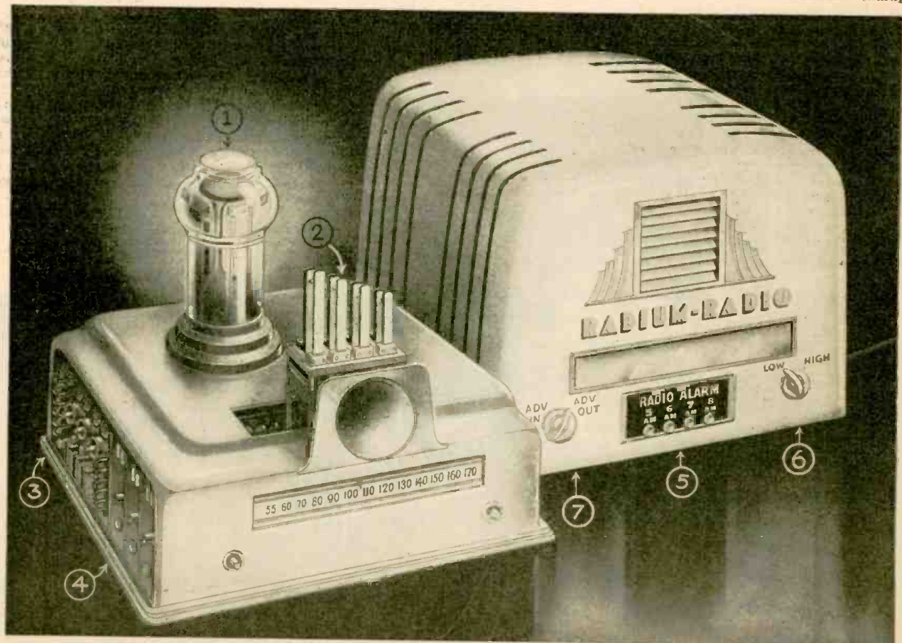
A photograph of the perfected Radium-Radio set. (1) The new radium currentless radio tube. (2) Tuned reeds to operate the radio alarm. (3) Electronic memory control to eliminate ad plugs. (4) Iron dust core tuning inductance. (5) Radio alarm. (6) Low and high volume knob. (7) Switch to cut in or cut out objectionable radio advertising plugs.
