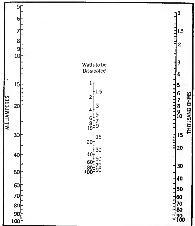
With this chart one may determine the relationship between current, resistance, and wattage when two factors are known. A straight edge is laid across the two known factors and extended, if necessary, to include the third. The chart was prepared by R. C. Hitchcock.
