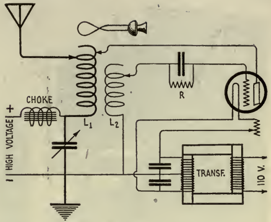
FIG. 1 The fundamental British circuit
