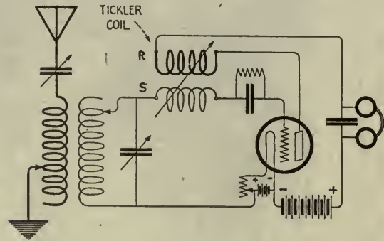
FIG. 2 A non-regenerative circuit made regenerative by the inclusion of a tickler coil. In the variometer set, the rotor and stator, R and S would be changed for individual variometers, well separated
