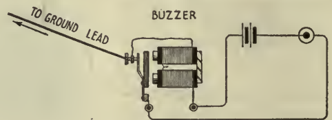
HOW TO CONNECT A BUZZER
