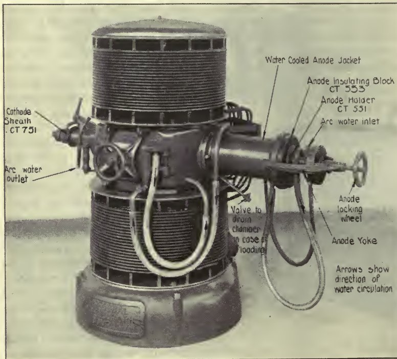
A 30-KW ARC CONVERTER
