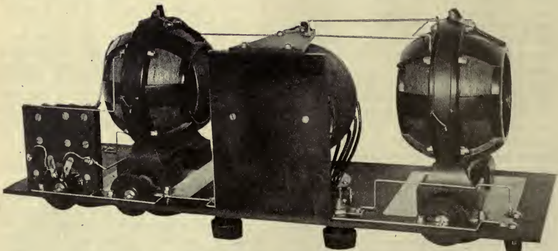
A WELL-DESIGNED 3-CIRCUIT TUNER
