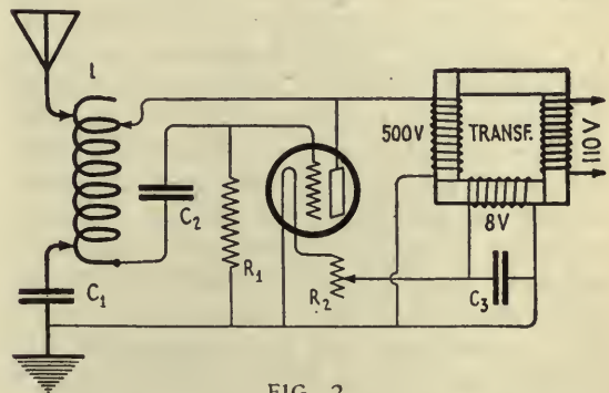
FIG. 2 Circuit of the half-wave self-rectified set which has been made for less than seventeen dollars and which has a reliable range of twenty-five miles
