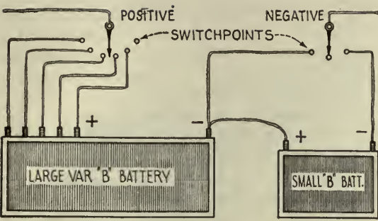
FIG. 7 Method of connecting B batteries
