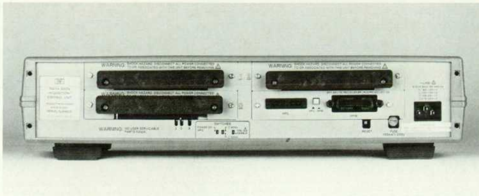
Fig. 2. Back panel of the 3421A. The three slots can be used to insert 10-channel latching-relay cards, digital I/O cards, or breadboard cards customized by the user for specific applications. This 3421A also has the optional HP-IB interface.
