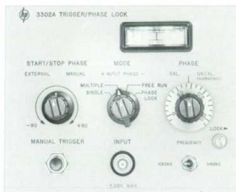
Fig. 1. Trigger/Phase-Lock Plug-in increases range of capabilities of hp -Model 3300A Function Generator. Plug-in enables generation of single cycles of output waveform or bursts of cycles, or it phase-locks Function Generator to external signal.
