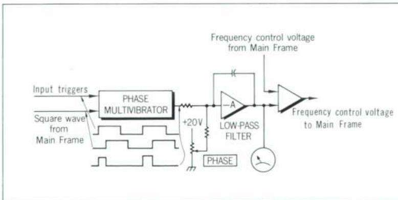
Fig. 3. Block diagram of Trigger/Phase Lock Plug-in 'Phase Lock' mode.
