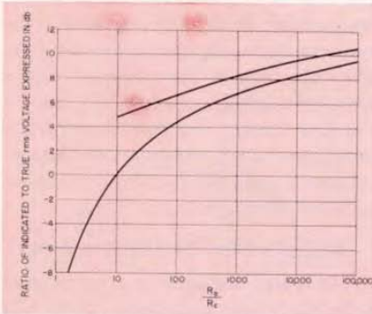
Figure 5. Previously published data of the response of a peak voltmeter to random noise (upper curve, reference (5); lower curve, reference (6)).
