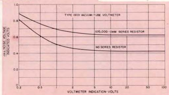
Figure 9. Correction for Type 1803 Vacuum-Tube Voltmeter indication to obtain r-m-s value of random noise.
