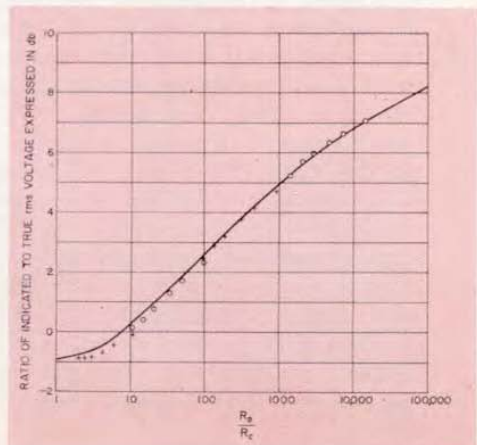
Figure 6. Response of peak voltmeter to random noise. Curve is calculated, points are experimental data.
