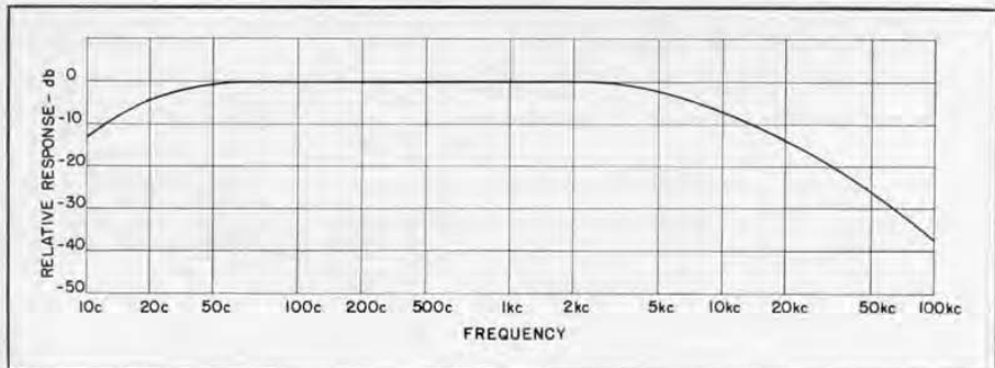
Figure 2. Frequency response characteristic of the amplifier.
