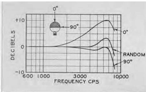
FIGURE 16. Typical curves showing the response of average TYPE 759-B Sound-Level Meters to sounds reaching the microphone at various angles. The random response which corresponds with the A.S.A. Standards represents the over-all characteristic, assuming that the sound arrives equally at all angles in a vertical plane.
