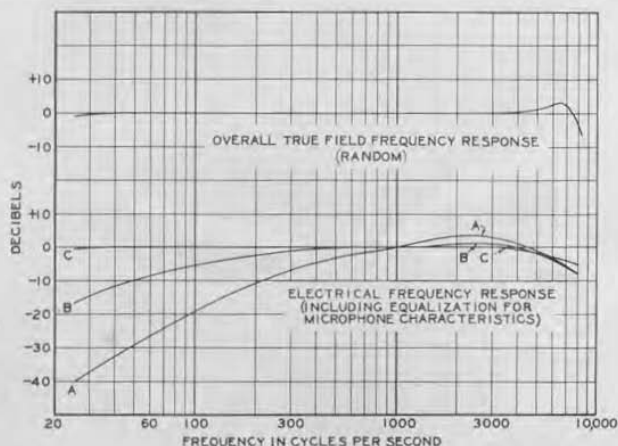
FIGURE 15. Typical average acoustical and electrical calibration curves for TYPE 759-B Sound-Level Meter.
