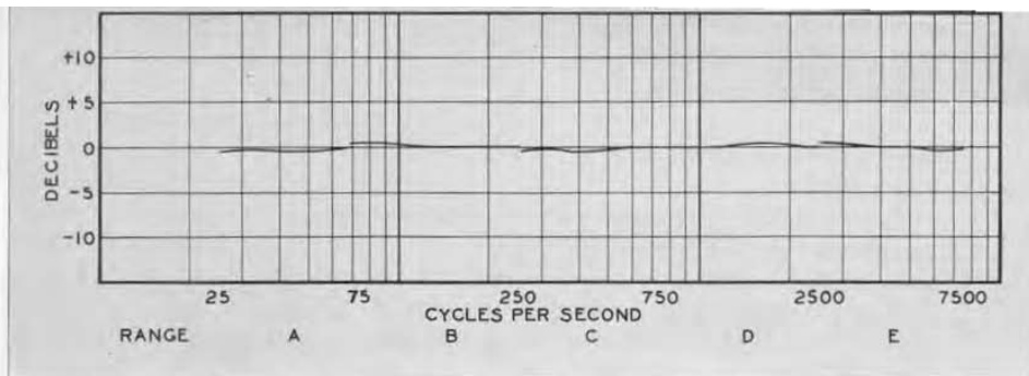
FIGURE 18. Typical response curve of TYPE 760-A Sound Analyzer. A calibration of this type may be made easily by anyone having a satisfactory audio-frequency oscillator and vacuum-tube voltmeter or other indicating device. All that is necessary is to maintain a constant voltage at the input of the analyzer, tune the oscillator to various frequencies throughout the range and at each frequency tune the analyzer to exact resonance and read the indicating meter.
