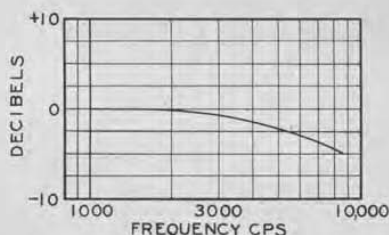
FIGURE 17. According to the A.S.A. Standards, a sound-level meter is calibrated for random response. Under conditions where all of the sound reaches the microphone from the horizontal (90°) direction the above corrections may be applied to the random microphone calibration in order to obtain better accuracy at high frequencies.
