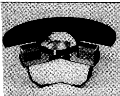
Cross section of the midrange driver.
