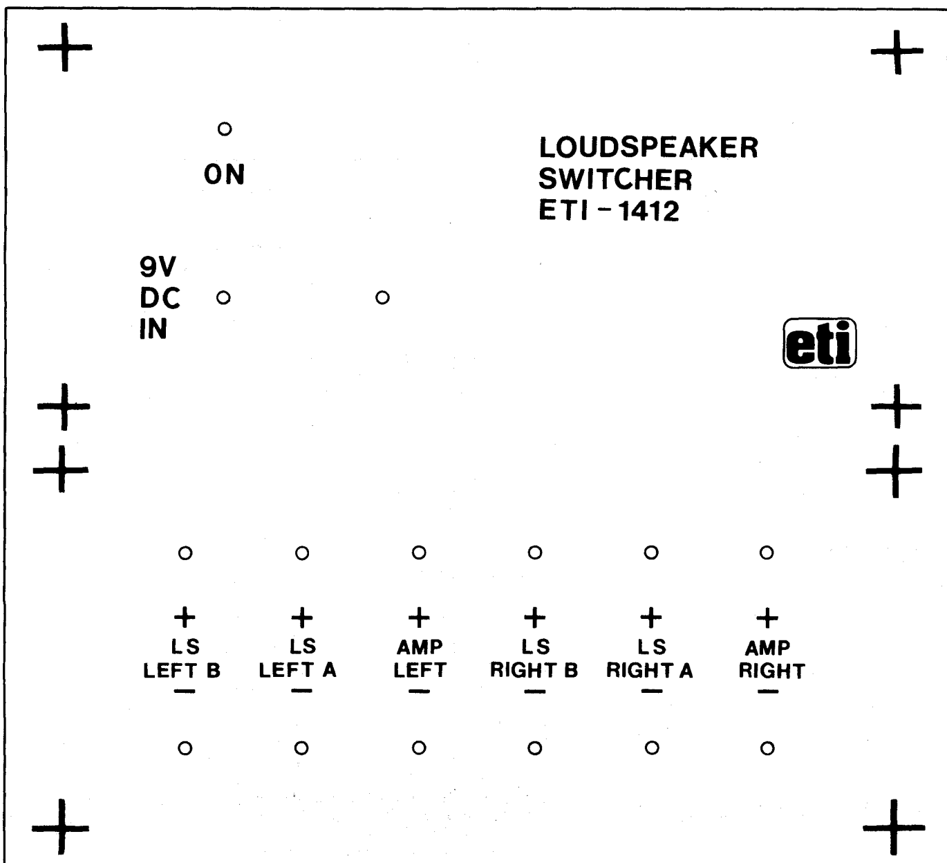
Sockets on the rear panel.
