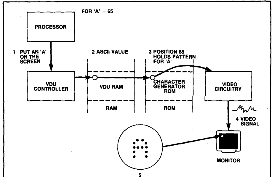
Figure 1. Block diagram showing how a character gets onto the screen.
