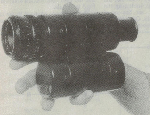
Fig.2: This shot shows a construction virtually identical to that described in September 1990. The difference is the size! Compare it to that shown in the September article. This is not the case being described here, as the new case is even simpler and smaller.
