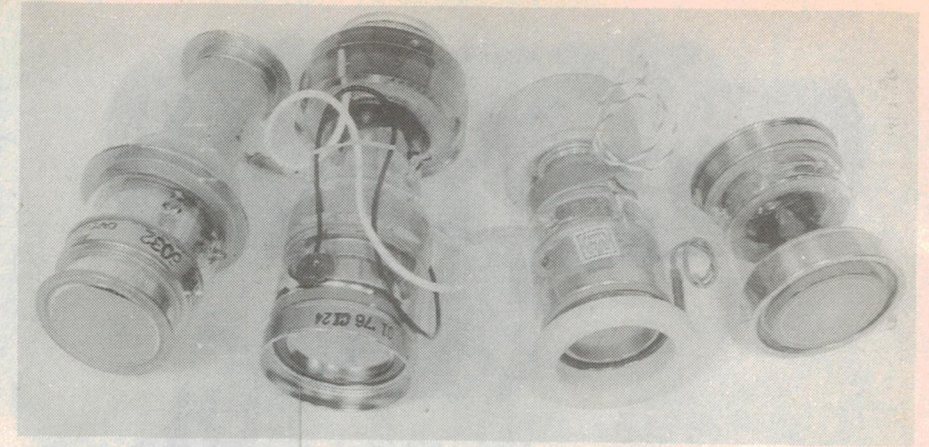
Fig.3: There are various IR tubes available, as shown in this photograph. The BWB448 tube, described in this article is shown in the centre. The 6032 and 6032A tubes on the left can also be used. The Philips fibre-optic coupled tube on the right has a greater sensitivity and doesn't need a focus voltage.
