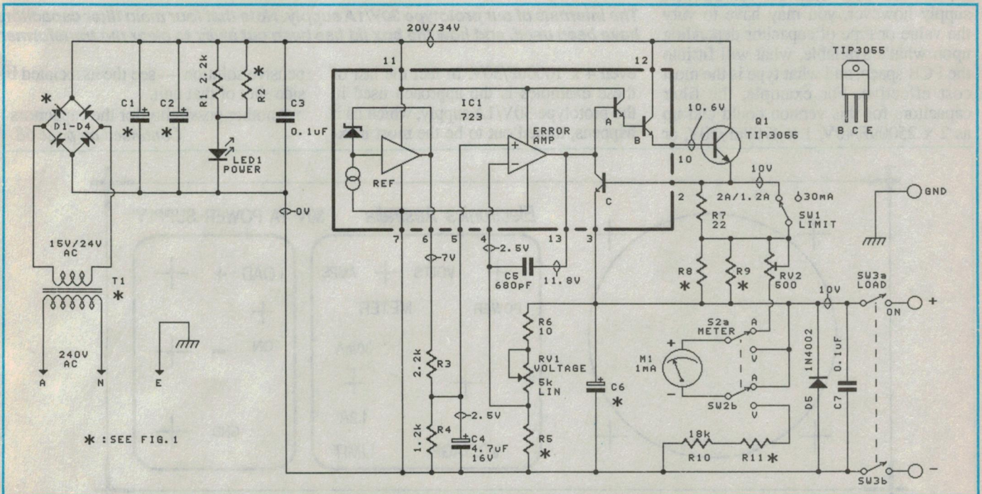
This is the schematic, showing the components that need to be changed. Fig.1 above, gives the components and values for each version of the benchtop power supply.
