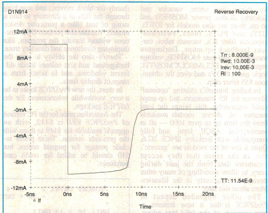
Fig.3: As part of its operation in helping you to produce device modelling data files from manufacturers' data sheets, PSPICE's modelling program PARTS.EXE allows you to plot the performance of the model. Here's an example.
