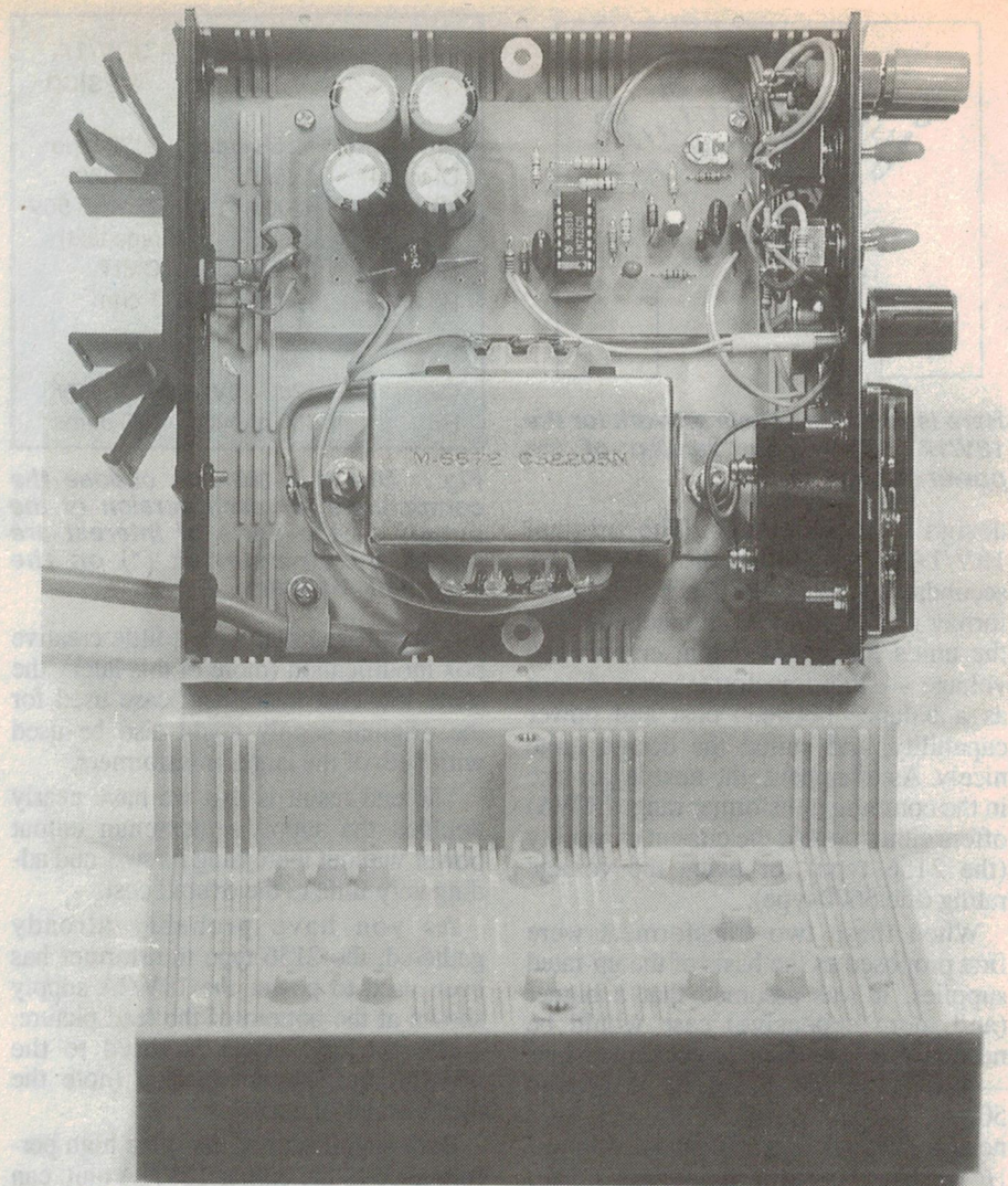
The internals of our prototype 30V/1A supply. Note that four main filter capacitors have been used, and how the box lid has been cut away to clear the transformer.
