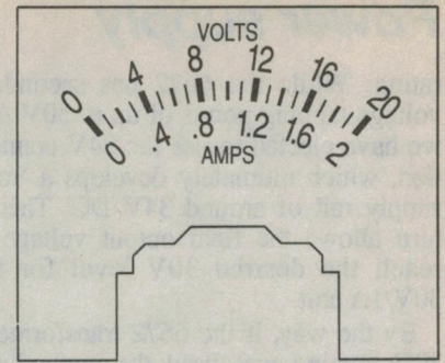
And this is the meter scale artwork for the 18V/2A version of the power supply.
