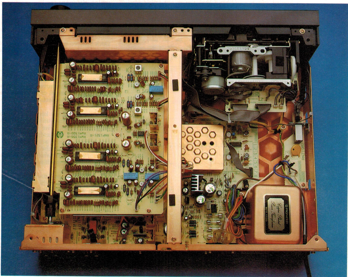
Inside the Pioneer CT-93. Virtually all of the exposed metal work is heavily copper plated, which Pioneer claims reduces stray electrical currents. Visible at upper right is the tape transport, which incorporates a number of dramatic new enhancements. The four large 52 pin ICs visible down the left hand side are presumably involved in the recorder's comprehensive audio processing.
