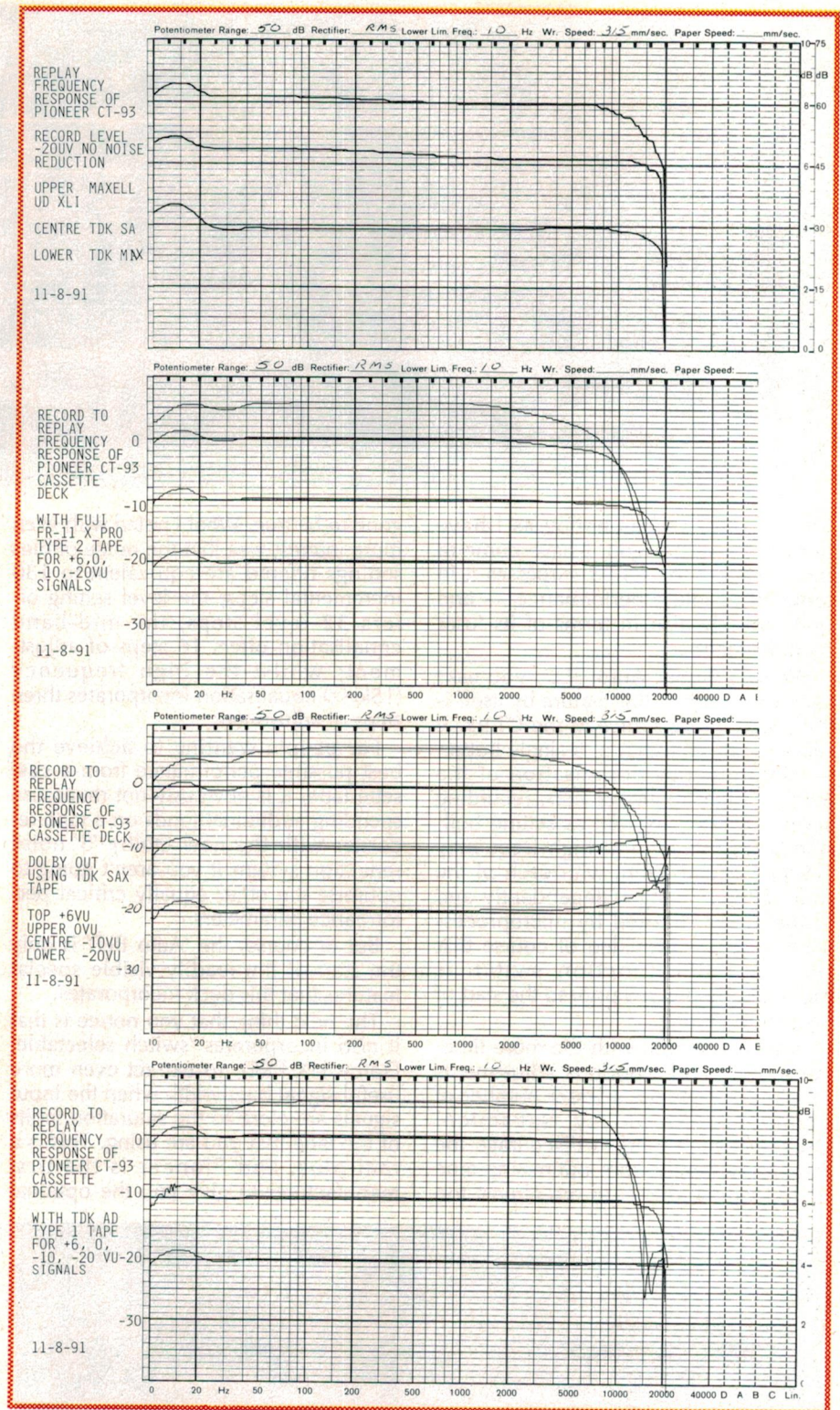
Four of the performance curves for the Pioneer CT-93 deck, as measured by Louis Challis. At top are the replay response curves with three different kinds of tape, while the lower curves show record/replay response curves at different recording levels, for three different tape formulations.
