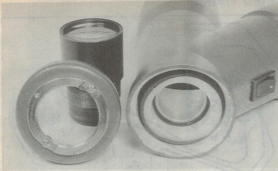
This photo shows the cathode end of the case and details of how the imaging lens is mounted.
