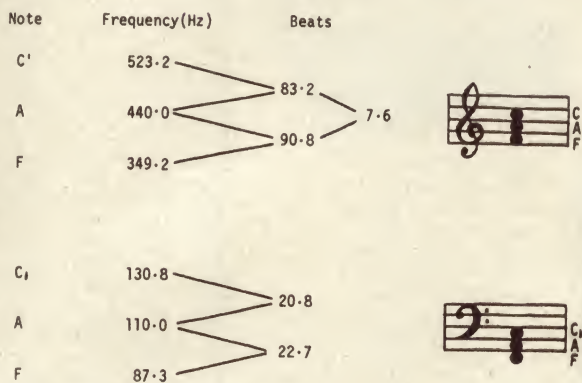
Figure 2. Beats in the major triad.
