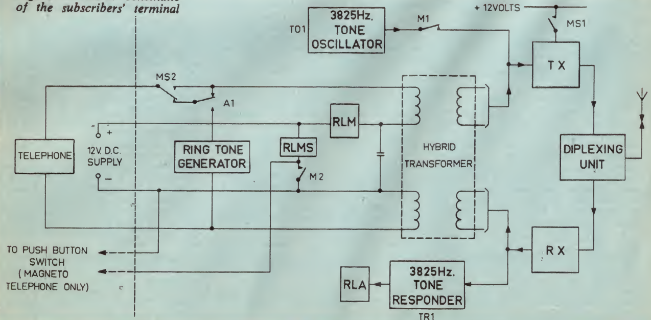
Figure 1. Block schematic of the subscribers' terminal
