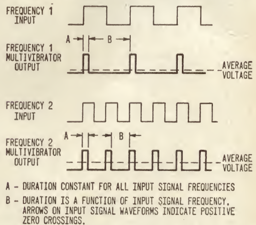
Figure 11. These waveforms are the inputs and MV outputs shown in figure 10.
