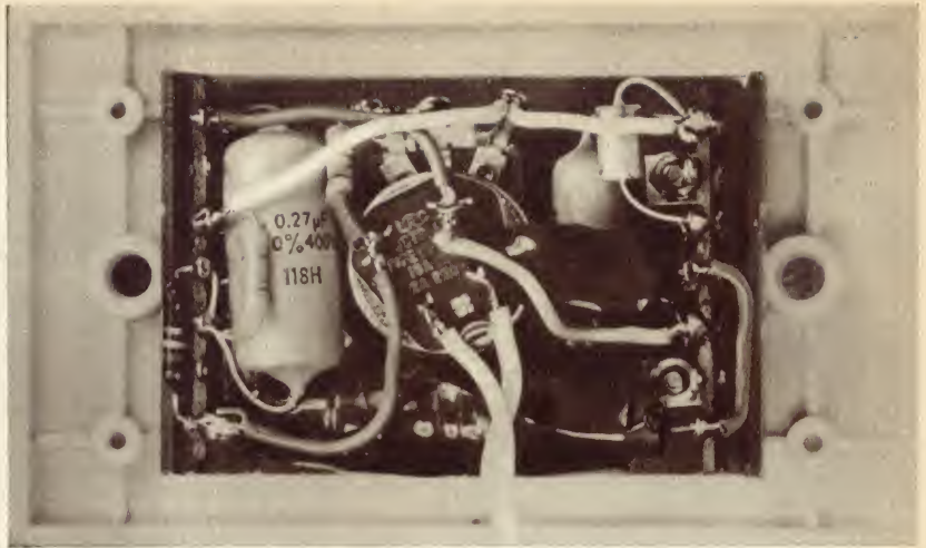
Rear view of the finished unit. The choke is lying horizontally below the pot., the Triac (in plastic tape) is to the right, and the Diac in the top right corner. (See also page 43.)
