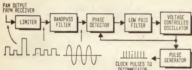
Figure 16. It is important to keep step in telemetry. One way the job is done is with this closed-loop PAM telemetry channel synchronization circuit.
