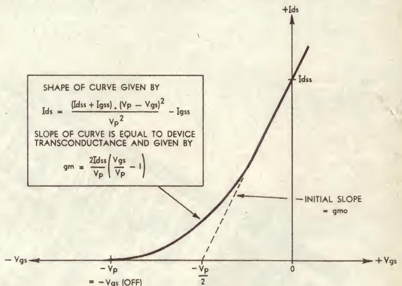
Figure 8.4 N-CHANNEL JFET "STATIC TRANSFER CHARACTERISTIC"
