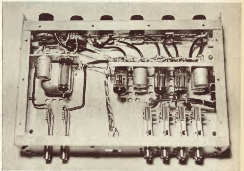
Underside view, showing component arrangement.
