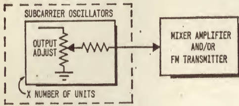
Figure 6. A typical resistor-mixer circuit usually used in FM/FM telemetry systems.
