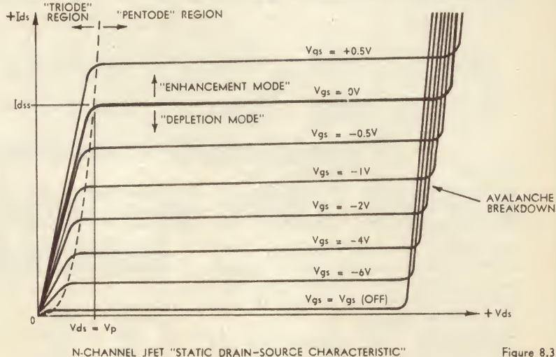
N-CHANNEL JFET "STATIC DRAIN-SOURCE CHARACTERISTIC"
