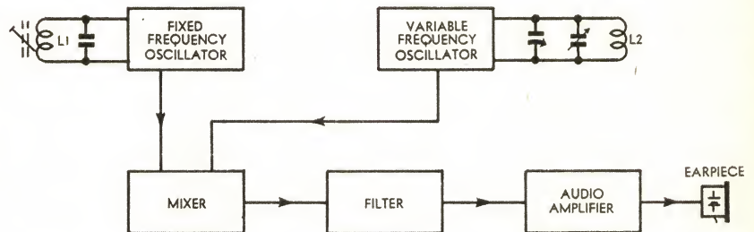
Block schematic for the metal detector. The variable frequency oscillator at right is the search head.
