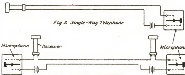
Diagrams for connections for single and duplex telephones.
