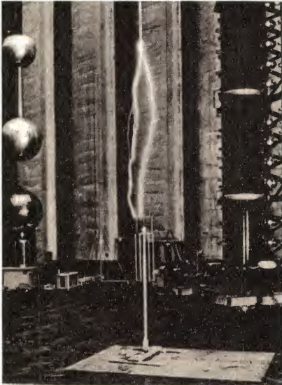
An active receiving antenna, type HA 430/141, undergoes a lightning test in the high-tension house at the Technical University of Munich.
