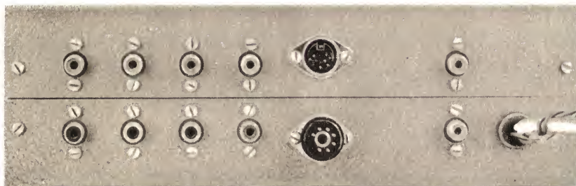
A rear view of the control unit is shown above, with connections being left to right: Radio 2, Radio 1, Disc, Tape, 5-pin DIN socket for tape input/output, 7-pin socket for tuner connections. Two coaxial connectors, on the extreme right, are for high level "flat" output.
