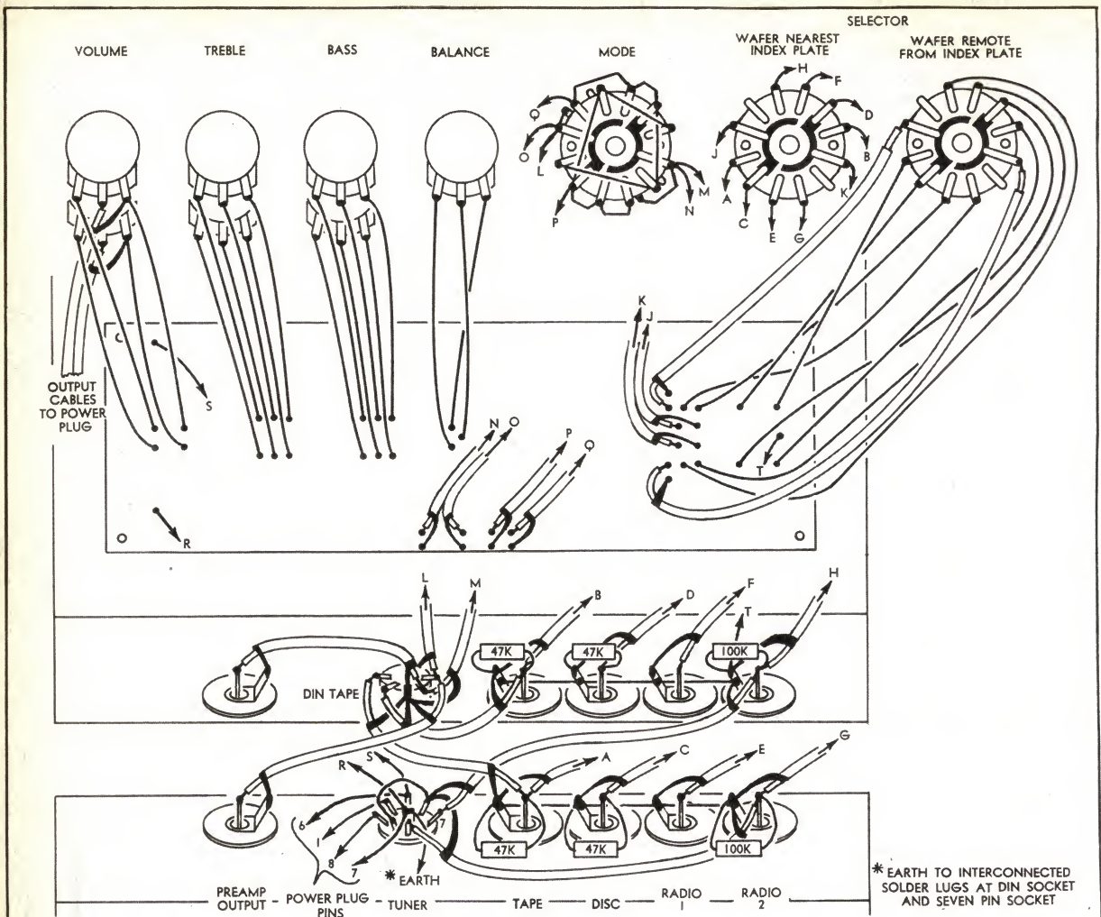
A complete wiring diagram of the control unit with the printed board in position is shown above. Allow plenty of lead length from the wiring board and input sockets to the switches and be careful to make correct connections by systematically following the wiring diagram.
