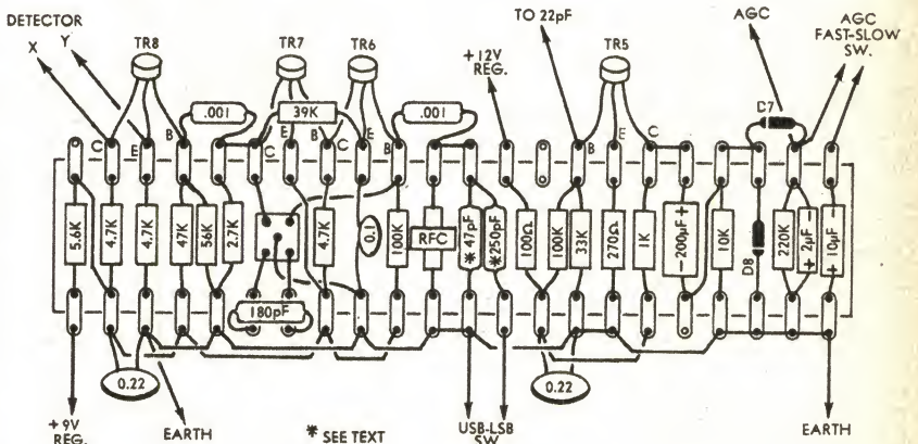
Corresponding with the opposite side of the main assembly, this is the wiring details for the BFO and AGC circuits. As with the IF strip wiring, this should also be checked against the photograph and circuit.
