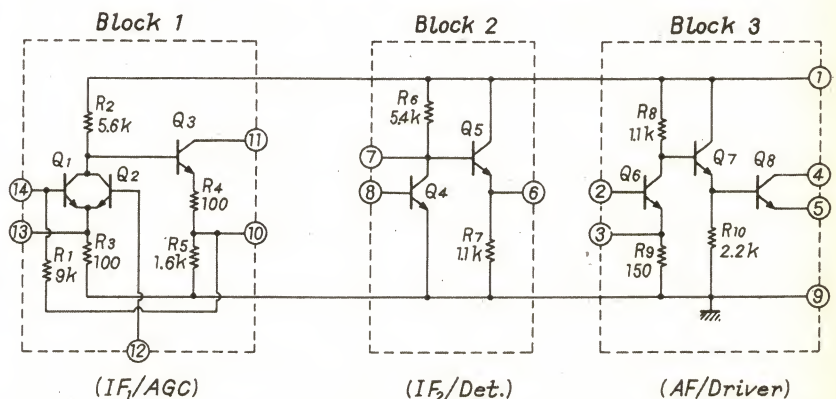
Figure 3. The circuit for the Toshiba TA7049P integrated circuit.
