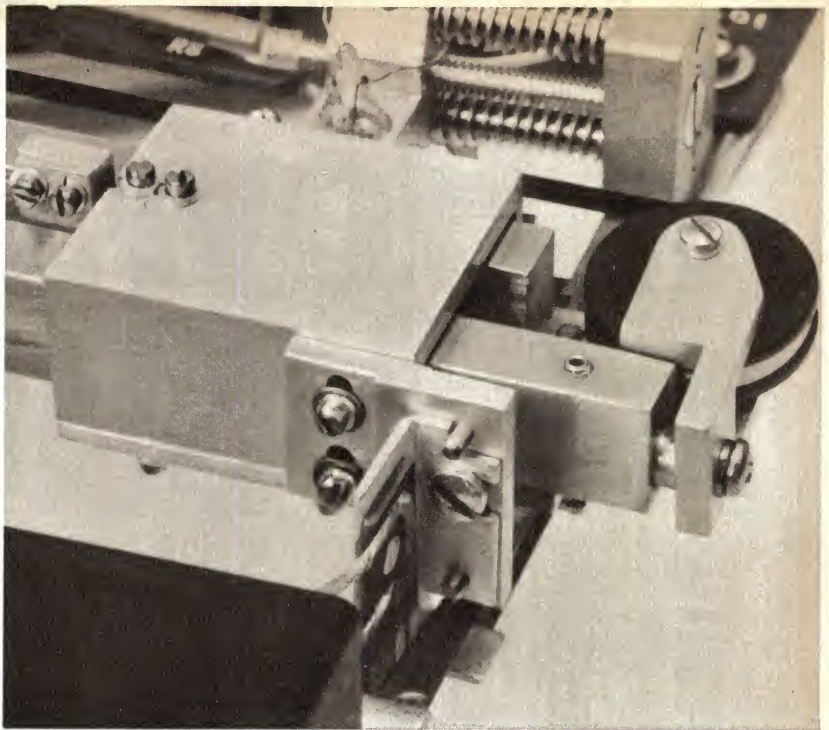
A closeup of the head carriage. The rear of the head assembly proper and the two flexible connectors can be seen in the foreground. The rest of the assembly is beneath the carriage.
