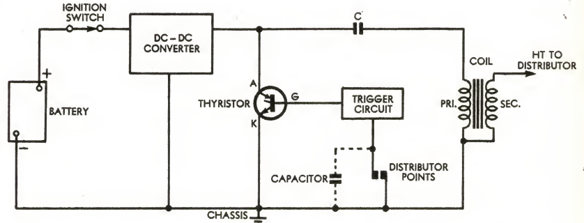
The basic principles of the capacitor discharge system. Energy from the converter is stored in "C" until the points open, then discharges into the coil primary. The capacitor across the points is optional.
