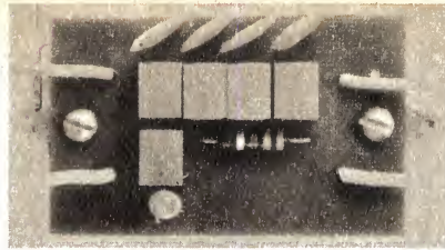
A top view of the filter assembly, showing the simple arrangement of the resonators, top coupling capacitors and 3.3K resistor. The board is shown approximately full size.
