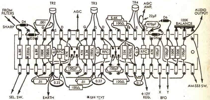
Wiring diagram of the IF strip and detector shows clearly how the components are wired in. This should be studied along with the relevant picture and that part of the circuit.
