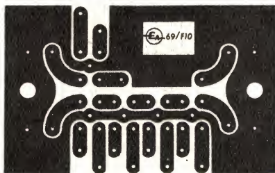
The pattern of the printed wiring board for the filter illustrated on page 81. It is reproduced exact size.
