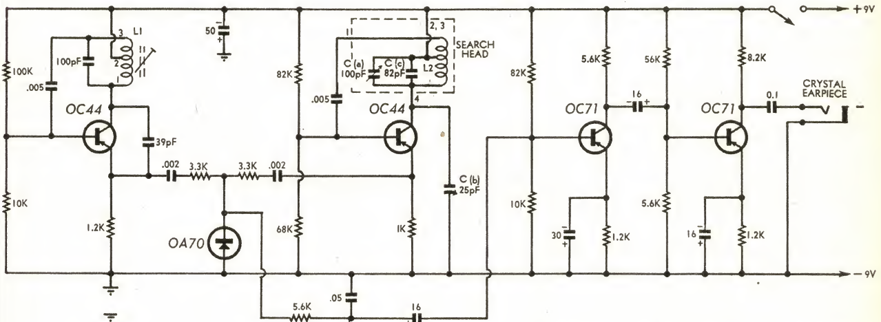
The circuit for the metal detector. All resistors are \frac{1}{2} -watt, 5 or 10 per cent types.
