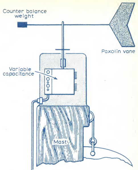
Figure 3. Diagram of the mast-head unit, showing the wind vane and the capacitor unit.
