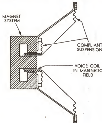
A much simplified diagram of a moving coil loudspeaker. A vital factor is the distance the cone has to travel to produce the required acoustic output. This vitally affects the length of the voice coil and, as a result, the acoustic efficiency.
