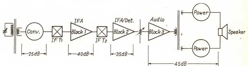
Figure 2. Block diagram of the Toshiba IC-310.
