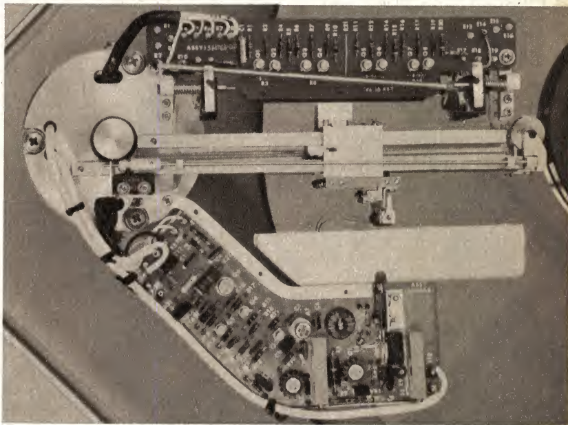
The stepper assembly in position over the disc. The stepper motor pulley is at the left, with an idler pulley at the opposite end of the carriage rails. The head assembly is mounted on the right of and beneath the head carriage.
