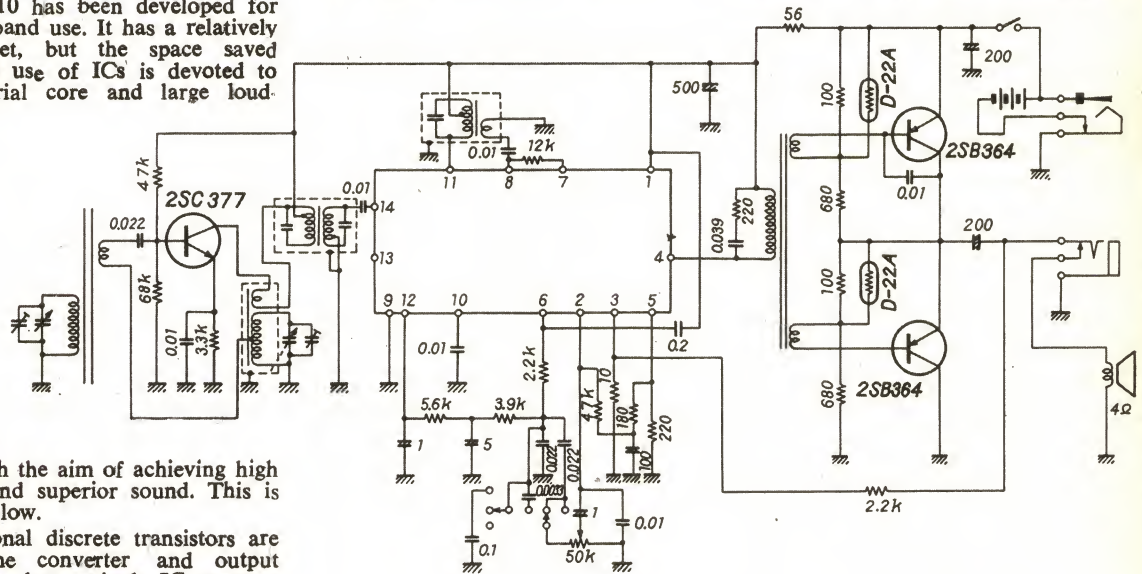
Figure 1. Circuit diagram of the Toshiba IC-310 receiver.
