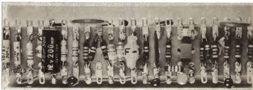
This side of the complete assembly shows the BFO components at the right, with the AGC amplifier, rectifier and time-constants at the left.
