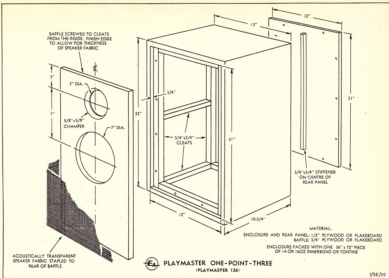
Constructional details of the enclosure for the Playmaster "One-Point-Three" loudspeaker system. Prime requirements for the enclosure are airtightness and rigidity. Note that the baffle should be sprayed black before fitting the grille cloth.
