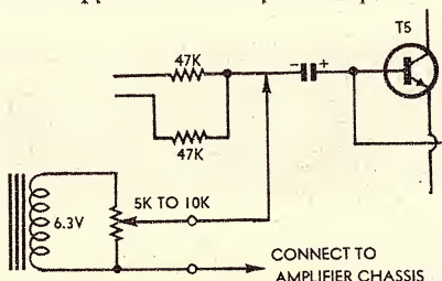
Figure 2. A simple test set-up to determine whether the amplifier is working correctly.
