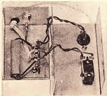
Interior view of the shunt type supply. Note the resistor clamped to the case which functions as a heat sink. The switch is optional.
