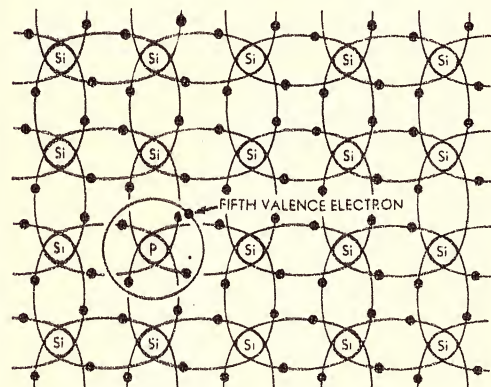
(NUCLEI AND CORE ELECTRONS NOT SHOWN)
