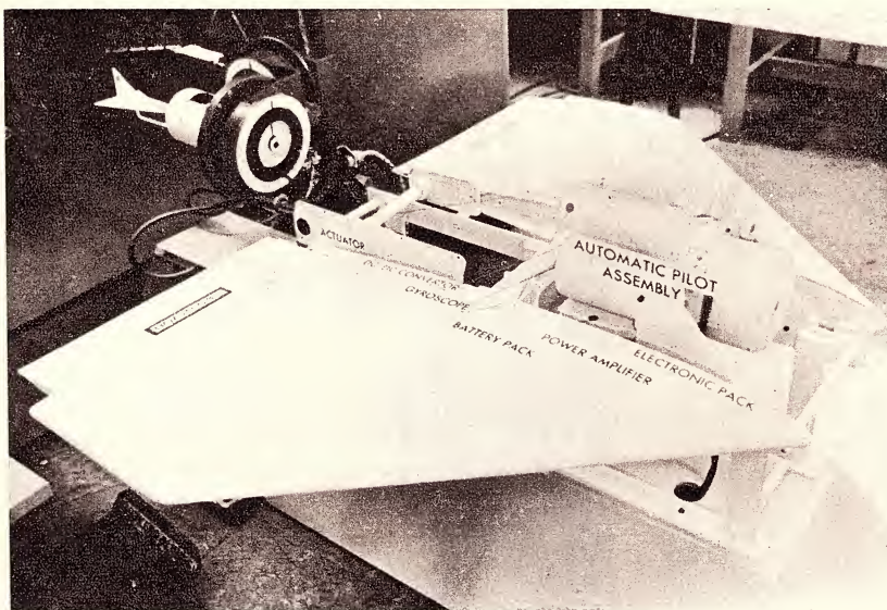
The Aeronautical Research Laboratories, Melbourne, played a major part in the development of Ikara, and featured the system in an exhibit during a series of open days held at the Laboratories recently. Above: The fuselage section in its transporting trolley with the firing sequence equipment (rack at left) and the control system test equipment. Left: The wing section was coded to show the disposition of parts, and visitors were able to operate the controls from an associated panel.
