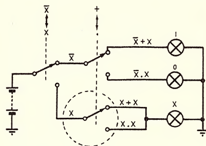
Figure 1. A circuit to demonstrate the simplification of simple expressions using multi-pole rotary switches.
