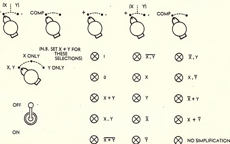
The panel layout of the device. The main function switches perform either AND/OR or COMPLEMENT/NO COMPLEMENT functions, as indicated.
