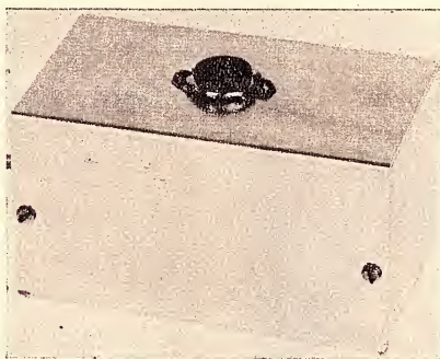
The complete series power supply. The four pin outlet socket also completes the input circuit via a shorting link in the matching plug.
