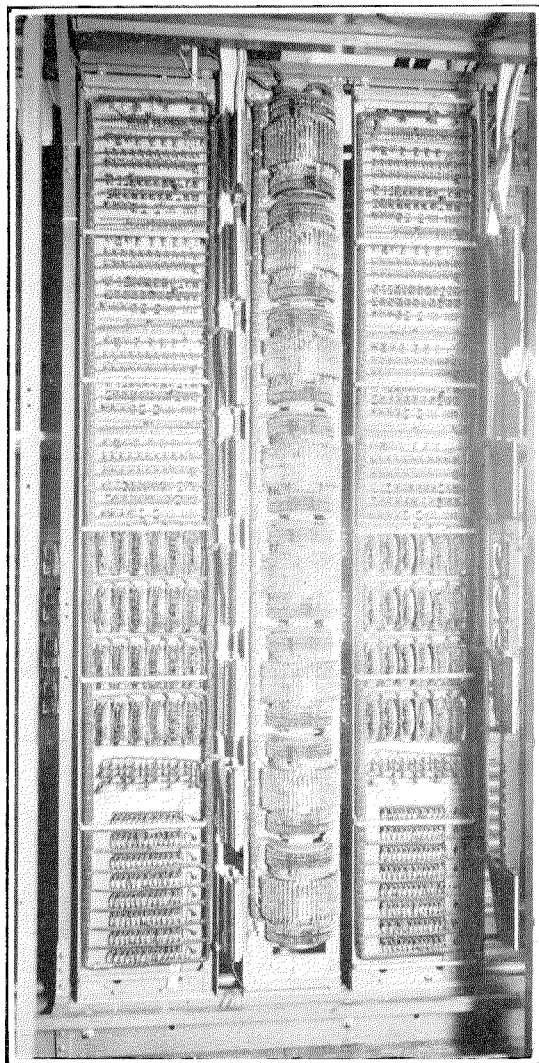
Rear View of Two Register Bays; and, in Between, the Rear View of the Translator Switch Bay, Including the Semi-Circular Terminal Strip. With each register is associated two translator switches and between them is a distributing strip by means of which the office prefix and junction routing may be varied at will.
