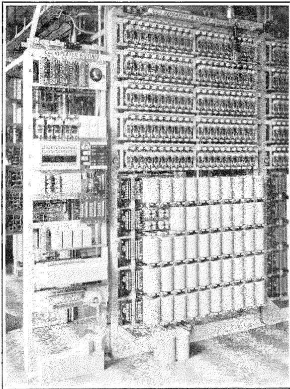
Figure 19—CCI Repeater Routiner.
