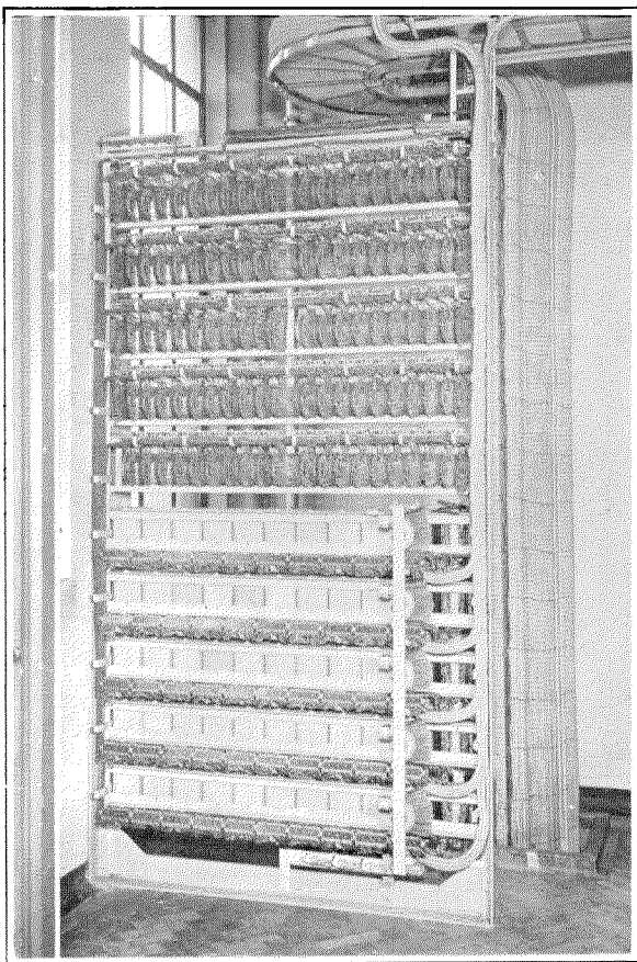
Figure 15—CCI Repeater and Coder Finder Rack—Rear View.
