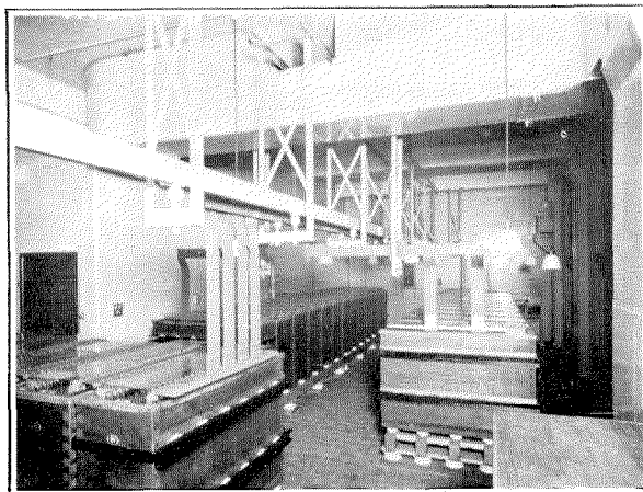
Figure 25—Battery Room.
