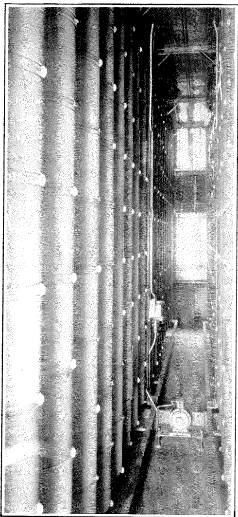
Rear View of Selector and Finder Bays Showing the Manner of Protecting the Rear of All Bays by Sheet Iron Covers, Thereby Guarding the Cable and Wiring Against Mechanical Injury, Dust, etc. The covers also serve to localize any fire which may start in the cabling and wiring.
