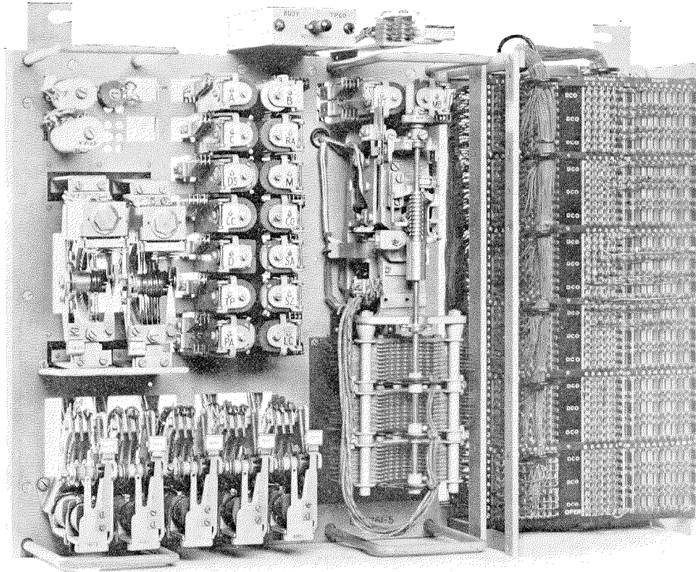
Figure 5—Register-Translator.
