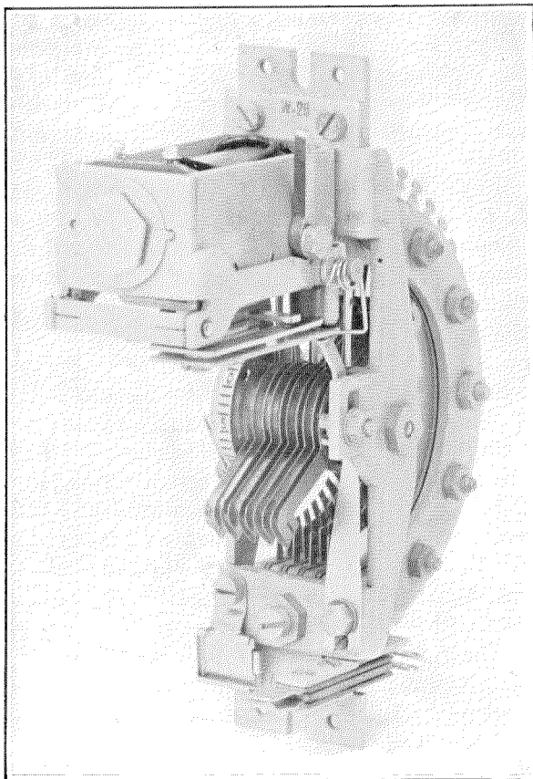
Figure 3—Subscriber's Line Switch.
