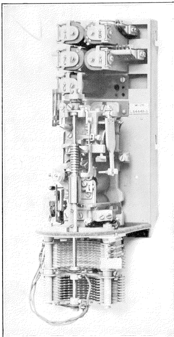
Figure 4—Group Selector.
