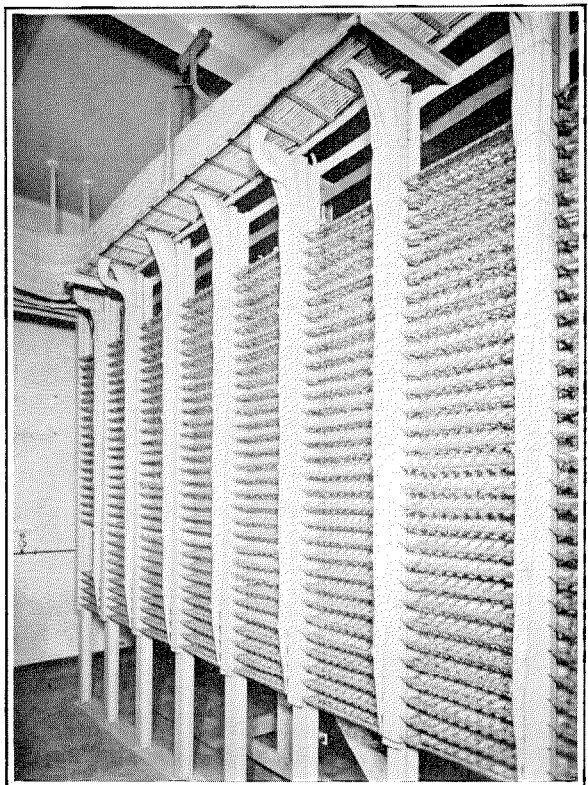
Figure 18—Subscribers' Meter Rack—Rear View.
