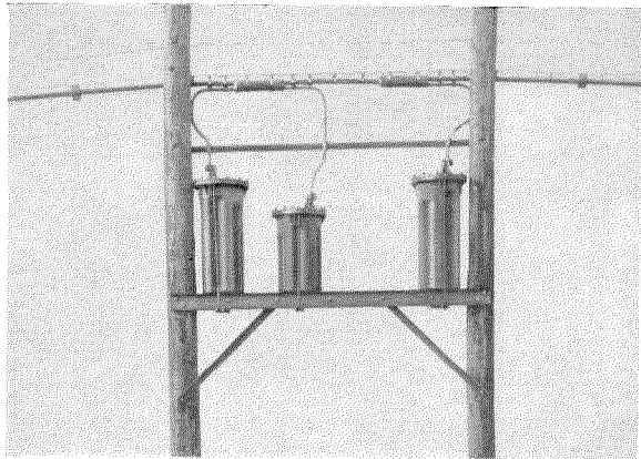
Figure 12—Installation of Aerial Toll Cable Loading on 4-casc "H" Fixture
