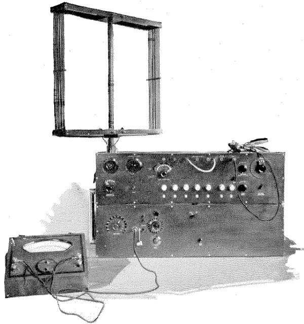
Fig. 3—Portable Field Strength Measuring Set for the Broadcasting Range
