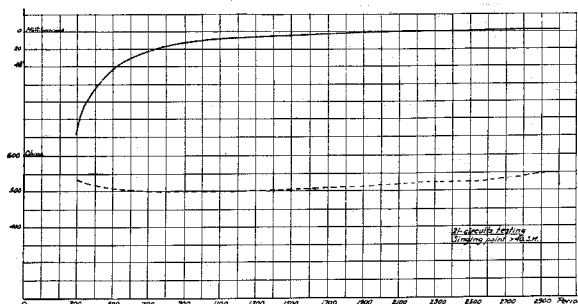
Figure 5—Stockholm-Norrköping Cable—Impedance curve in repeater section I, from Västerlång to Stockholm. Extra light loaded 0.9 mm. phantom circuit (pairs 401/402)
