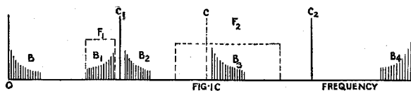
Figure 1—Spectra of Speech Bands
