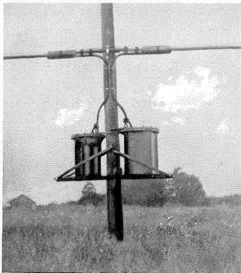
Figure 13—Installation of Aerial Toll Cable Loading—Single Pole Fixture for Small Branch Cables
