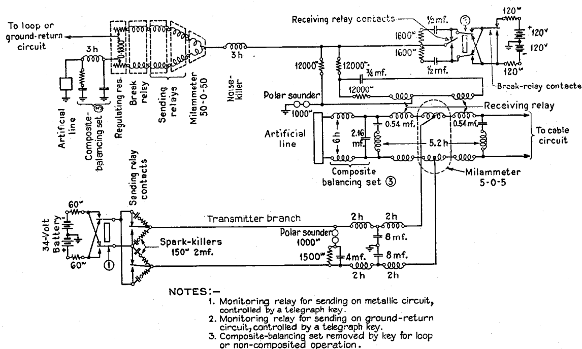
Figure 13—Terminal Repeater
