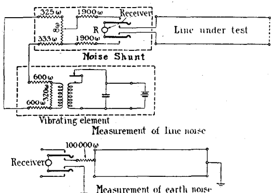
Figure 1—Noise Measuring Set—Circuit
