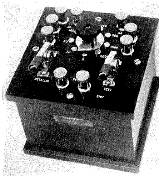
Figure 3—Noise Shunt
