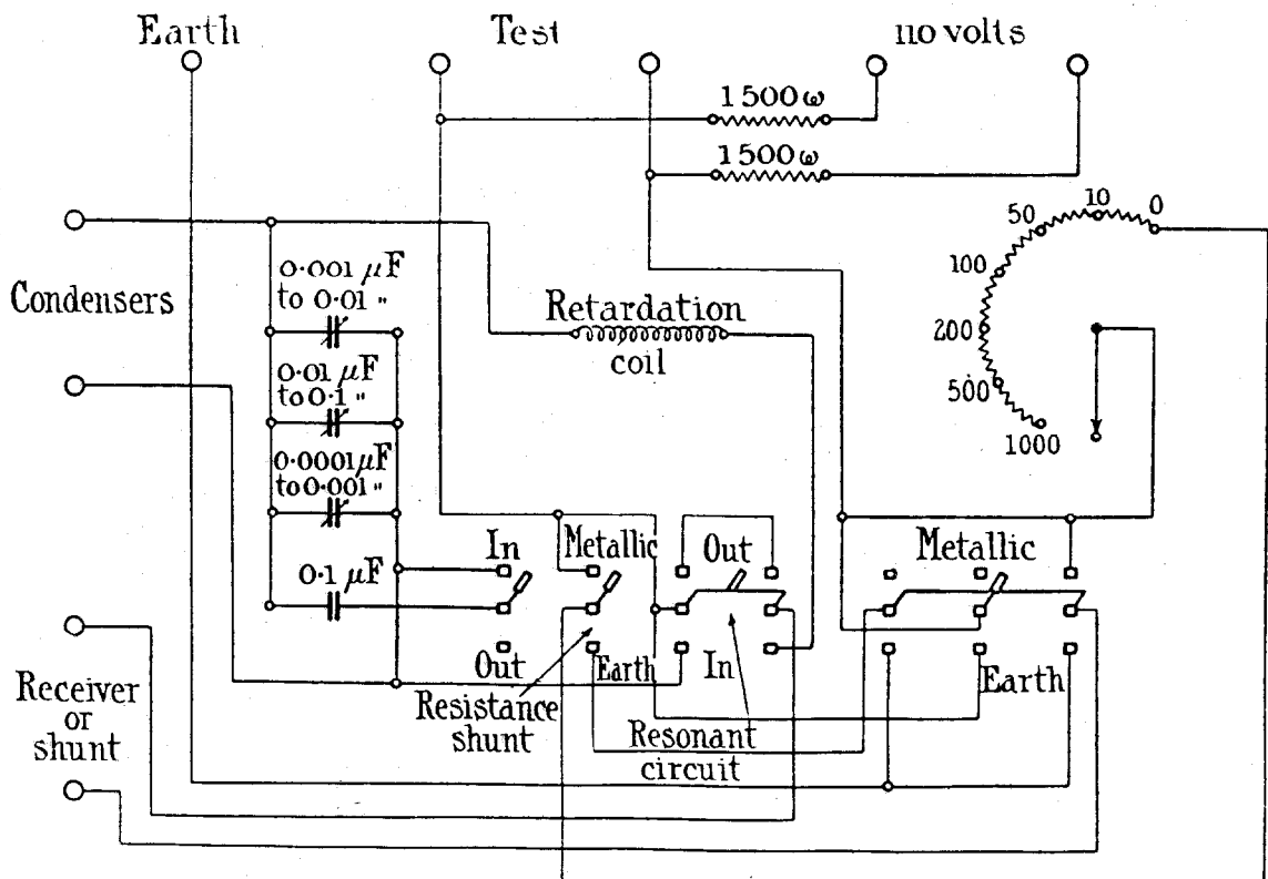
Figure 5—Noise Analyzer—Circuit
