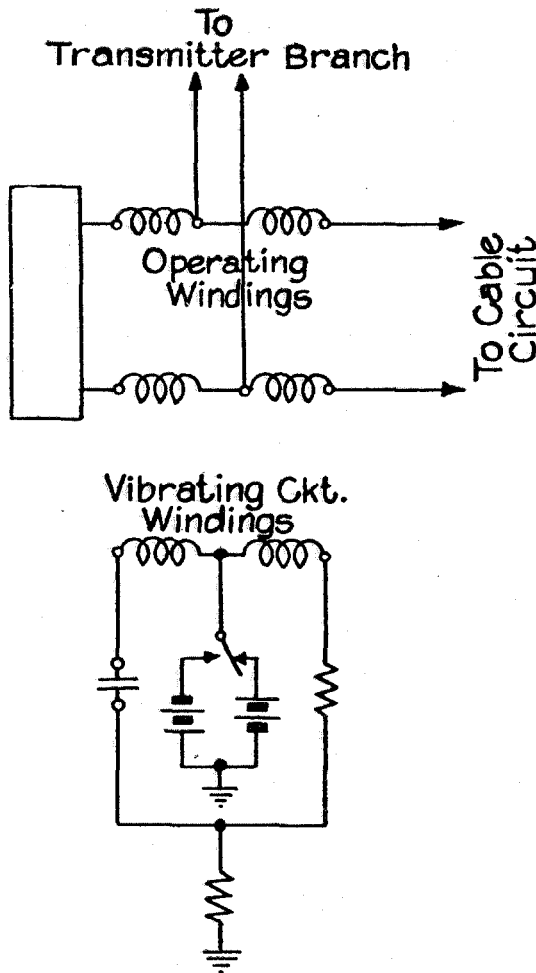
Figure 9—Vibrating Circuit
