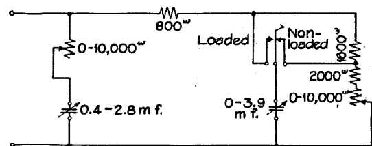
Figure 6—Duplex Artificial Line
