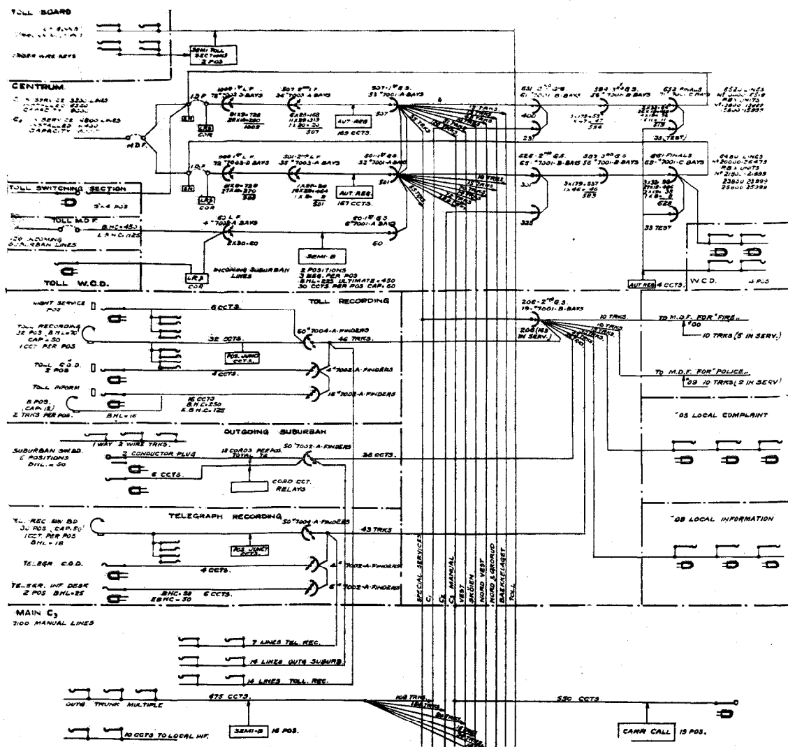
Figure 1—Junction Diagram—Kristiania Area
