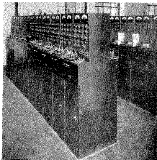
Figure 16—Installation of Metallic Telegraph Repeaters—Terminal Type
