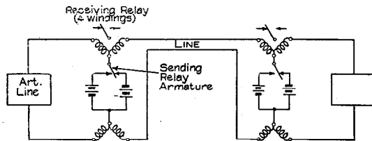
Figure 3—Symmetrical Differential Duplex on Metallic Circuit
