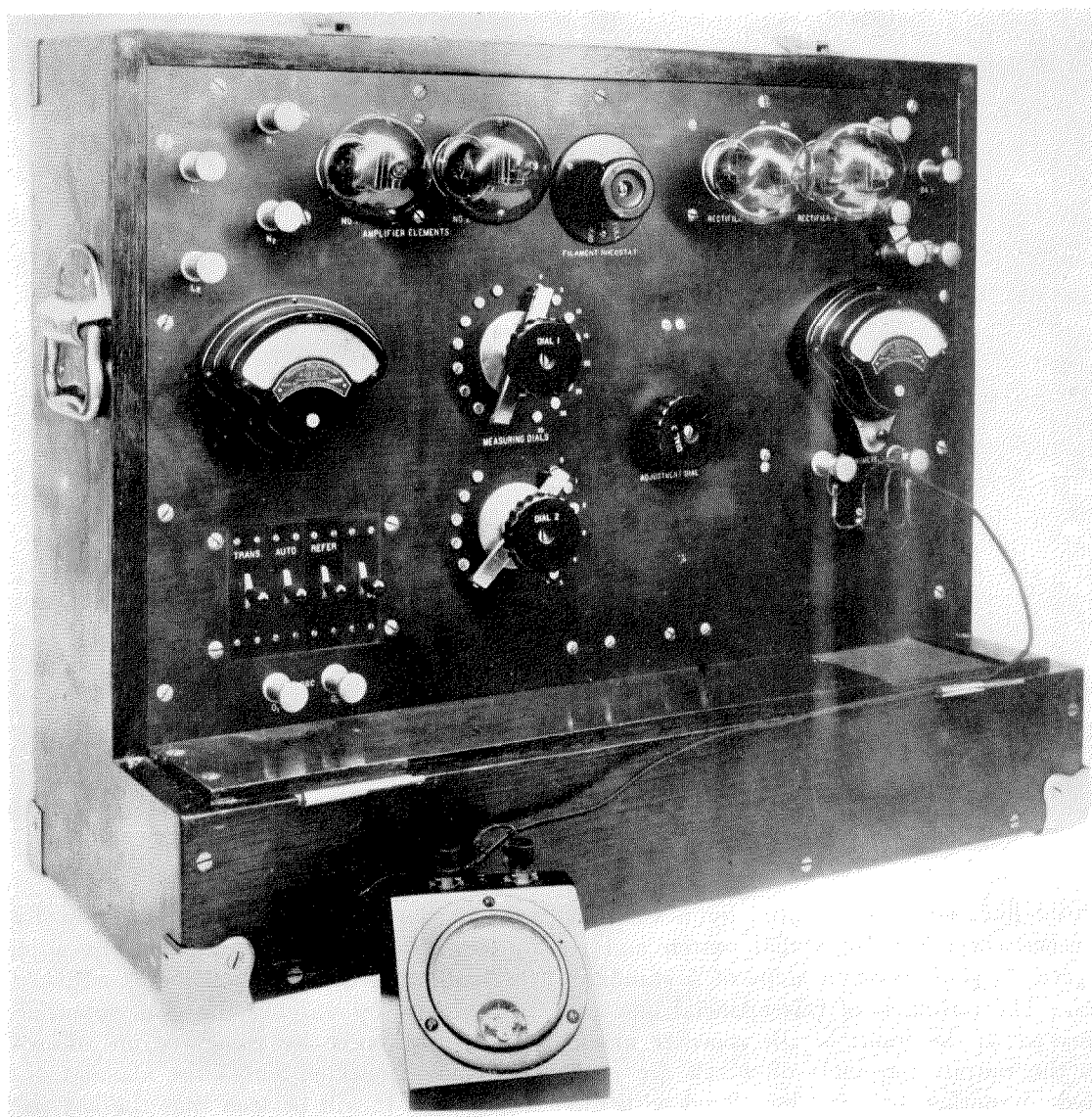
Figure 14—Impedance Irregularity Measuring Set
