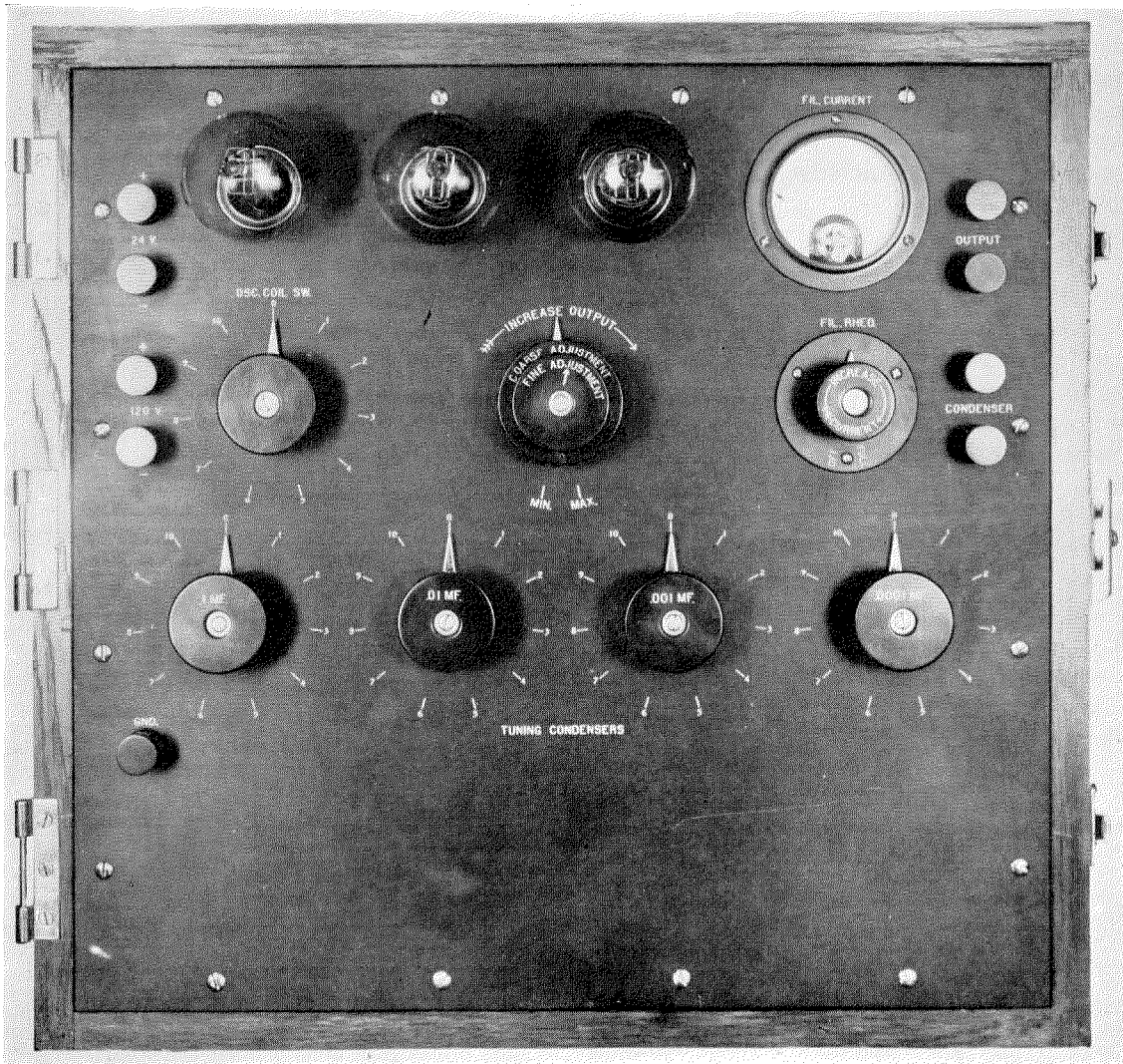
Figure 20—100-5,000 Cycle Oscillator
