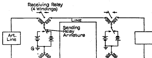
Figure 4—Metallic Duplex Circuit—Single Commutation
