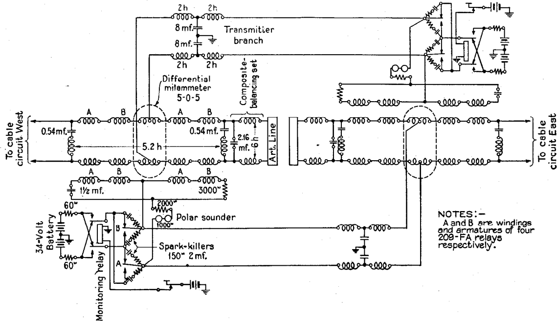
Figure 10—Through Repeater
