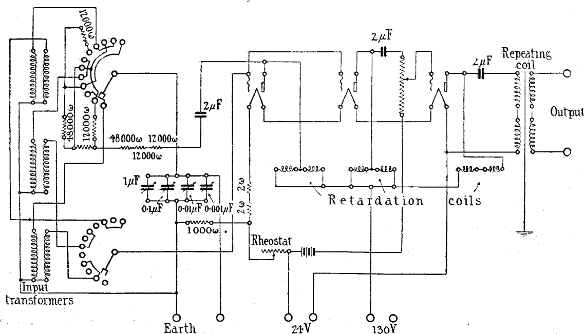
Figure 19—100-5,000 Cycle Oscillator—Circuit
