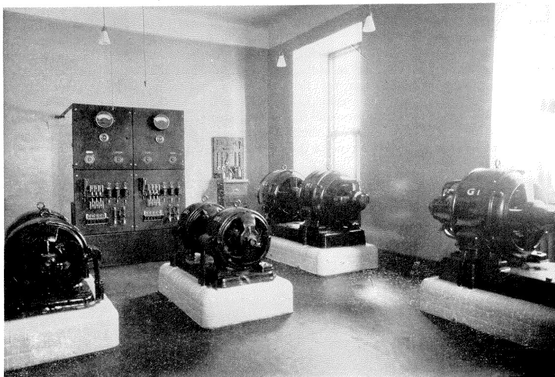
Figure 12—Power Room
