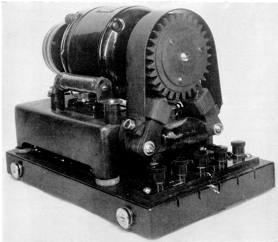
Figure 17—1,000 Cycle Oscillator
