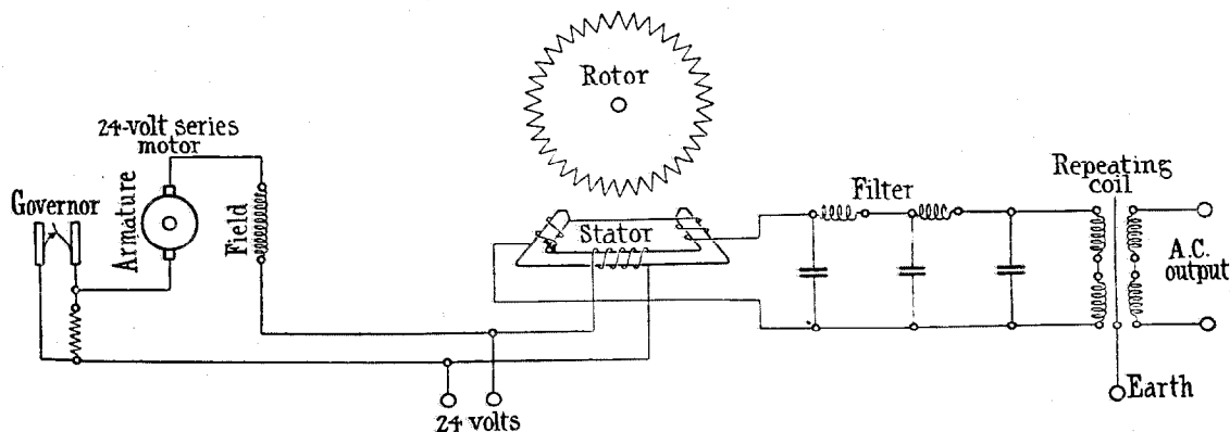
Figure 18—1,000 Cycle Oscillator—Circuit
