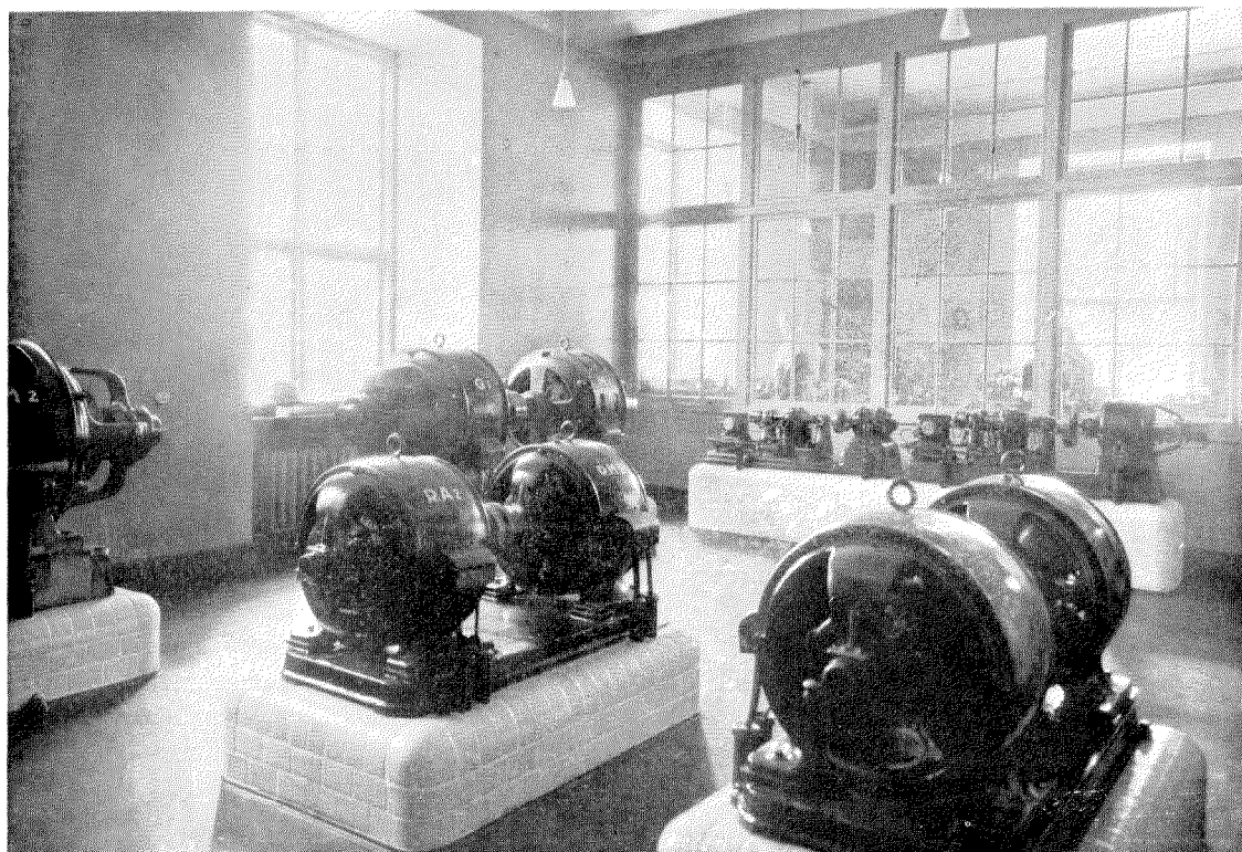
Figure 13—Power Room
