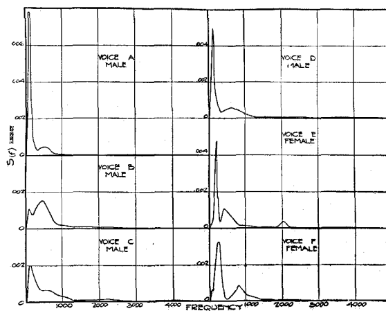
Fig. 5—Analysis of Individual Voices
