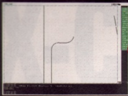
▲ FIGURE 9. The inner edge of the crankcase needed a bit of filleting. A quick bit of filleting and you're away.
