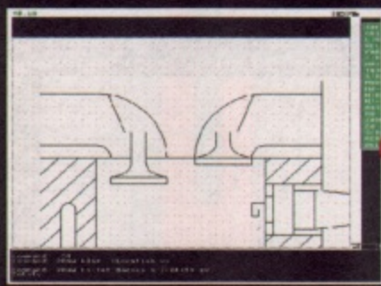
▲ FIGURE 21. The other side is drawn in. I chose to do this using MICOPY again and then modified it slightly. Note the valves have been filleted.
