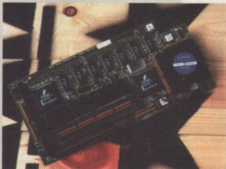
▲ GVP's G-Force Accelerator is a Zorro card for the A4000 and A3000. As a bonus feature, you get a built-in SCSI connector, allowing additional SCSI devices to be used with your Amiga.
