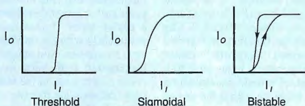
Figure 2: These functions represent the type easily implemented on optical processors, where I_i is the input signal intensity and I_o is the output signal intensity.
