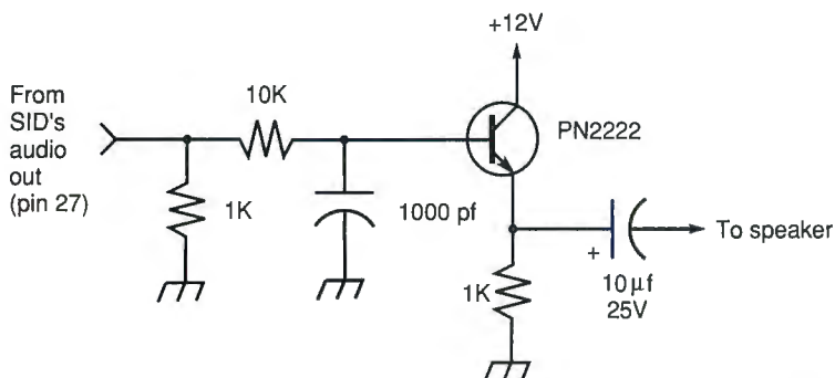
An audio amplifier circuit for the 6581 sound interface device (SID).
