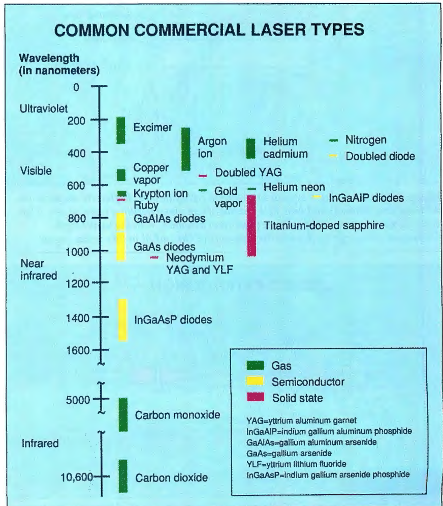
Figure 1: The three types of lasers shown here—gas, solid-state, and semiconductor—are all capable of generating visible light. (See table A.)
