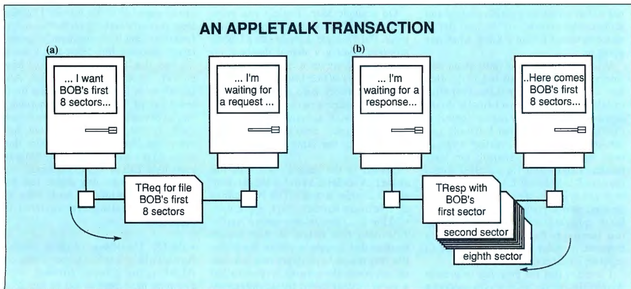
Figure 1: The anatomy of a transaction. (a) The system on the left sends a request (TReq) to the system on the right. The request is for the first eight sectors of a file. (b) Since a single request can be answered with up to eight responses, the system on the right is able to satisfy the request with eight response (TResp) packets.
