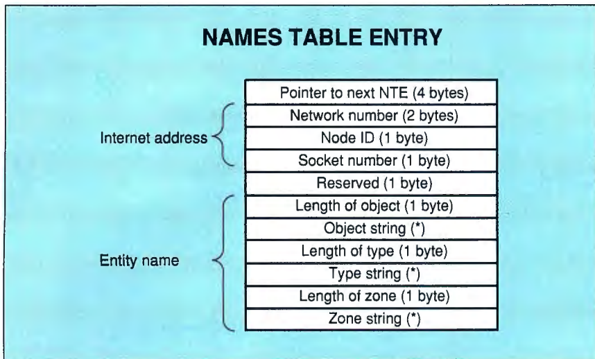
Figure 3: The names table entry (NTE) list is the Name Binding Protocol's in-memory notebook of what names are currently active on the network. Each NTE is composed of two parts, the entity's internet address and name. (Fields with asterisks are variable-length, with size determined by a preceding count byte.)
