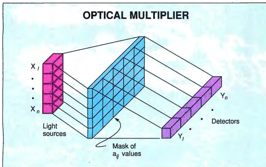
Figure 3: This analog optical multiplier evaluates the expression y = Ax .
