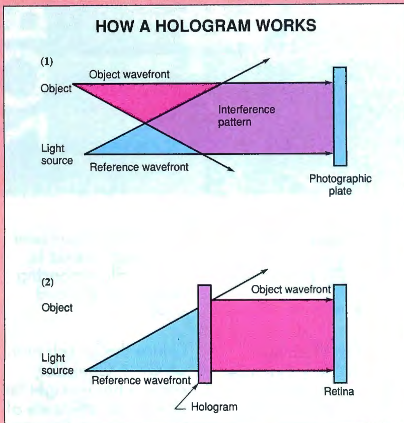
Figure B: (1) The interference between the reference wavefront and the object wavefront creates the hologram. (2) The hologram reconstructs the object wavefront from the reference wavefront.
