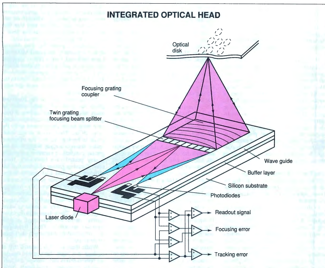
Figure 4: Developed at Osaka University, this device is substantially less massive than conventional optical heads. Work continues to improve its resolution. (Figure courtesy of Paul Y. Hu)
