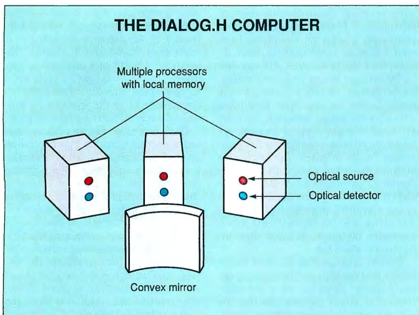
Figure 1: The Dialog.H computer is one of the earliest examples of using photonic interconnections within a computer. It consists of a multitude of electronic processors, each with its own local memory.
