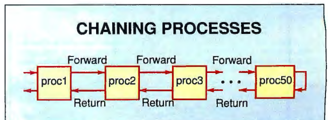
Figure 3: A simplified diagram of ray tracing using 50 parallel T80 transputers.
