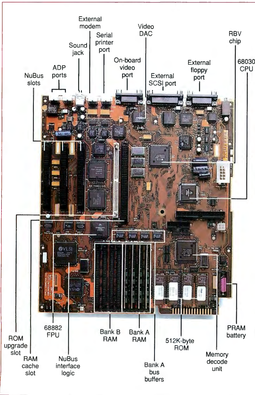
Photo 4: The Mac IIci motherboard. The various application-specific ICs reduce the board's component count and thus improve its reliability.
