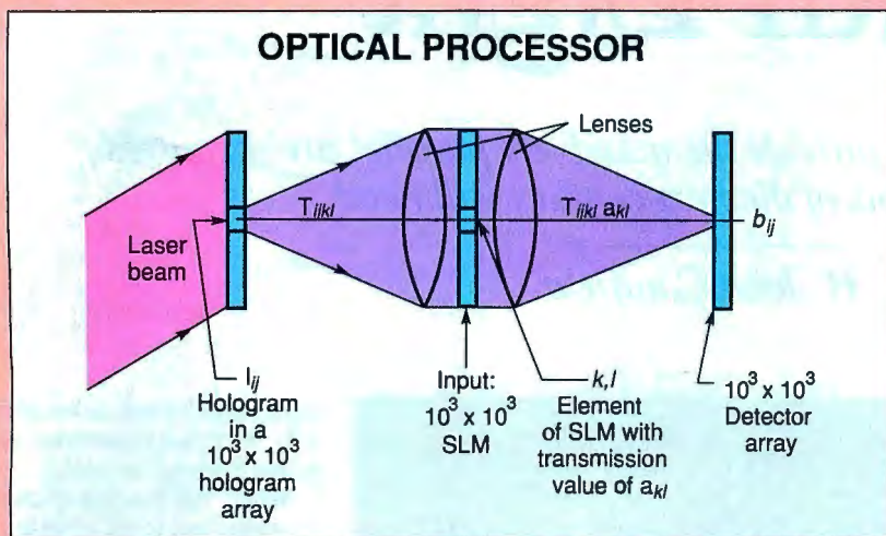
Figure A: Shown are the interconnections for one of the 1 million b_{ij} patterns.
