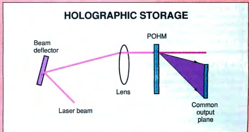
Figure C: Retrieving information from page-oriented holographic memory (POHM) involves deflecting the output of the read beam onto an output plane.
