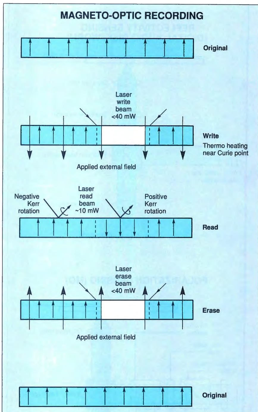
Figure 2: In synchrony with an external magnet, the strong write pulse fixes the magnetic orientation of a spot on the recording layer. The local magnetization imparts a positive or negative Kerr rotation to the reflection of the weak read beam. The magneto-optic head detects this rotation. (Figure courtesy of Paul Y. Hu)
