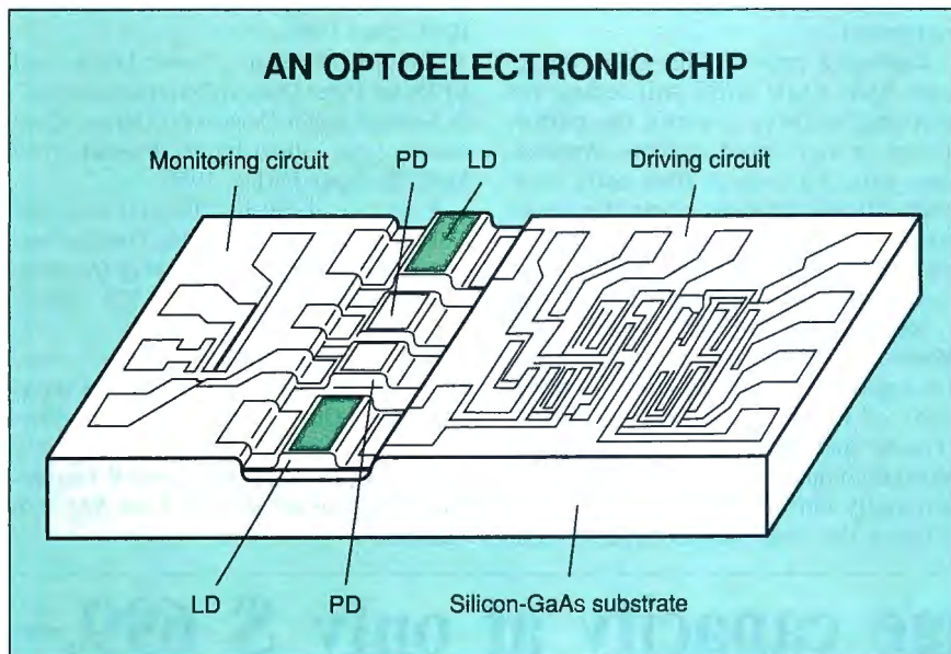
Figure 2: An example of the type of optoelectronic chip now being developed. It shows a typical OEIC structure containing laser diodes (LDs), photodetectors (PDs), and driving and monitoring circuits.
