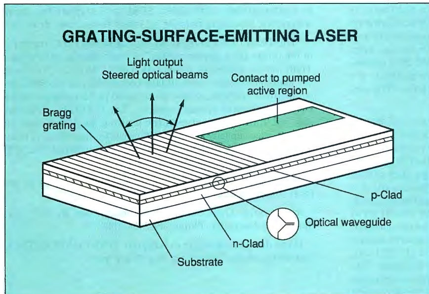
Figure 3: Grating-surface-emitting (GSE) laser structure. Light output is in the form of steered, focused, narrow optical beams from the surface of the diffraction grating. Current from the contact to pumped active region stimulates optical emission in the optical waveguide.
