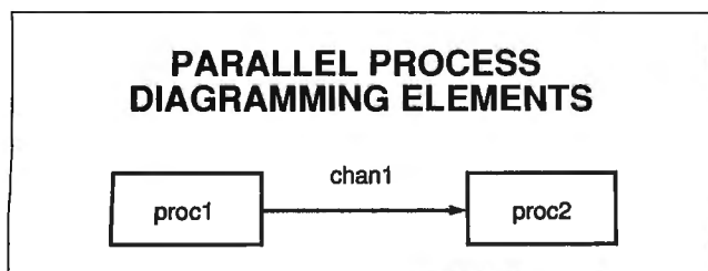
Figure 1: A process diagram of the simple program structure where proc1 communicates to proc2 through chan1 .
