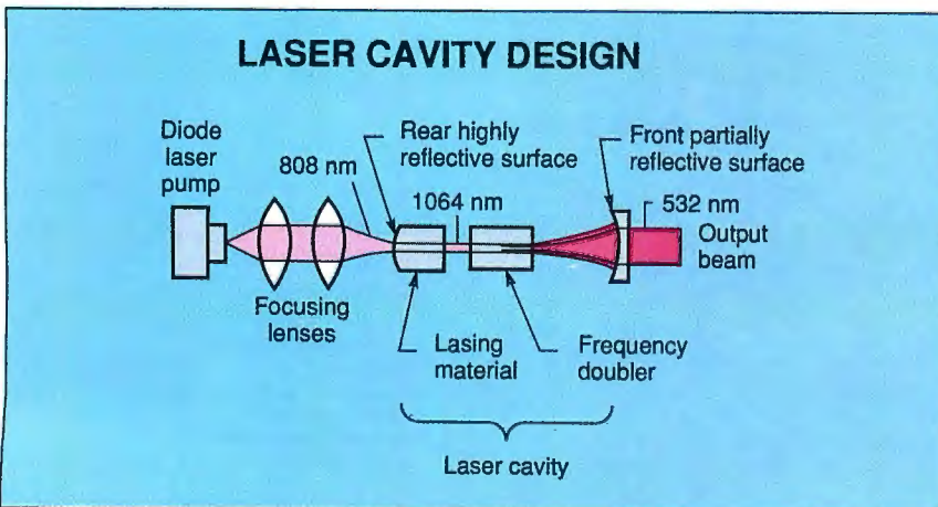
Figure 3: A CAD-generated, diode-pumped, frequency-doubled laser cavity. It illustrates the conversion of low-quality infrared diode-laser-pump light to high-quality infrared (1064 nm) and visible (532 nm) light in an all-solid-state design.
