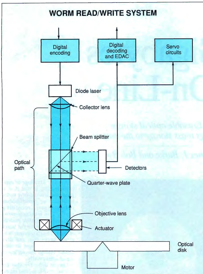
Figure 1: A strong laser pulse writes by creating a pit (or a bubble) at the recording layer. The reflectivity of the weaker read beam is analyzed to detect the presence or absence of pits. Compact-disk systems are very similar, except, of course, that they are read-only. (Figure courtesy of Paul Y. Hu)
