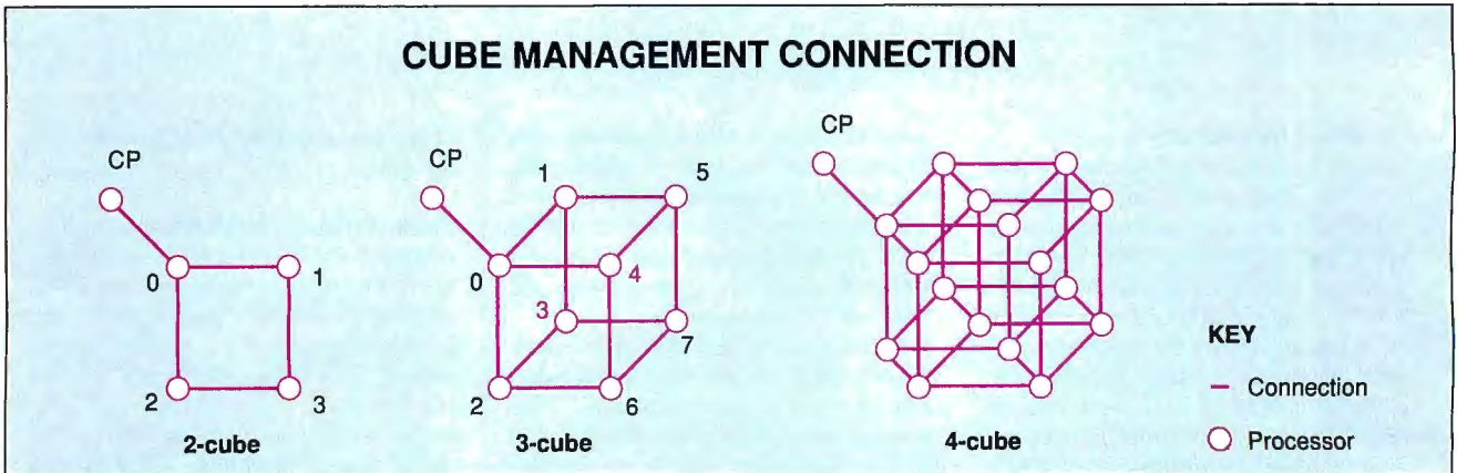
Figure 1: Hypercubes of dimensions 2, 3, and 4. Each cube has 2^p processing nodes and a single control processor, and each node is connected to p other processors. Thus, a 2-cube has four processing nodes and one control processor, and each processing node is connected to two other nodes.
