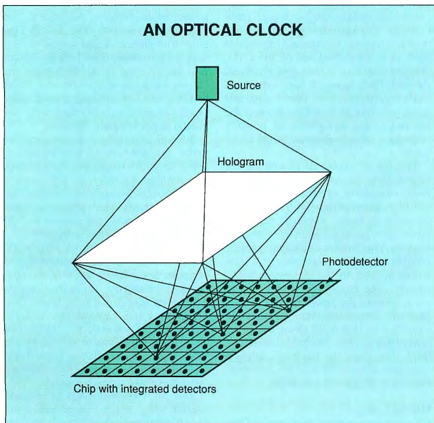
Figure 2: Optical clock distribution to a chip via a holographic optical element. An off-chip semiconductor laser source generates an optical timing signal, which a holographic optical element then efficiently broadcasts to many photodetectors embedded in the chip.
