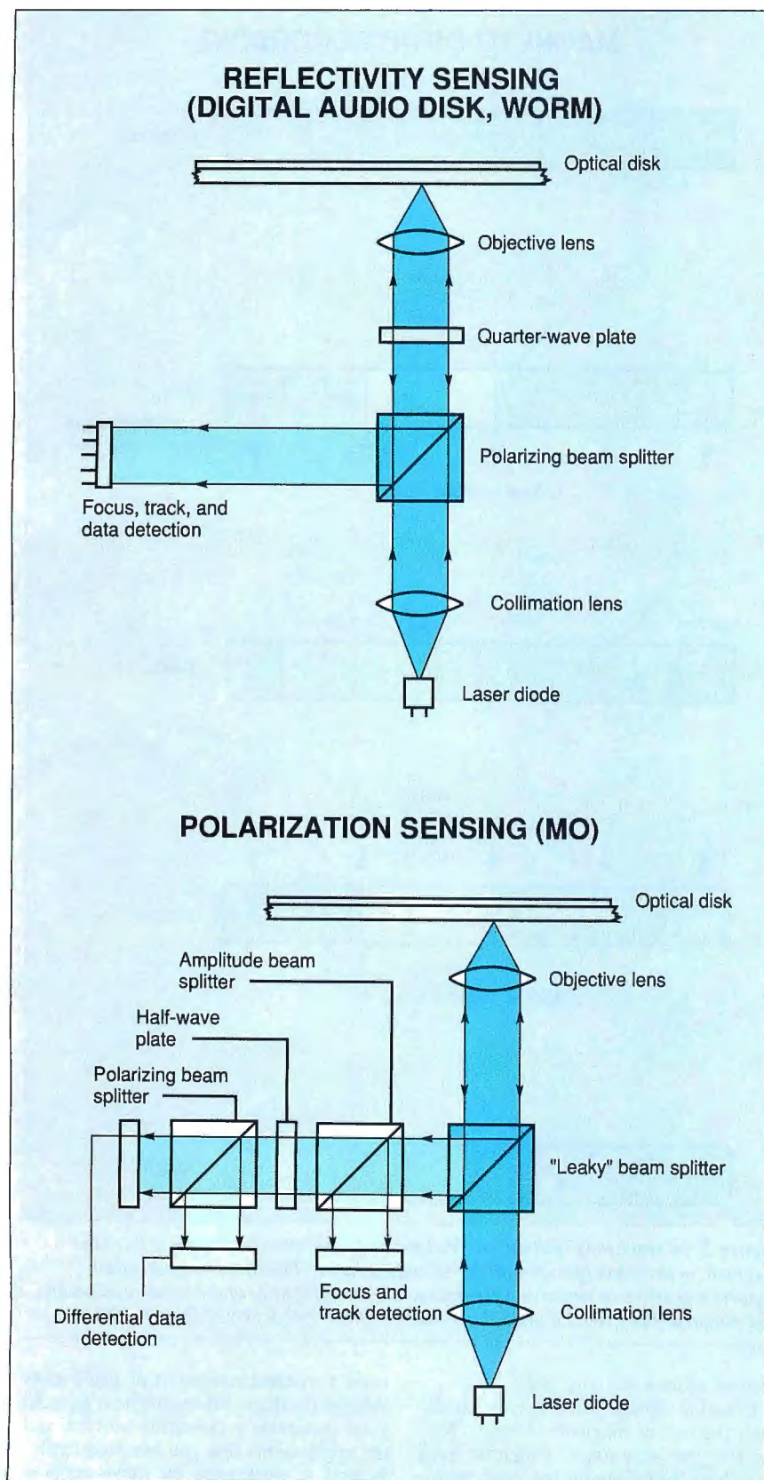
Figure 3: The size and complexity of magneto-optic heads result in their relatively slow access times. (Figure courtesy of Paul Y. Hu)
