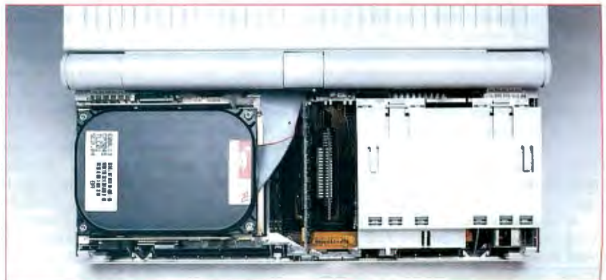
Photo 3: Inside the Portable. At left is an optional 40-megabyte SCSI hard disk drive; in the center are RAM/ROM expansion slots; to the right is the battery housing.
