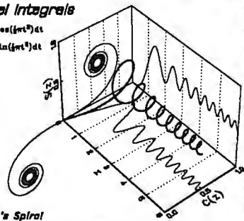
Cornu's Spiral
