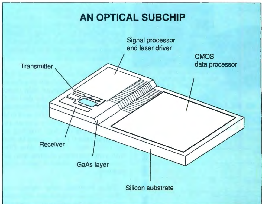
Figure 1: An optical interconnect subchip. Note that it is fabricated on GaAs, a substance with properties different from those of the silicon substrate but capable of being grown directly on it. The OEIC computer chip itself is fabricated of silicon.
