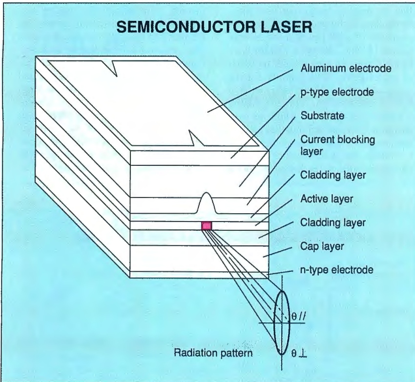
Figure 2: Illustration of a typical laser-diode cavity design. Reflective surfaces on the front face (shown) and rear face (hidden from view) define a laser cavity. The active layer is composed of gallium aluminum arsenide, with the wavelength determined primarily by the relative amounts of Ga and Al in this active region.
