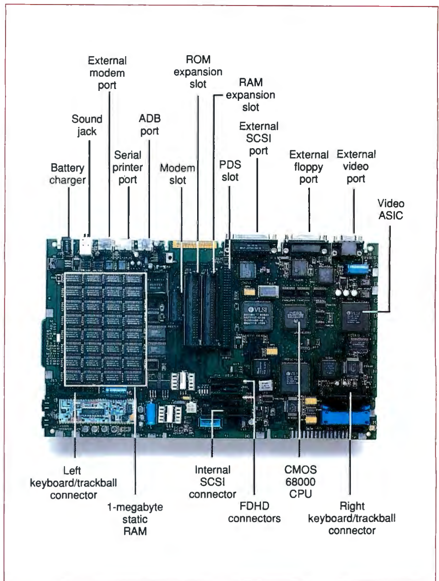
Photo 2: The Mac Portable motherboard. It uses CMOS components to reduce power consumption. The 68000 CPU runs at 15.67 MHz, twice the rate of a Mac SE.
