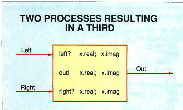
Figure 2: A process diagram of two input streams multiplexed into a single output stream. The Boolean value FALSE on channel shutoff will terminate the program.
