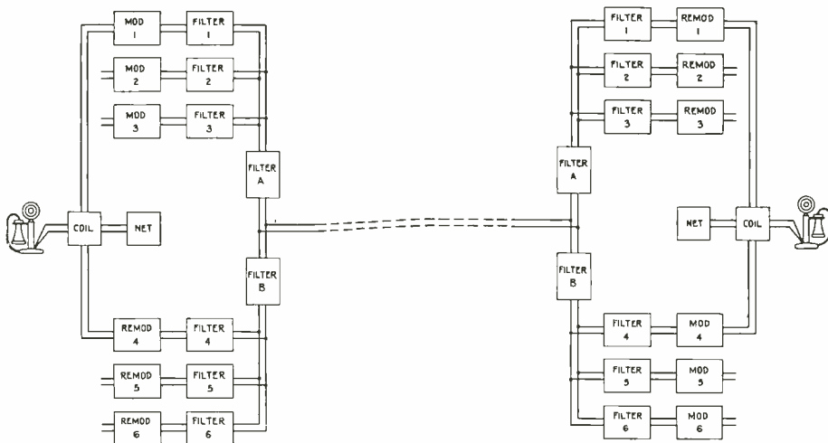
Fig. 3: Arrangement of filters and modulating circuits for a three-channel carrier system, illustrating the "directional grouping" scheme
