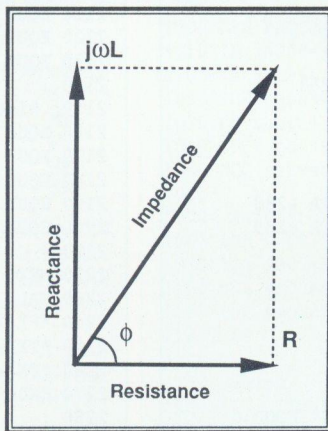
Figure 1. The construction of an impedance triangle
