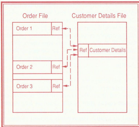
Figure 2. A Relational File Structure
