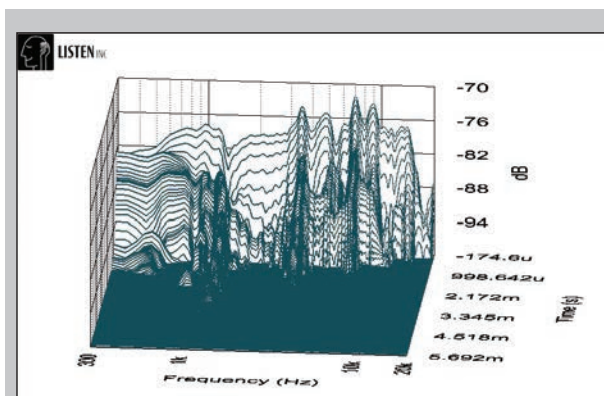
Figure 23: SB Acoustics MW16R SoundCheck CSD waterfall plot
