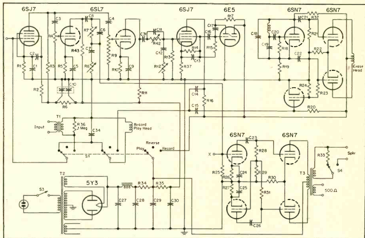
Fig. 1. Complete schematic of the modified Brush amplifier for use with the machine described.
