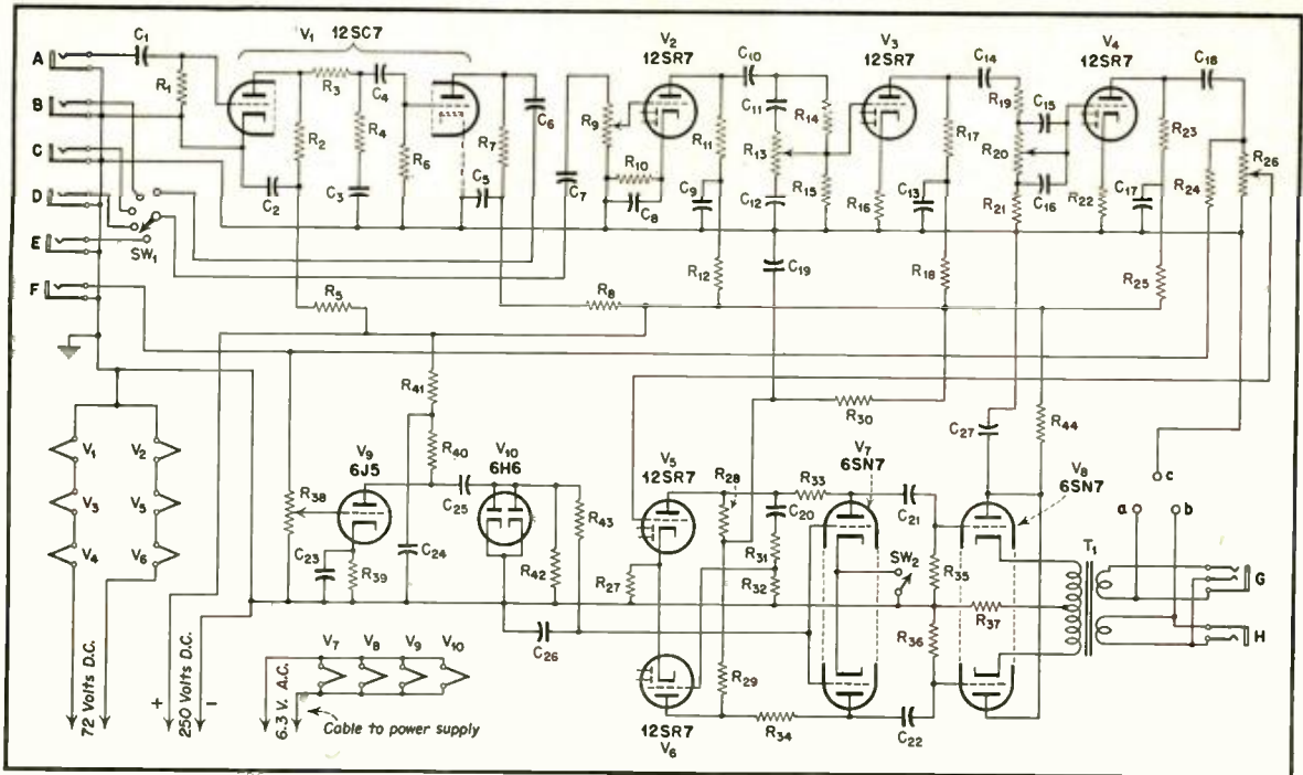
Fig. 1. Schematic of preamplifier unit. Note flexibility of control and provision for expansion if desired.
