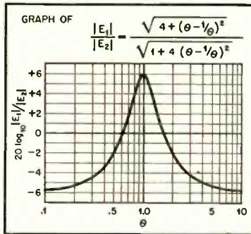
Fig. 3. Curve showing relative voltage at output #1 of Fig. 2. This curve also applies to output #2 if signs are interchanged.
