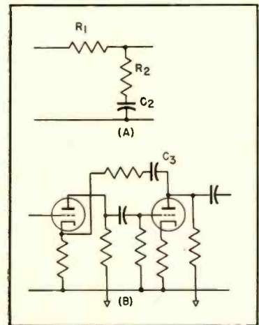
Fig. 3. (A) Losser circuit to provide low-frequency boost. This circuit is usually placed between two high- \mu triode stages. (B) Feedback circuit commonly used in preamplifiers to provide required low-frequency boost.
