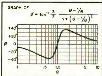
Fig. 4. Phase-shift curve for circuit of Fig. 2.
