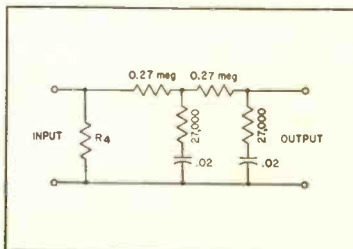
Fig. 4. Losser circuit suitable for use between magnetic pickup and high-gain, high-impedance input of P.A. system amplifier, such as normally used for crystal microphones.
