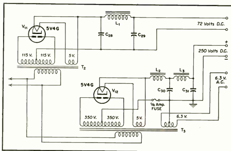
Fig. 2. Schematic of power supply used with preamplifier of Fig. 1.
