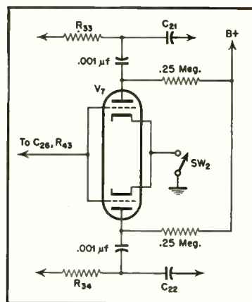
Fig. 3. Modification of V_7 circuit to make the expander function as a noise suppressor.
