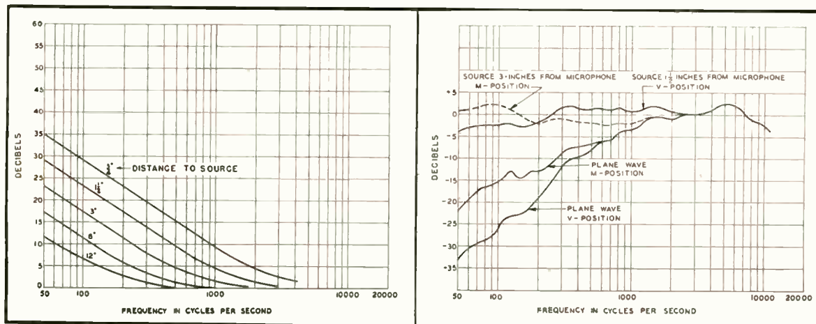
Fig. 6 (left). Curves showing increase in low-frequency response due to proximity of sound source. Fig. 7 (right). Response-frequency characteristics of KB-2C with special packing for plane wave and for close talking. Curves show how modification results in anti-noise characteristic.
