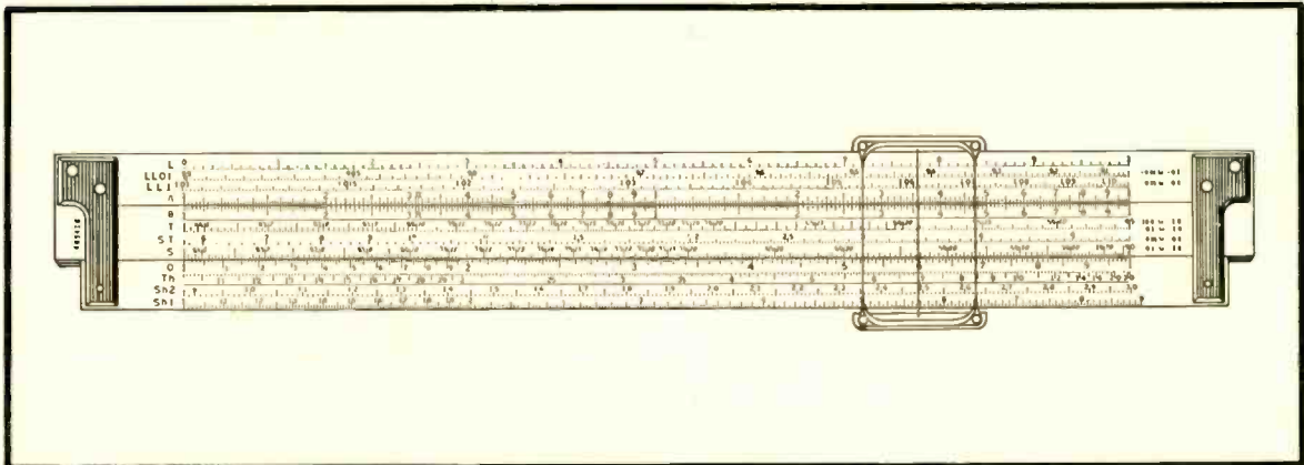
Fig. 2. The N4083 Slide Rule, showing the hyperbolic scales. Illustration shows one side of rule. Hyperbolic tangents are obtained by use of Th scale, while hyperbolic sines are given by use of scales Sh1 and Sh2 . (Copyright by Keuffel & Esser Co.)
