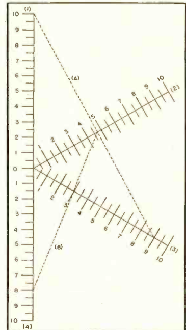
Fig. 7. Graphical solution for resistors in parallel; a handy device for attenuator design and general audio work.
