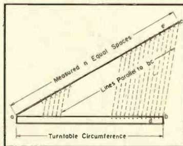
Fig. 2. Simple method commonly used for laying out a rim array for a phonograph turntable.
