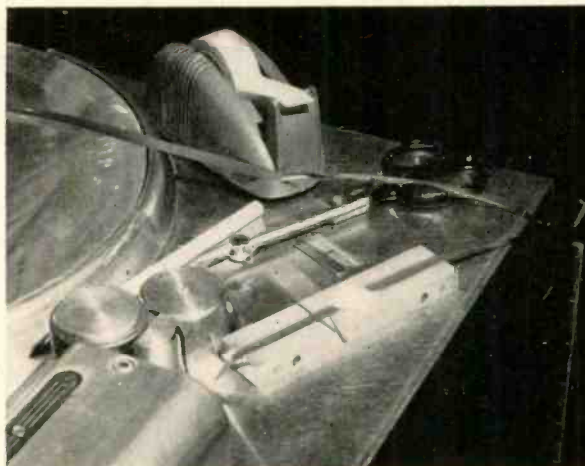
Fig. 5. Tape ends are joined together in the splicing block. The #41 Scotch tape is applied at an angle to the magnetic tape so there will be the least possible disturbance to smooth motion of the tape through the head assembly.
