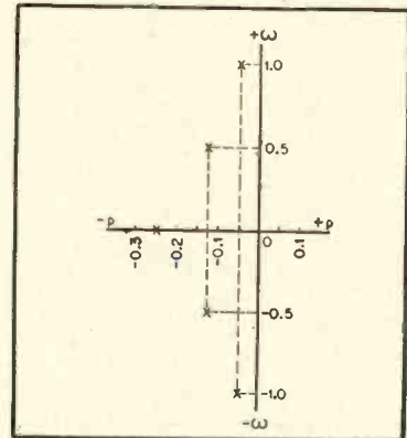
Fig. 2. Pole locations in complex frequency plane for a typical loudspeaker.
