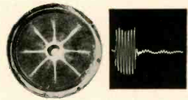
Fig. 10A (left). Cone breakup at 450 cps, with eight radial nodes; point B. Fig. 10B (right). Transient response to same signal.
